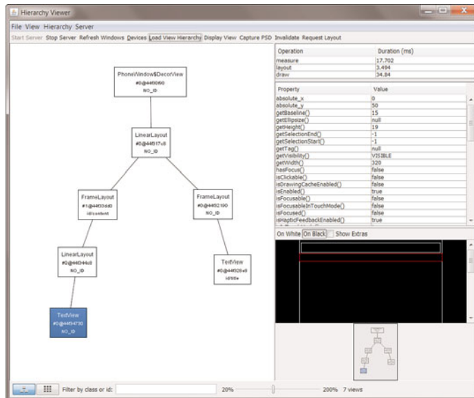
Figure 2.8 Screenshot of the Android Hierarchy Viewer in action.
