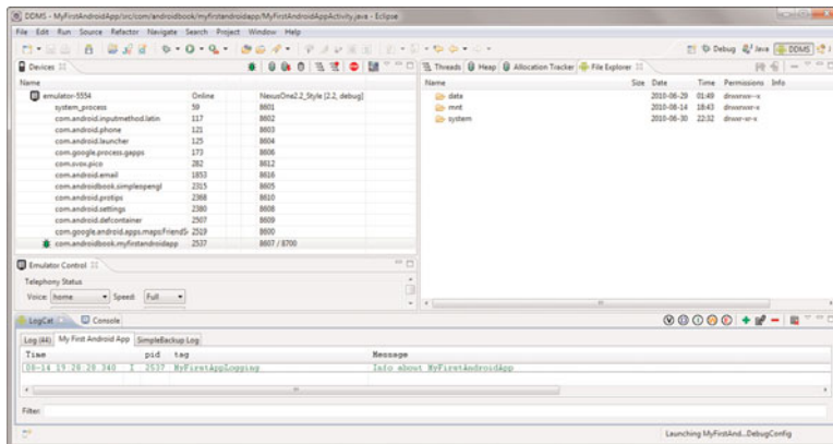
Figure B.5 Using a custom LogCat filter with DDMS.
