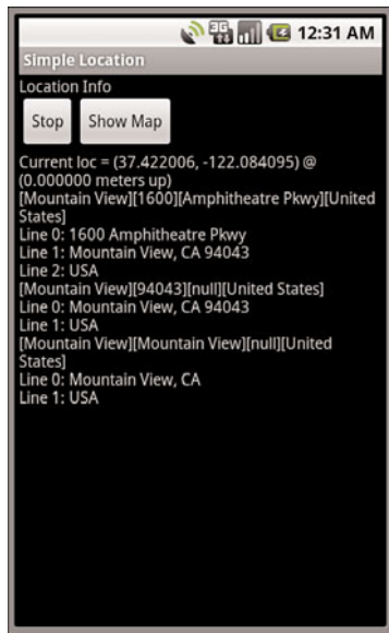
Figure 14.1 Image showing location geocoded to three “addresses.”
