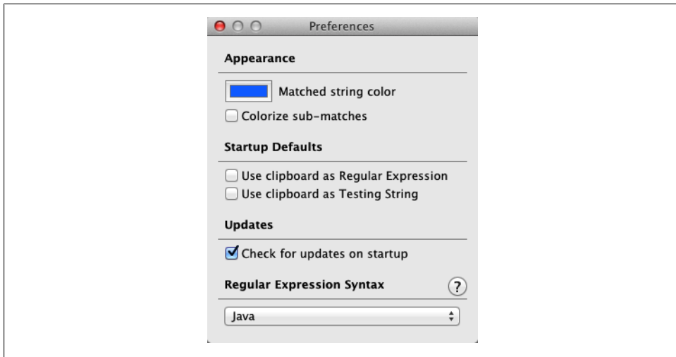
Figure 5-3. Reggy preferences
