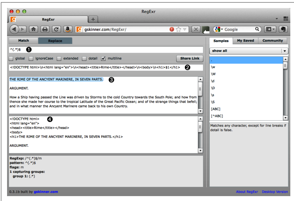
Figure 3-4. Adding markup with RegExr
