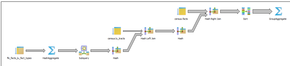
Figure 9-7. Graphical explain of using subqueries instead of CASE
