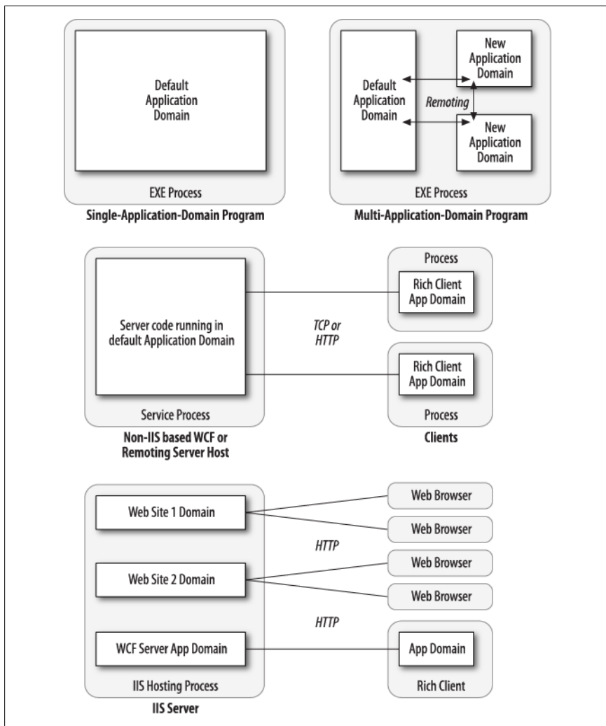
Figure 24-1. Application domain architecture
