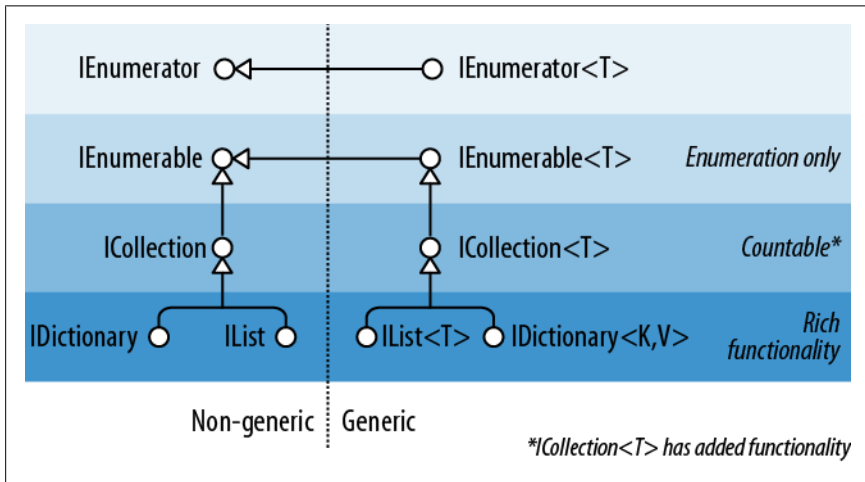
Figure 7-1. Collection interfaces
