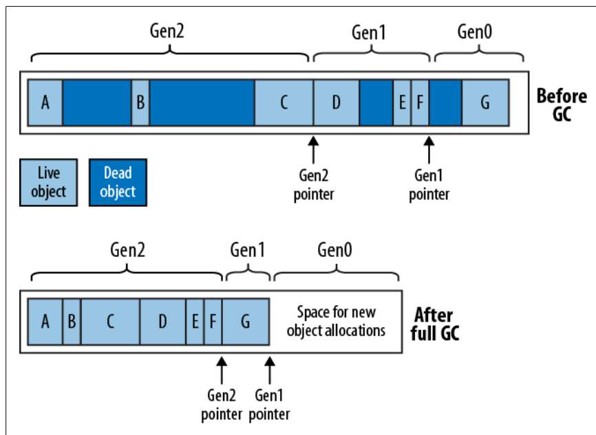
Figure 12-2. Heap generations
