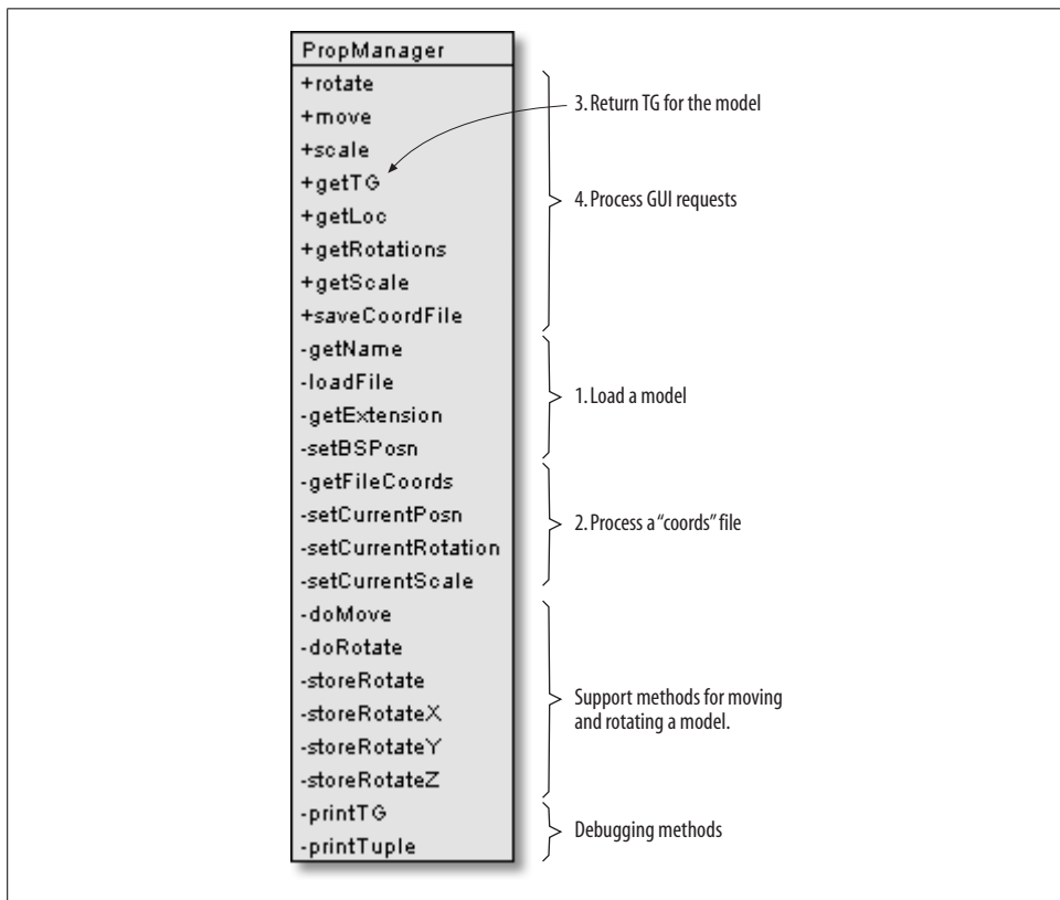
Figure 16-21. PropManager methods
