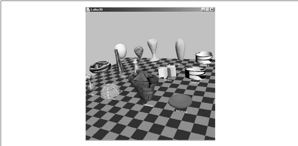
Figure 17-1. LatheShape3D objects
