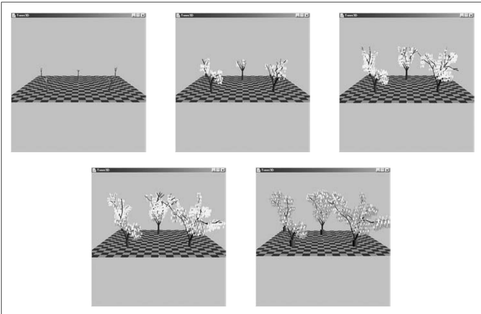
Figure 28-1. Growing trees
