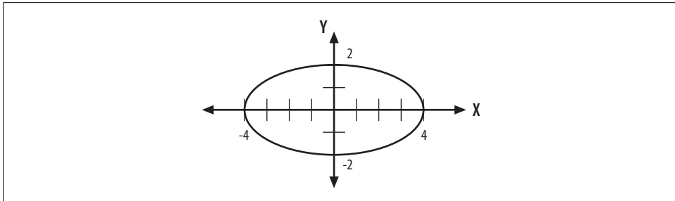
Figure 17-20. Another ellipse
