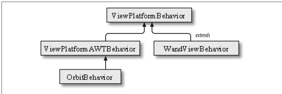
Figure 24-4. ViewPlatformBehavior and subclasses
