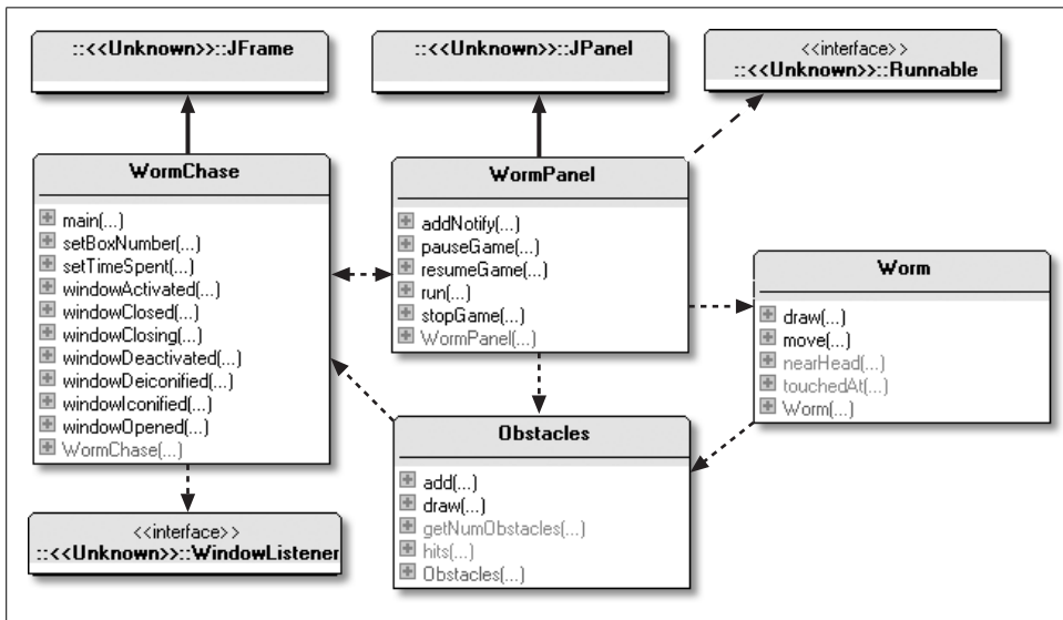
Figure 3-2. Class diagrams for the WormChase application
