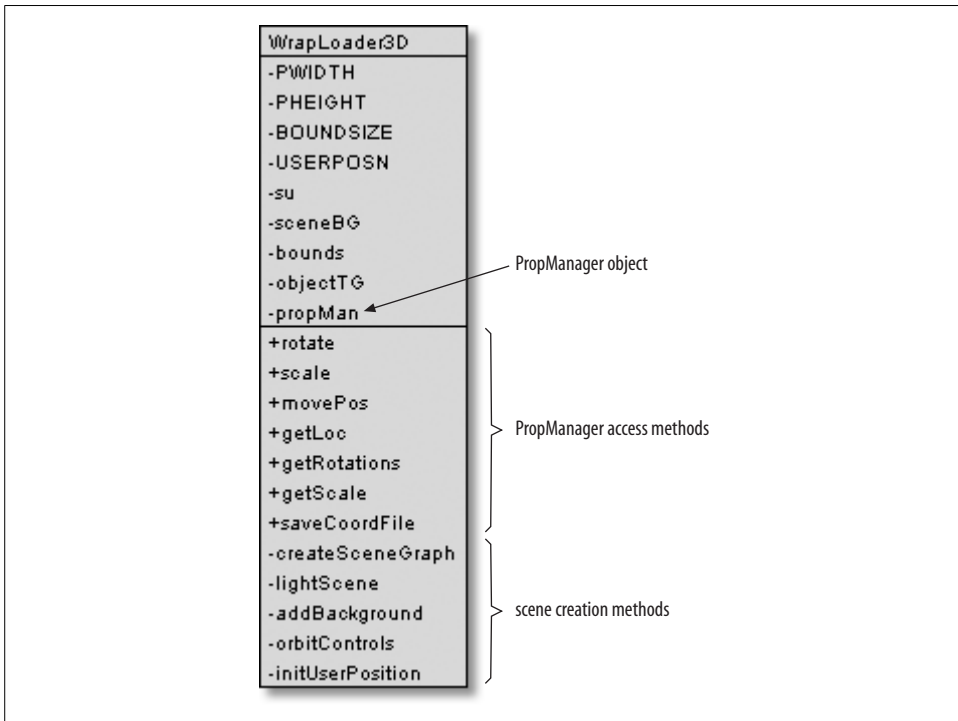
Figure 16-20. WrapLoader3D methods
