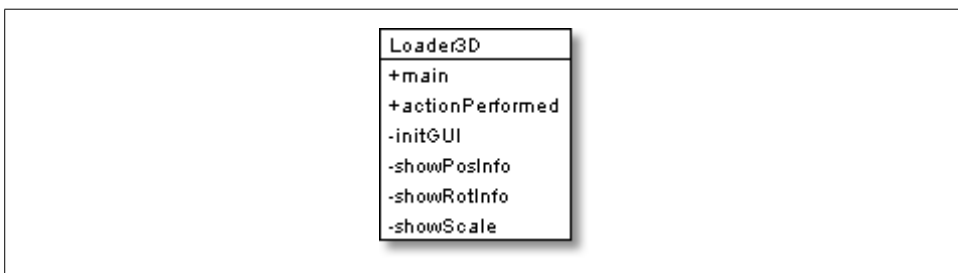
Figure 16-19. Loader3D methods
