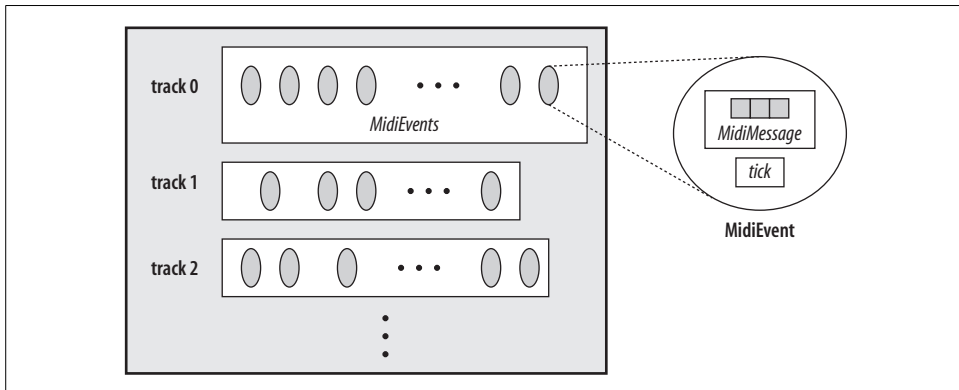
Figure 7-9. The internals of a MIDI sequence
