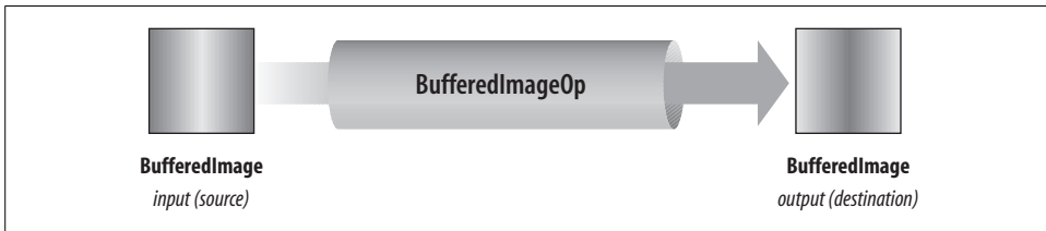
Figure 5-5. The BufferedImageOp imaging model
