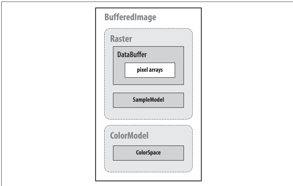
Figure 5-4. BufferedImage internals
