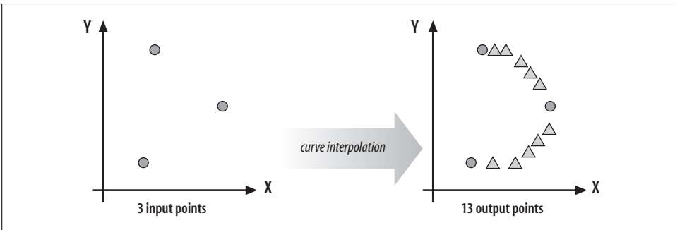
Figure 17-9. Interpolating curves
