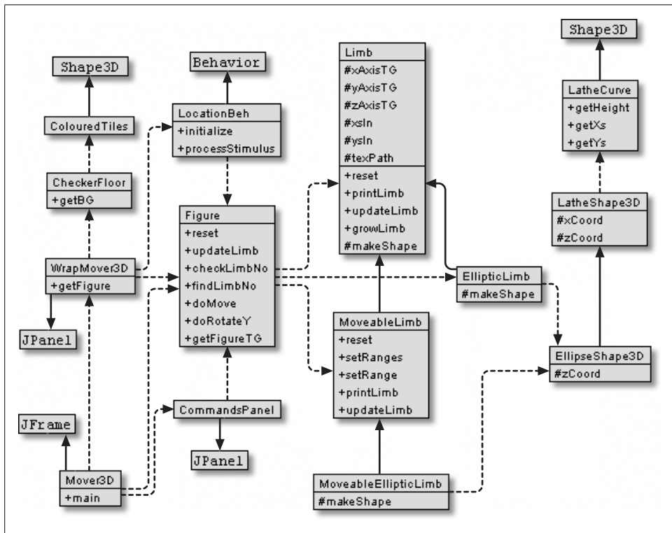
Figure 20-7. Class diagrams for Mover3D
