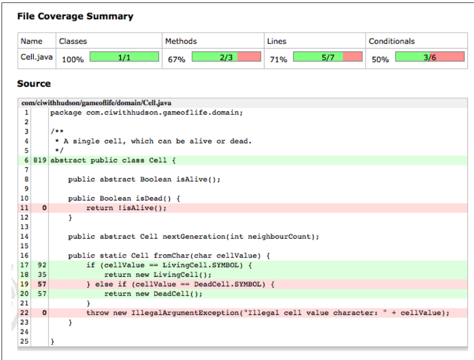
Figure 2-31. Jenkins lets you display code coverage metrics for packages and classes
