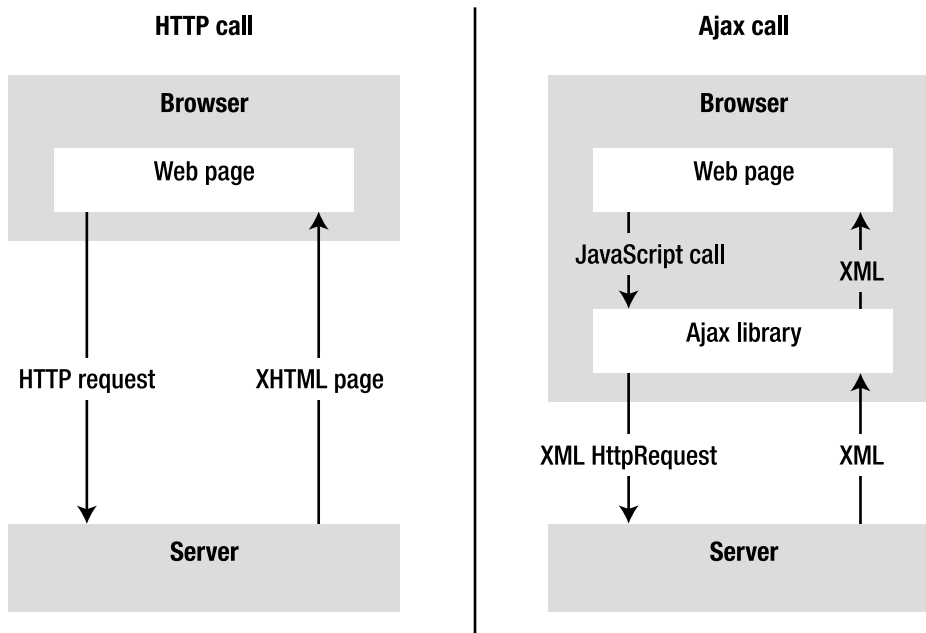
Figure 12-7. Plain HTTP calls vs. Ajax HTTP calls
