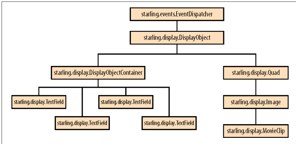
Figure 2. DisplayObject inheritance
