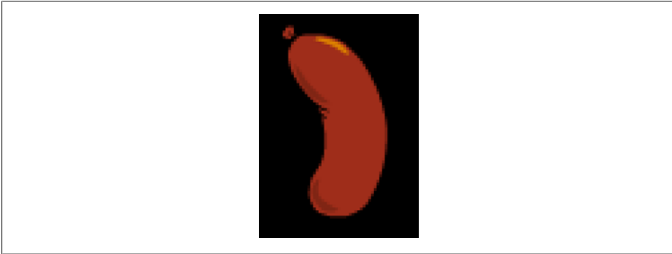
Figure 18. TextureSmoothing.NONE
