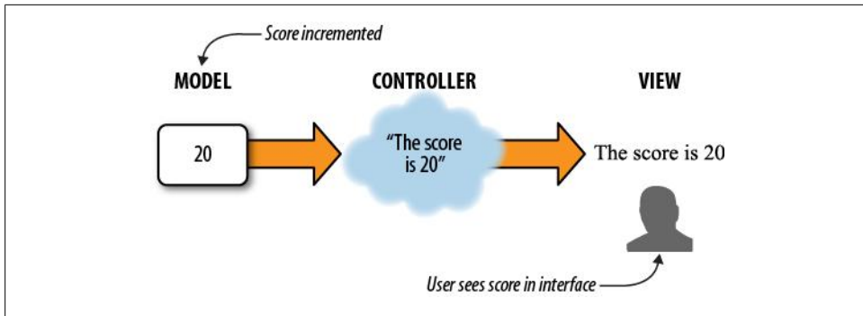
Figure 13-1. Model–view–controller
