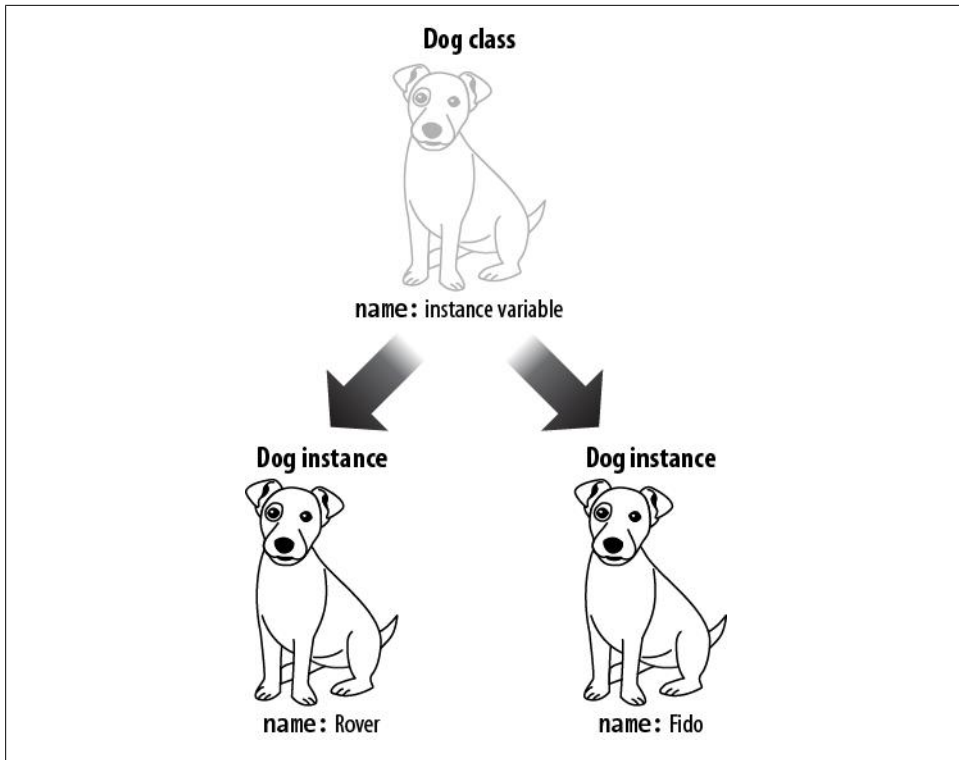
Figure 2-2. Instance variables
