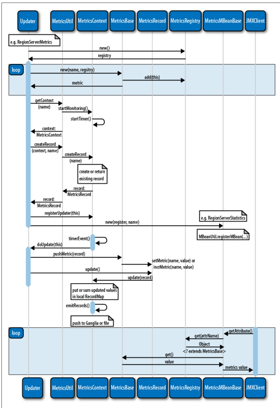
Figure 10-1. Sequence diagram of the classes involved in preparing the metrics
