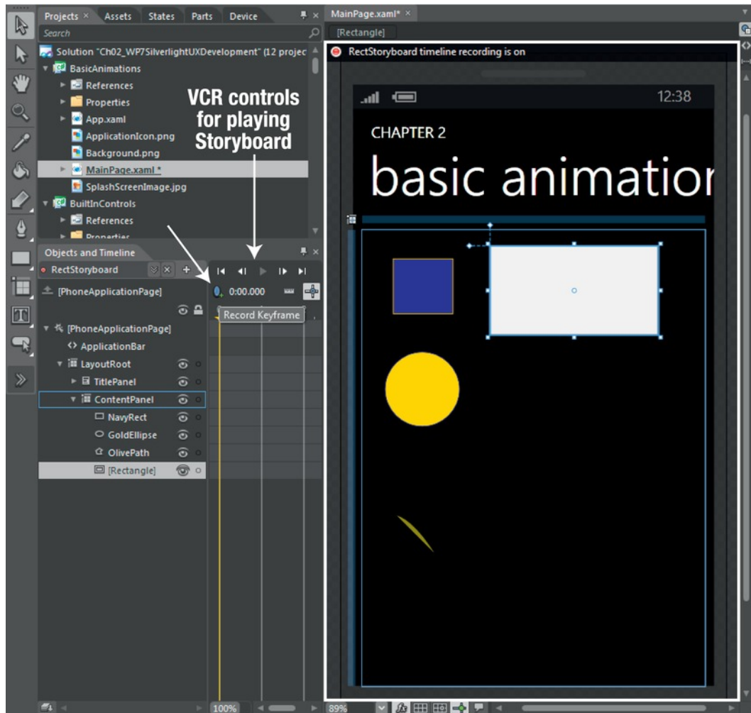
Figure 2–42. Storyboard editor
