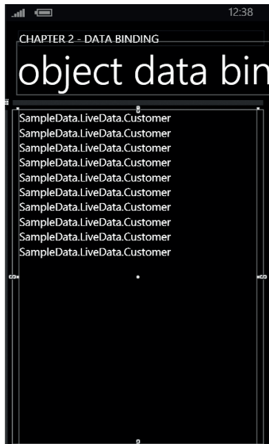
Figure 2–29. Data-bound ListBox
