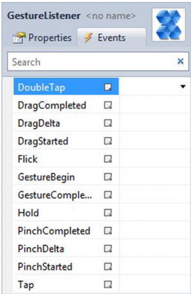
Figure 3–10. GestureListener events
