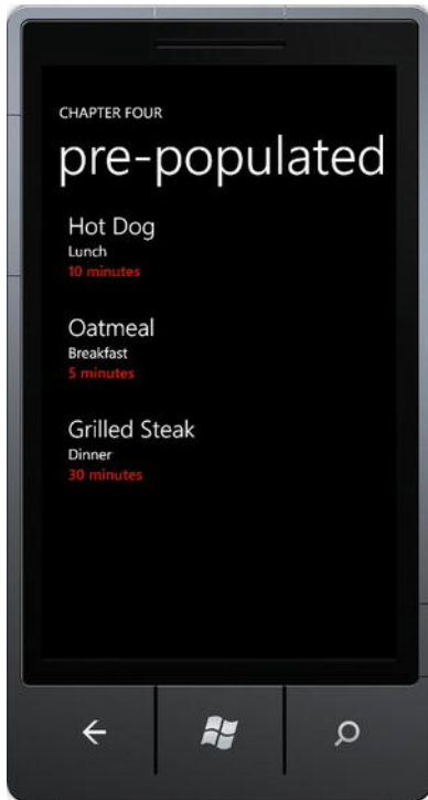
Figure 4-3. DBPrePropSample MainPage.Xaml
