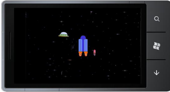
Figure 8-11. Animated sprites
