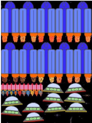
Figure 8-10. Generated textures
