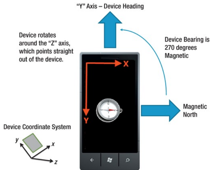
Figure 3-18. Compass functionality
