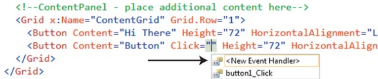
Figure 1-8. XAML IntelliSense
