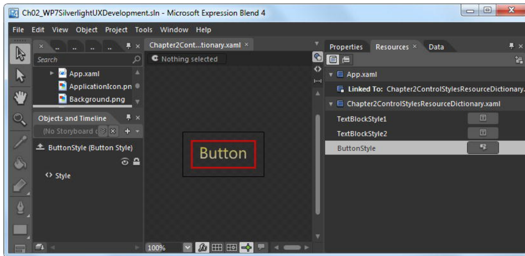
Figure 2–36. Resources window
