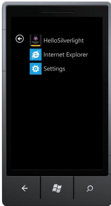
Figure 1–19. App list
