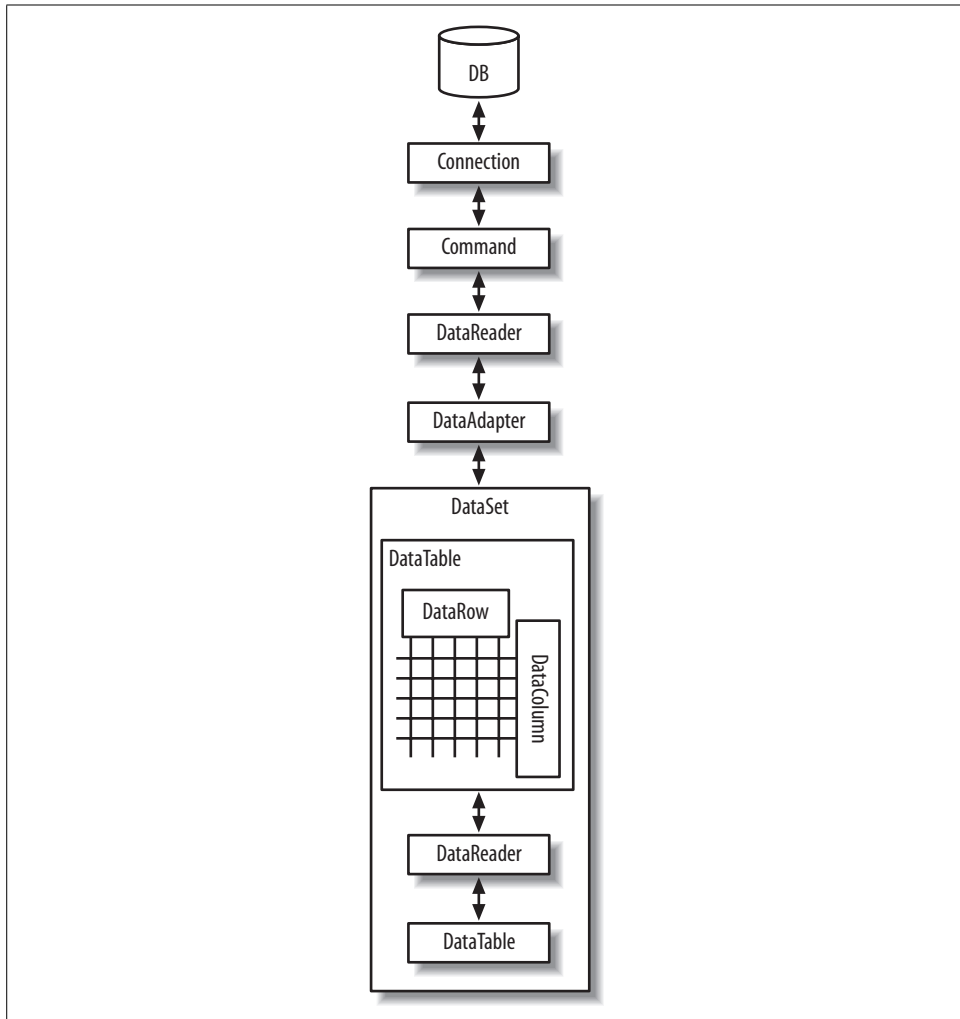
Figure 10-1. Providers and data sets in action
