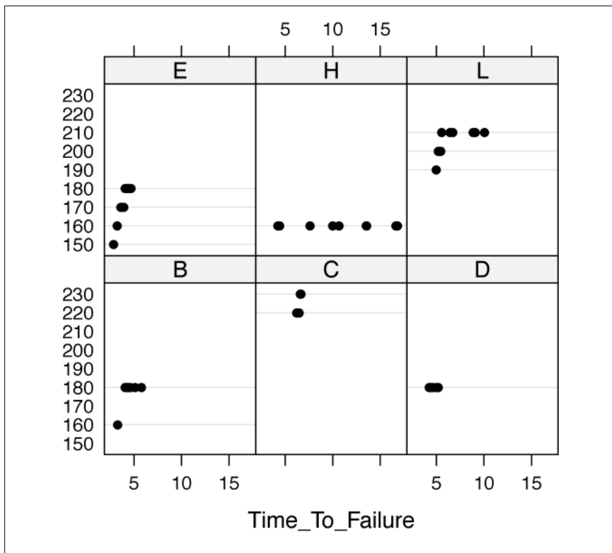
Figure 15-10. Time to failure and speed at failure for different types of tires
