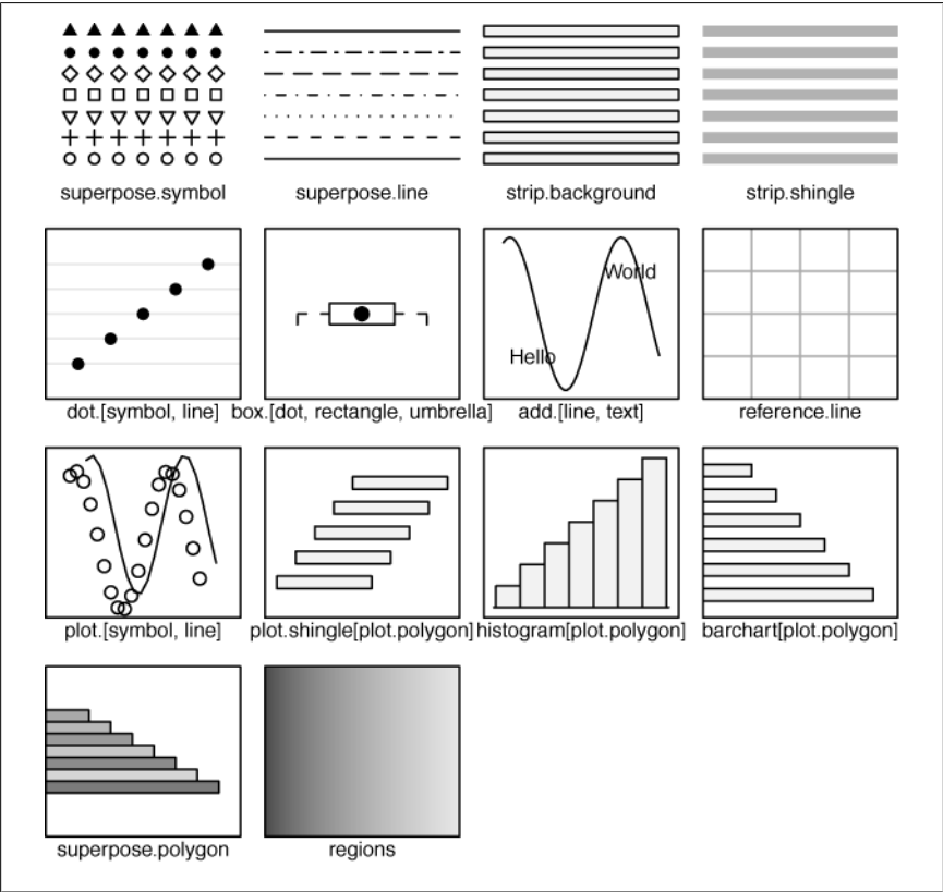
Figure 15-32. Example of show.settings
