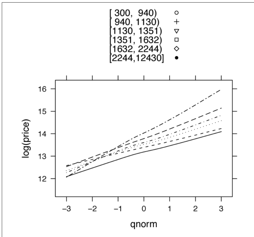
Figure 15-21. Quantile-quantile plots of logs of property prices for different numbers of square feet
