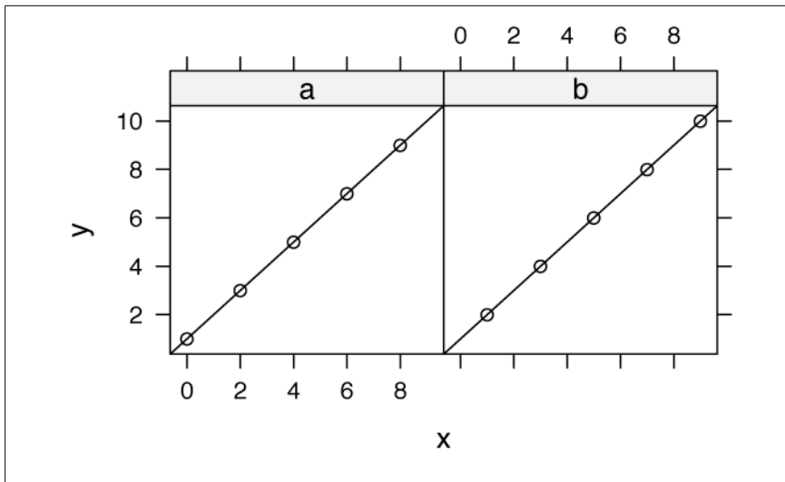
Figure 15-4. Scatter plot showing custom panel function
