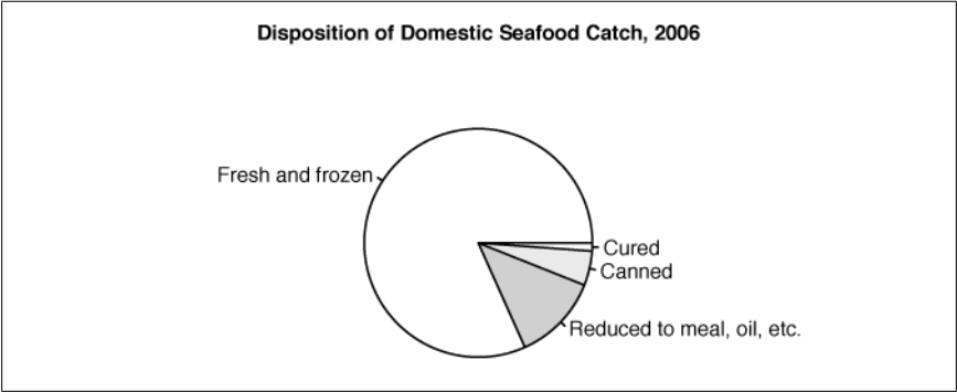
Figure 14-10. Pie chart
