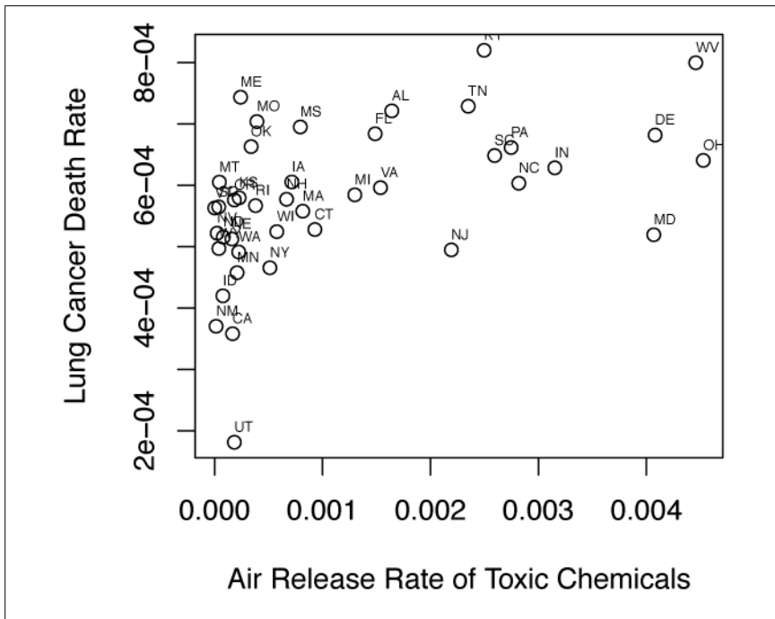
Figure 14-3. Toxins released by air and lung cancer deaths per capita, cleaned up
