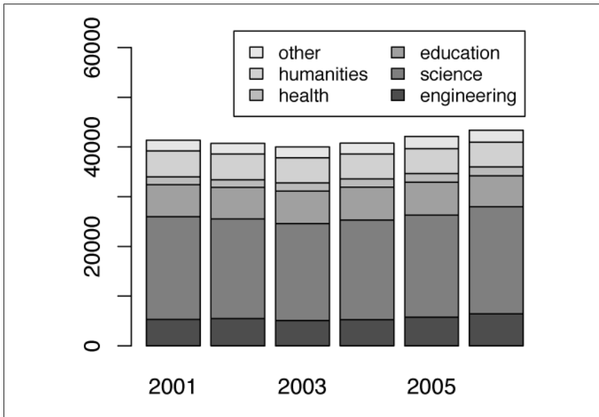
Figure 14-9. Stacked bar plot example
