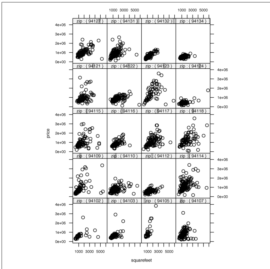
Figure 15-23. Scatter plot comparing house size and price by zip code
