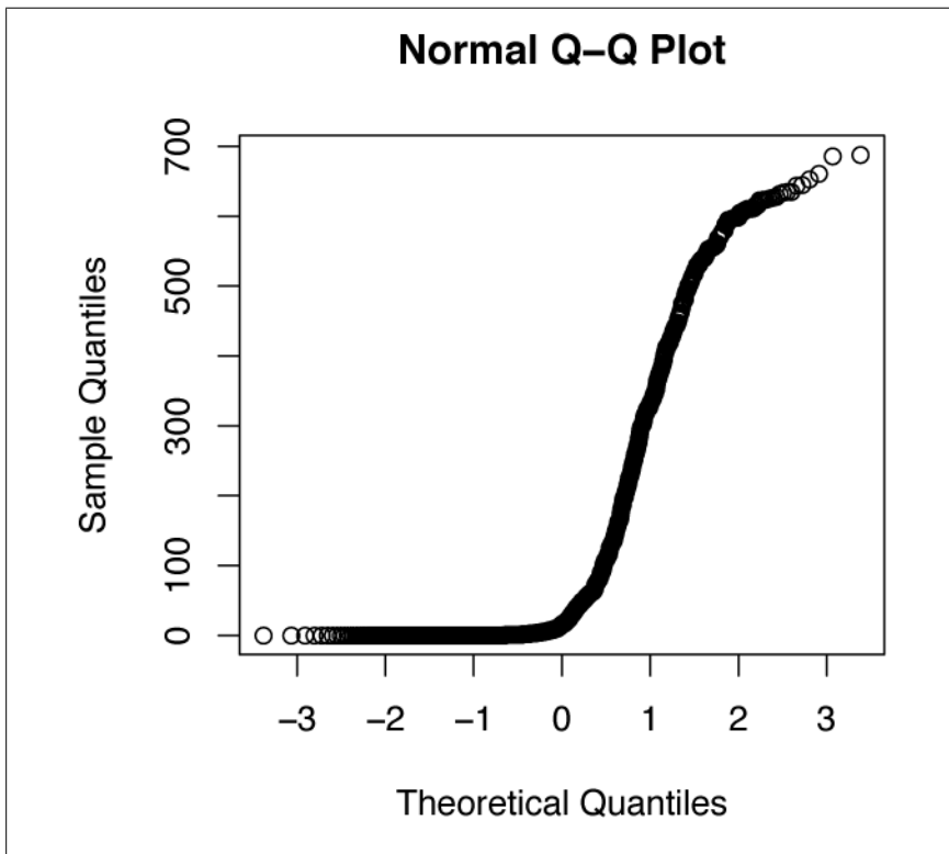
Figure 14-21. Quantile-quantile plot
