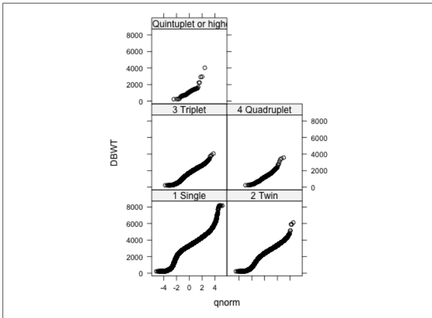
Figure 15-17. Quantile-quantile plots for birth weights
