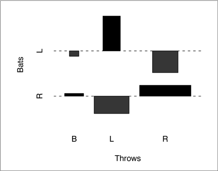
Figure 14-14. Association plot example
