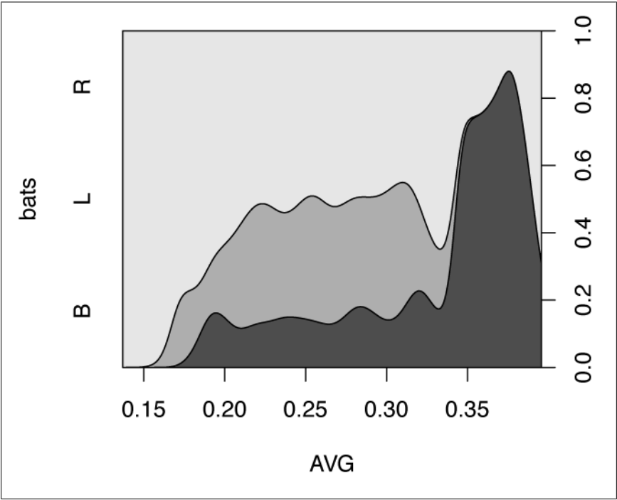
Figure 14-11. Conditional density plot
