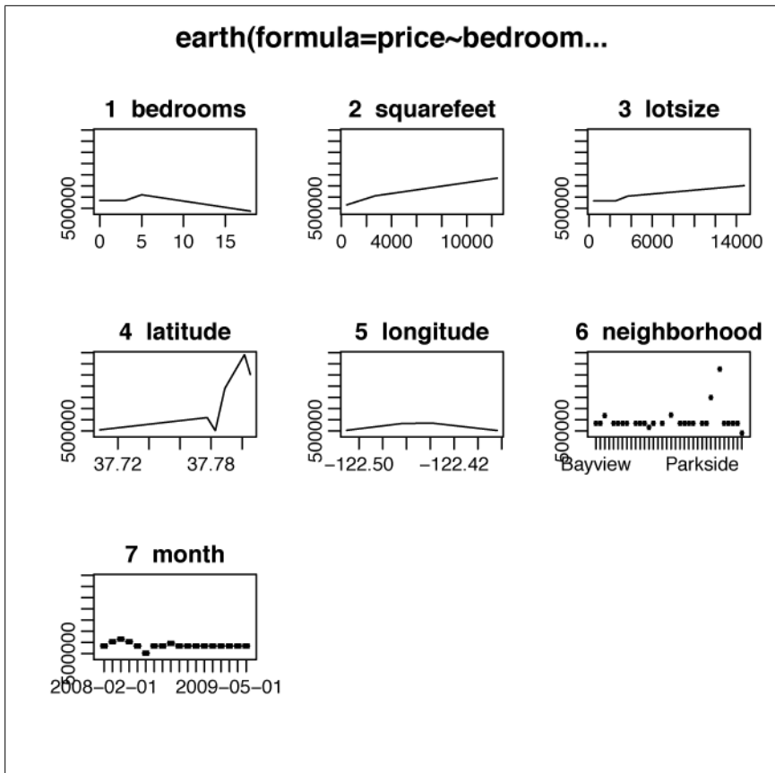
Figure 20-8. Output of plotmo
