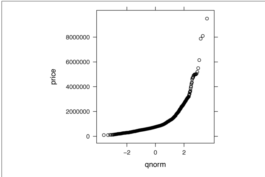
Figure 15-18. Quantile-quantile plot of San Francisco real estate prices
