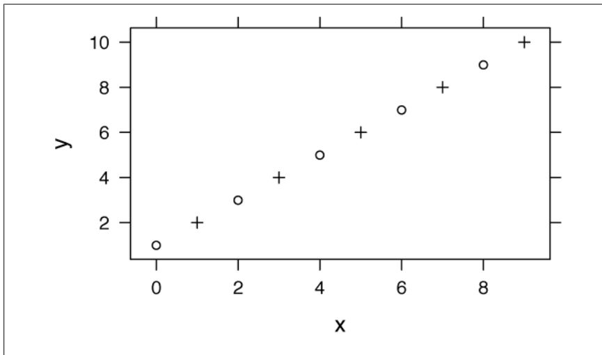
Figure 15-3. Scatter plot with grouping variable
