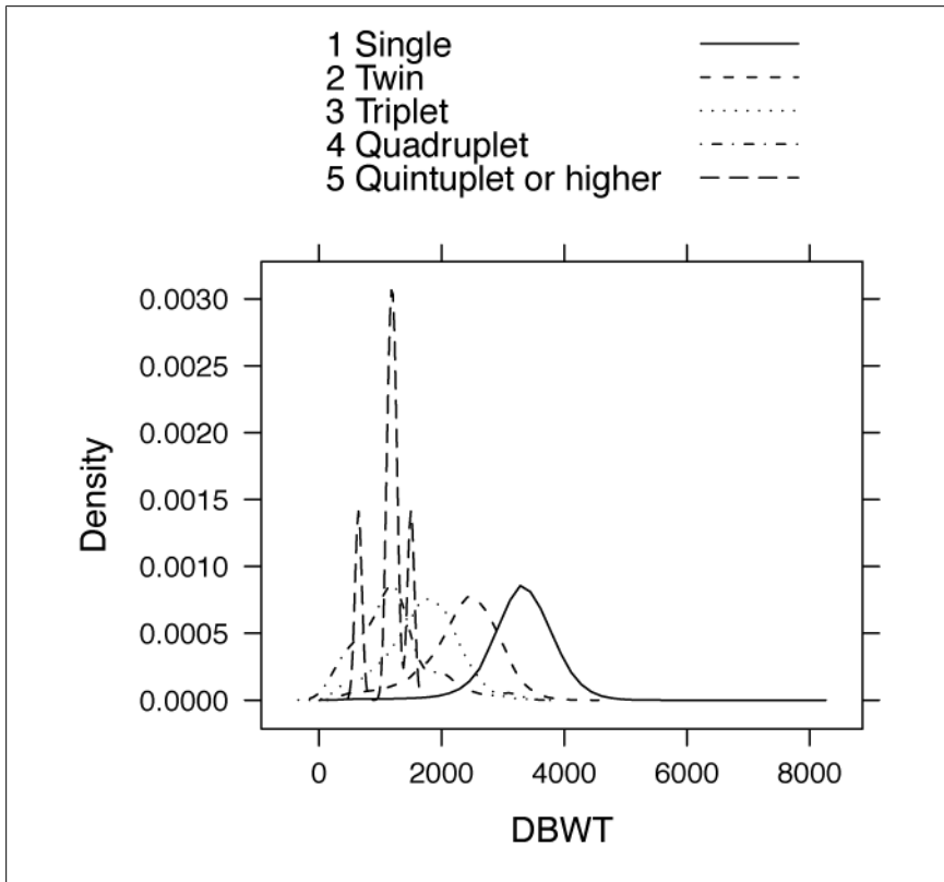
Figure 15-14. Superimposed density plots showing birth weight by number of babies
