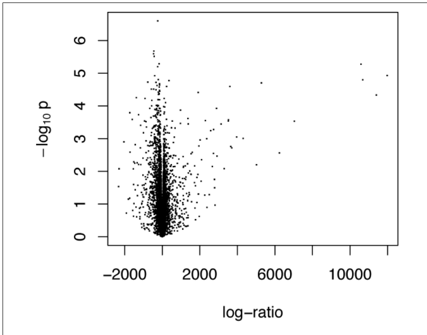
Figure 24-3. Volcano plot of filtered GSE2034 data
