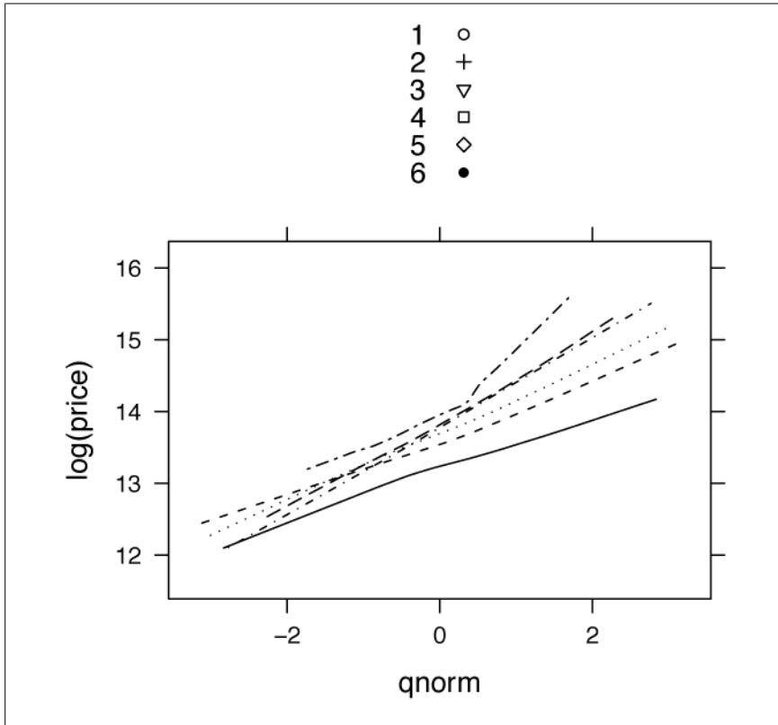
Figure 15-20. Quantile-quantile plots of logs of property prices for different numbers of bedrooms
