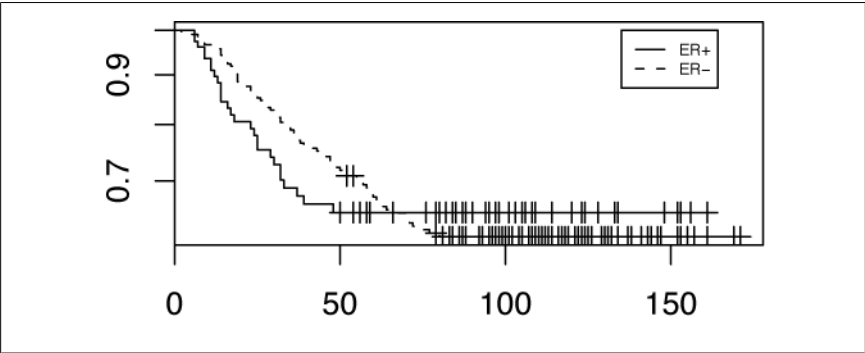
Figure 20-3. Survival curves for the GSE2034 data
