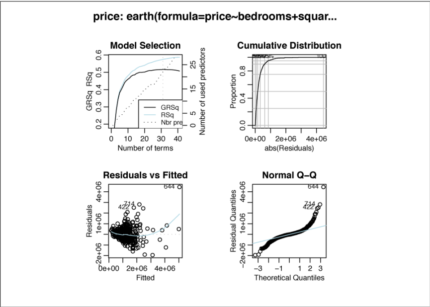
Figure 20-7. Output of plot.earth
