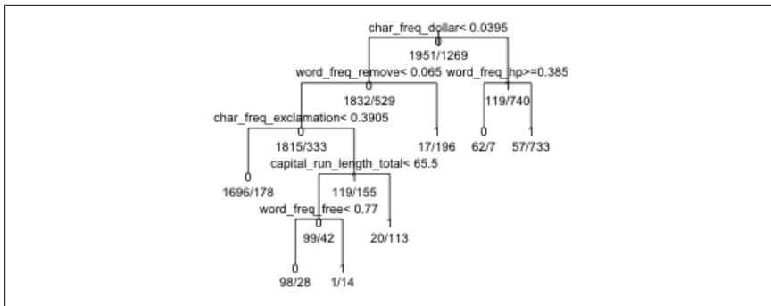
Figure 21-3. rpart tree for Spambase data, from plot.tree
