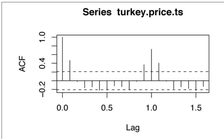
Figure 14-6. Autocorrelation function plot
