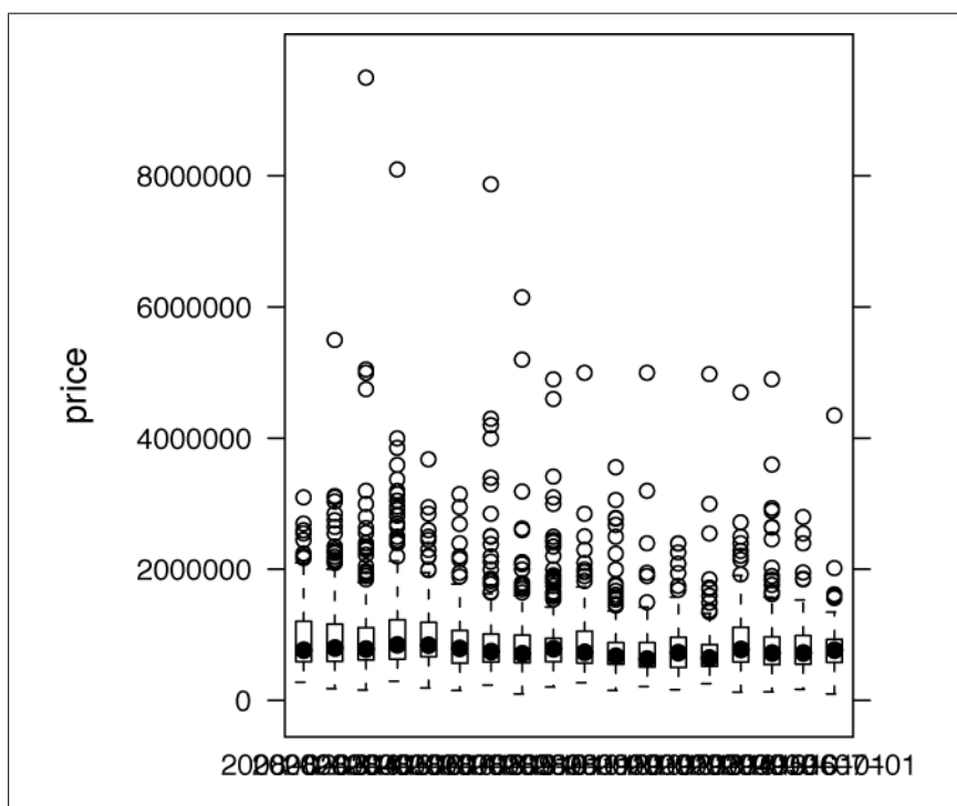
Figure 15-25. Box plot of real estate prices by month: first attempt
