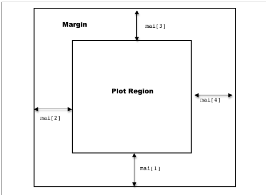
Figure 14-24. Margins around graphics area
