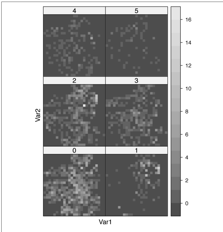
Figure 15-29. Level plot showing number of sales by location for different numbers of bedrooms
