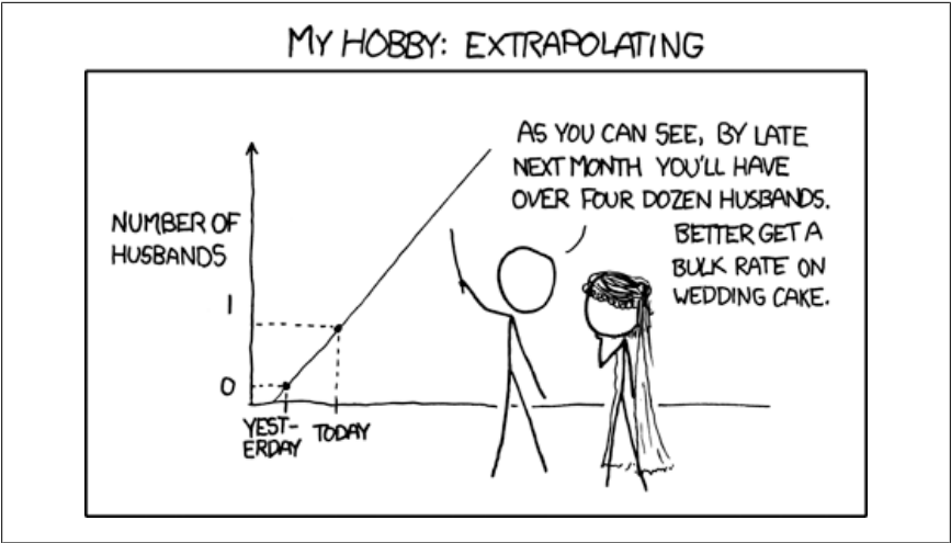
Figure 23-1. Extrapolating times series
