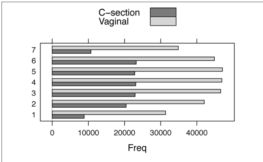
Figure 15-7. Births by day of week and method: unstacked bars
