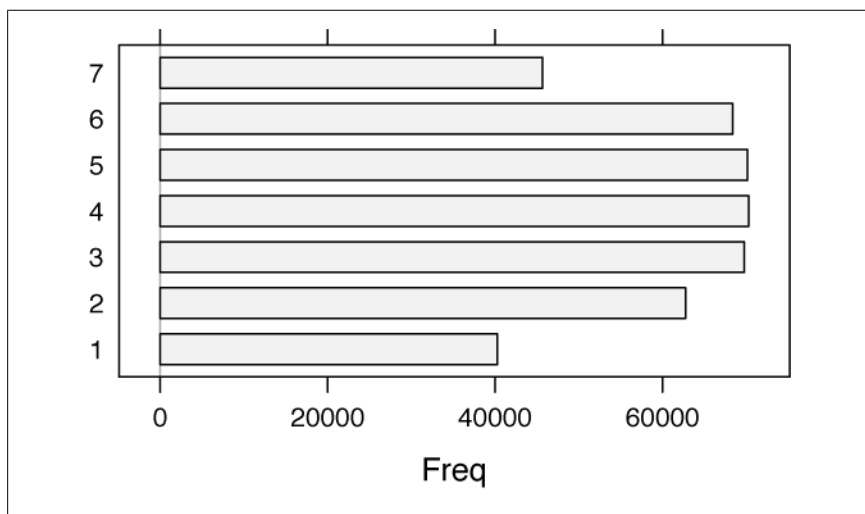
Figure 15-5. Births by day of week
