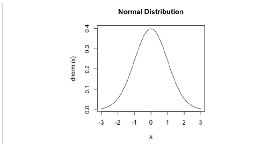
Figure 17-1. Normal distribution
