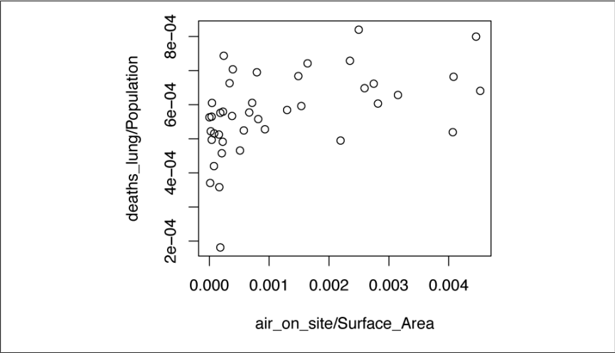
Figure 14-2. Toxins released by air and lung cancer deaths per capita
