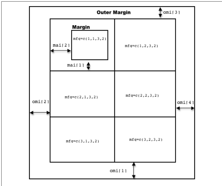
Figure 14-26. Multiple figure layout
