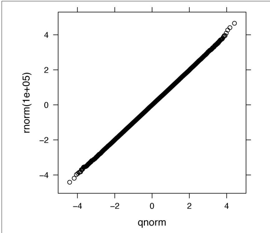
Figure 15-16. Quantile-quantile plot for random values from normal distribution
