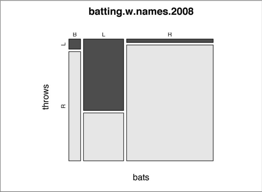
Figure 14-12. Mosaic plot
