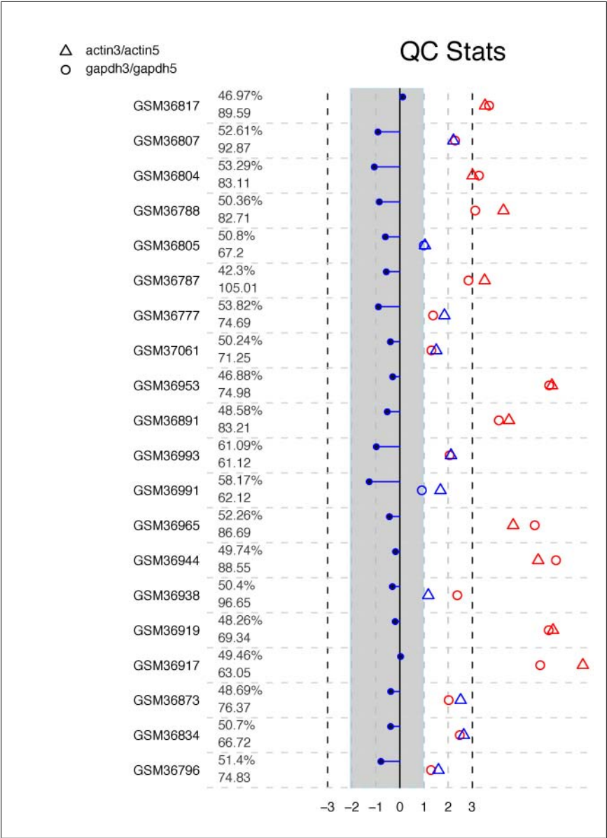
Figure 24-1. QC plot
