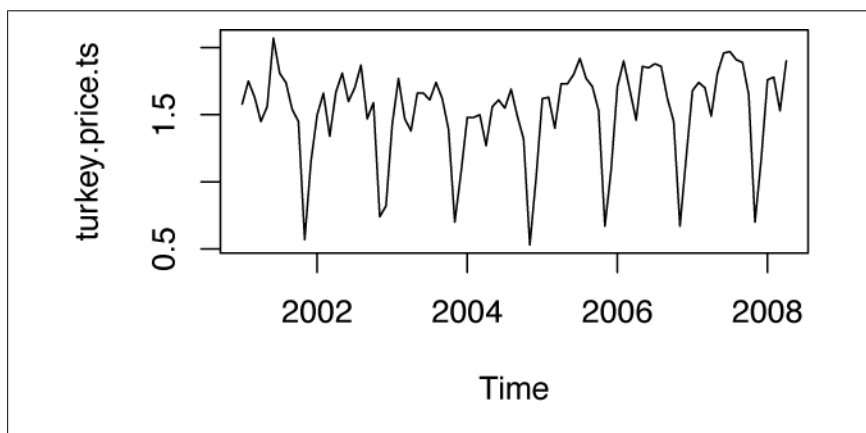
Figure 14-5. Time series plot
