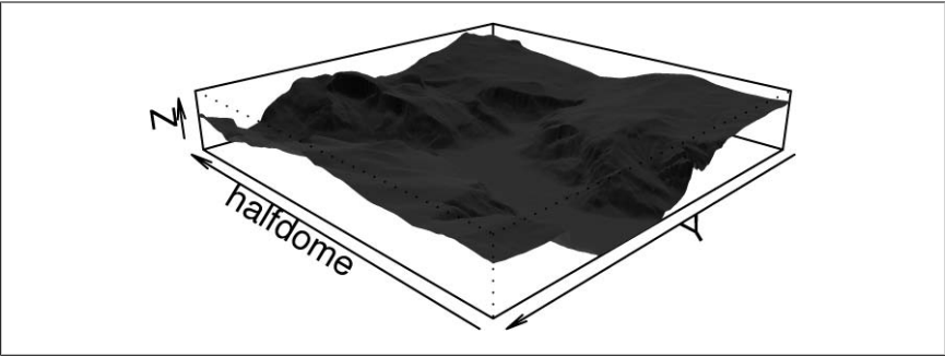
Figure 14-15. Perspective view of Yosemite Valley
