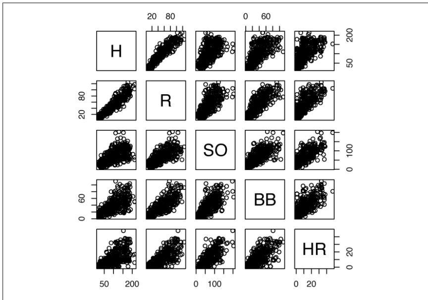
Figure 14-4. Pairs example
