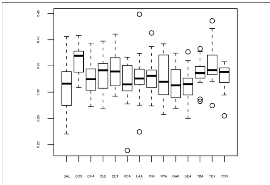
Figure 14-23. Box plot showing on-base percentage for players in the AL in 2008
