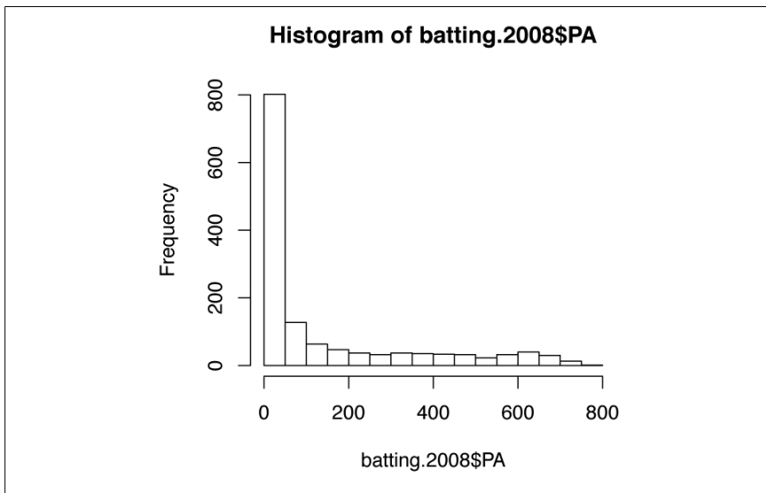
Figure 14-18. Histogram showing the distribution of plate appearances in 2008
