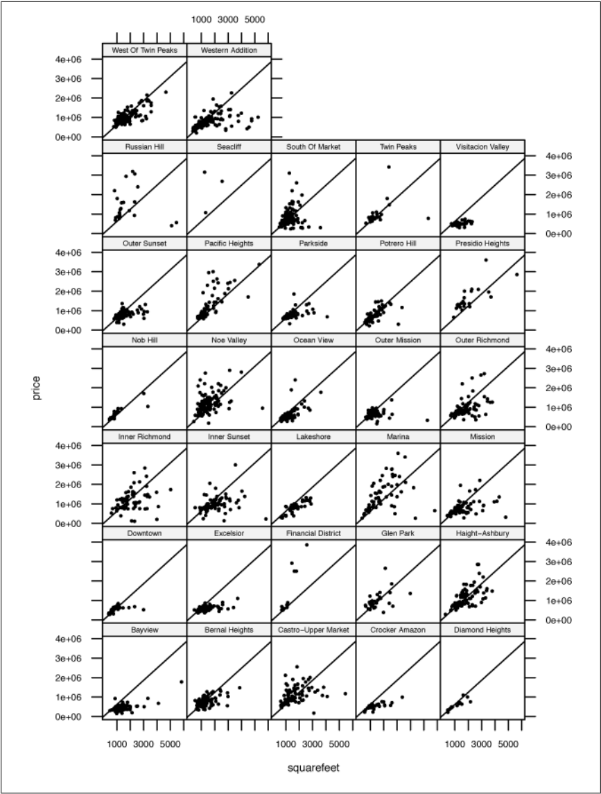
Figure 15-24. Scatter plot comparing house size and price by neighborhood
