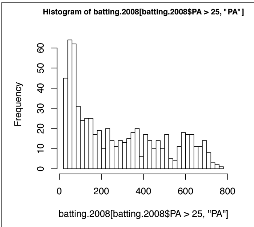
Figure 14-19. Histogram showing the number of plate appearances for players with over 25 plate appearances in 2008
