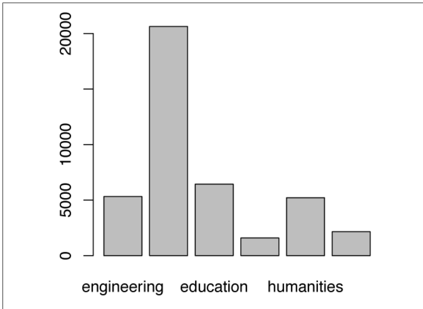
Figure 14-7. Simple bar plot example
