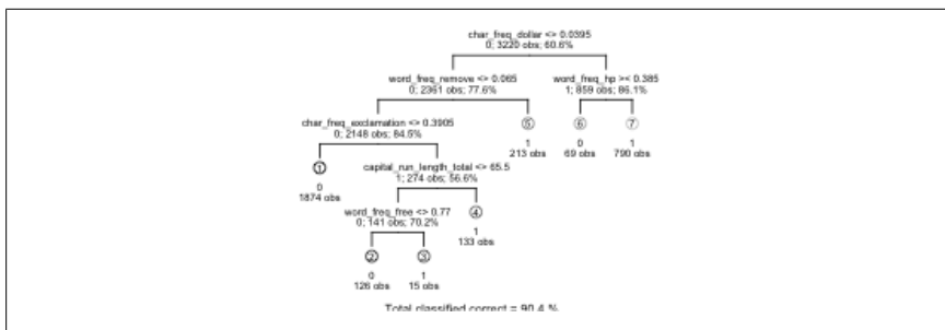
Figure 21-4. rpart tree for Spambase data, plotted by draw.tree
