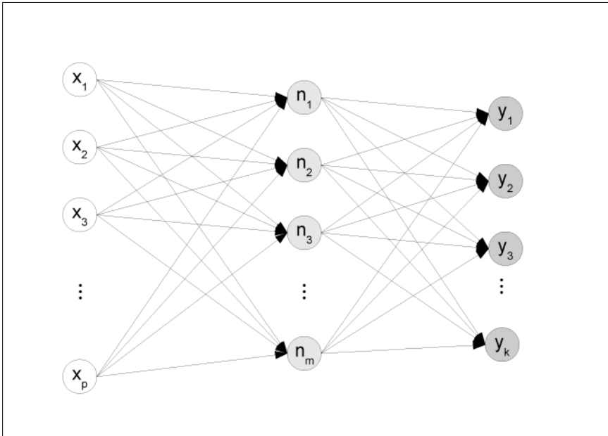
Figure 20-9. Single-hidden-layer, feed-forward neural network
