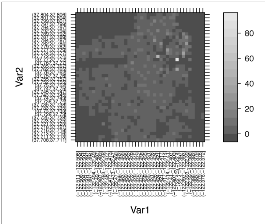
Figure 15-27. Level plot showing number of sales by location
