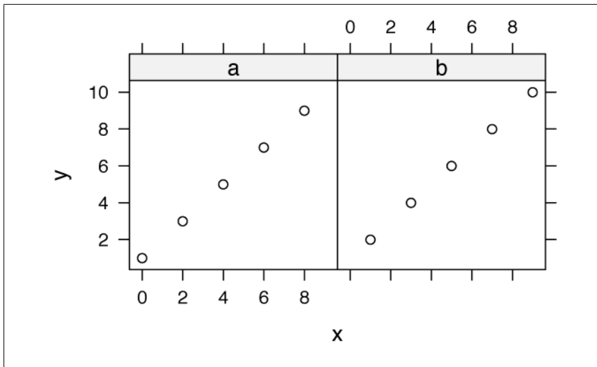
Figure 15-2. Simple scatter plot with conditioning variable
