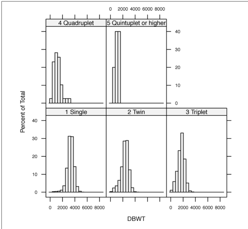
Figure 15-11. Histogram of birth weights by number of births
