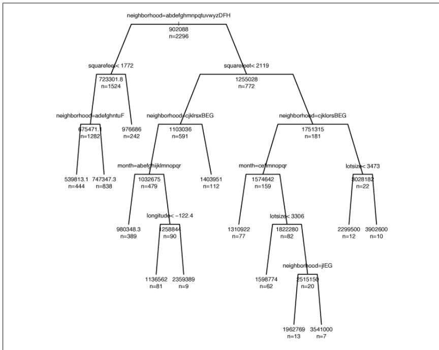
Figure 20-4. rpart tree for the San Francisco home sales model
