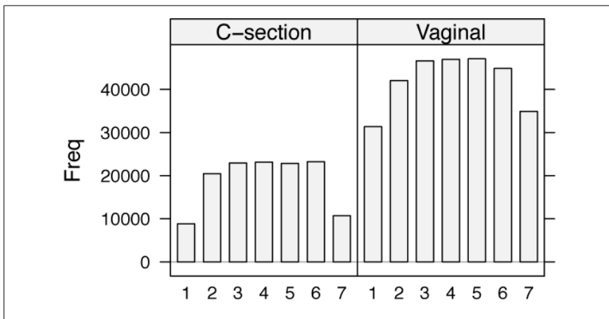
Figure 15-8. Births by day of week and method: two panels of columns
