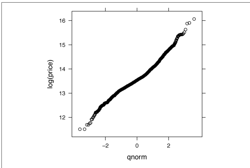
Figure 15-19. Quantile-quantile plot of log-scaled property prices
