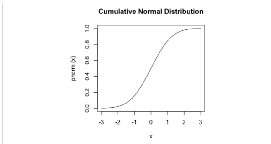
Figure 17-2. Cumulative normal distribution
