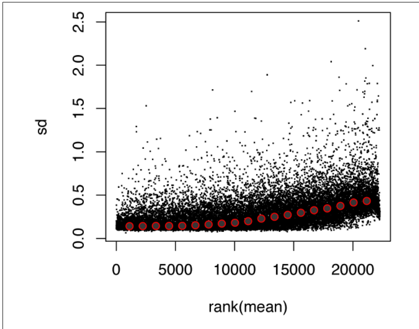
Figure 24-2. Row standard deviation versus row means, from meanSdPlot
