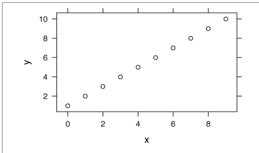
Figure 15-1. Simple scatter plot example
