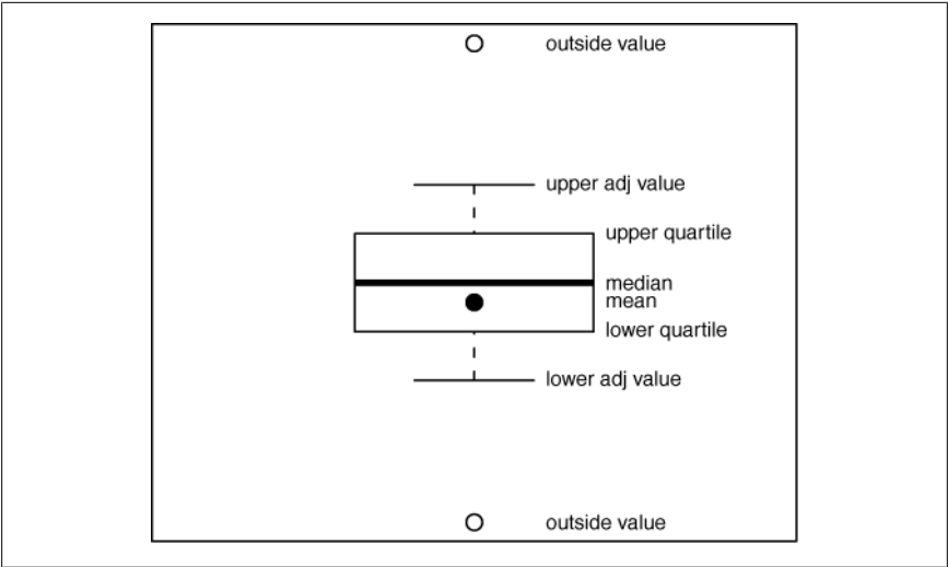
Figure 14-22. Box plot components
