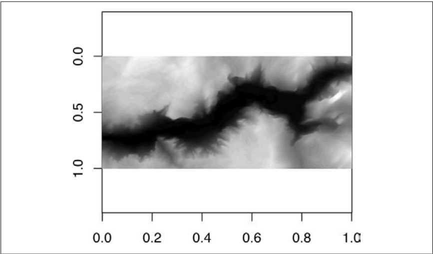
Figure 14-16. Image example: Yosemite Valley
