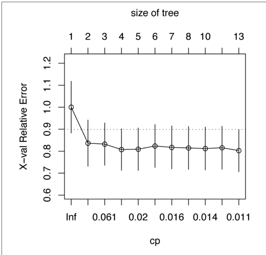
Figure 20-6. Output of plotcp for the sf.prices.rpart model
