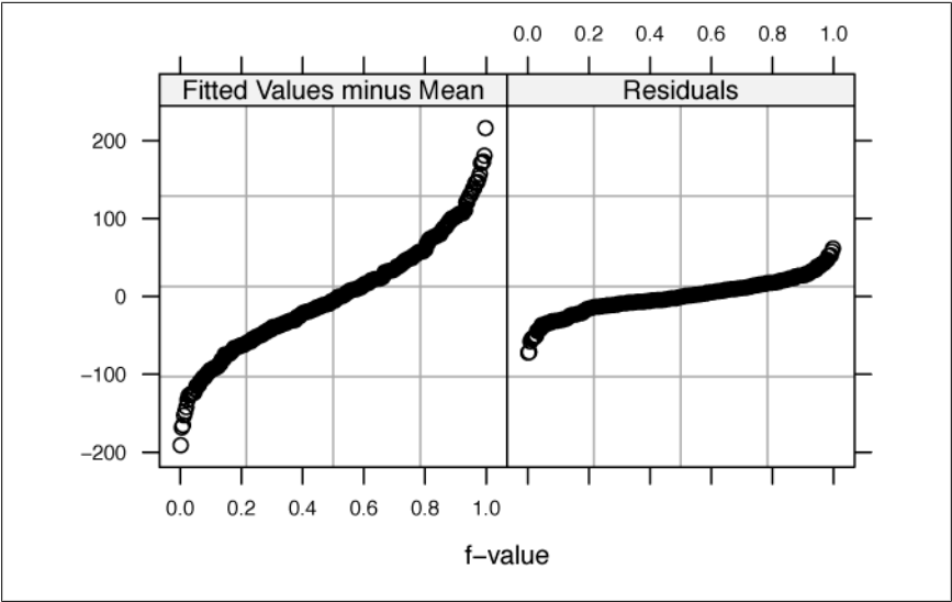
Figure 15-30. RFS plot for runs model (uniformly distributed residuals)
