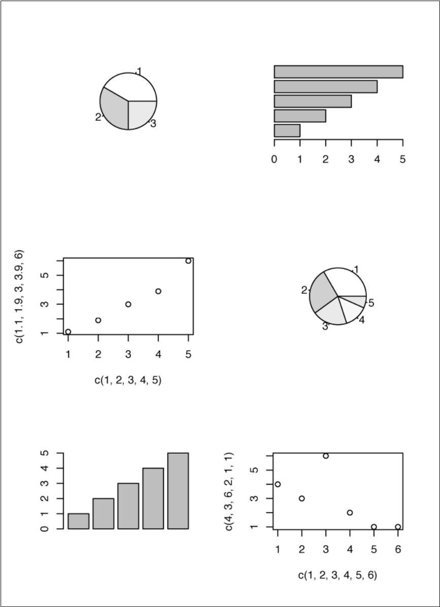
Figure 14-25. Multiple-figure example
