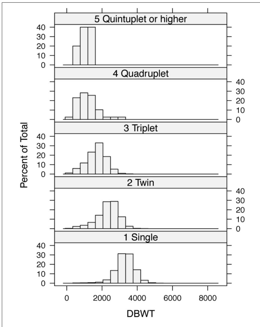
Figure 15-12. Histogram of birth weights by number of births: vertically stacked
