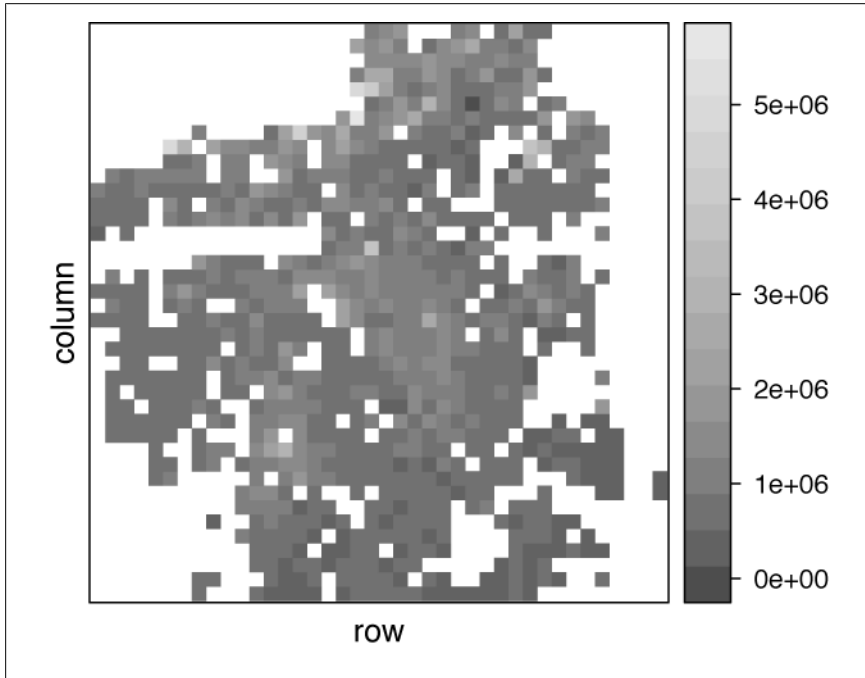
Figure 15-28. Level plot showing mean price by location
