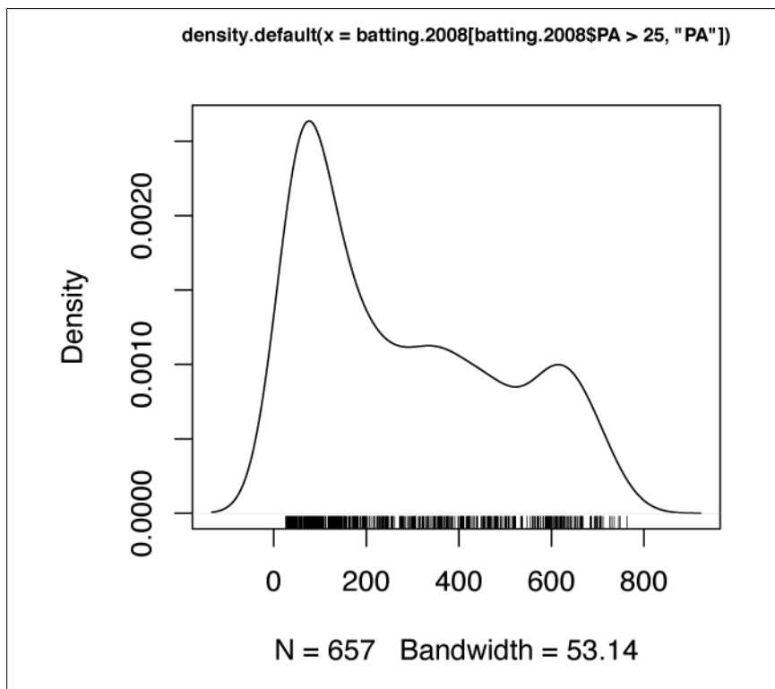
Figure 14-20. Density plot of plate appearances with rug
