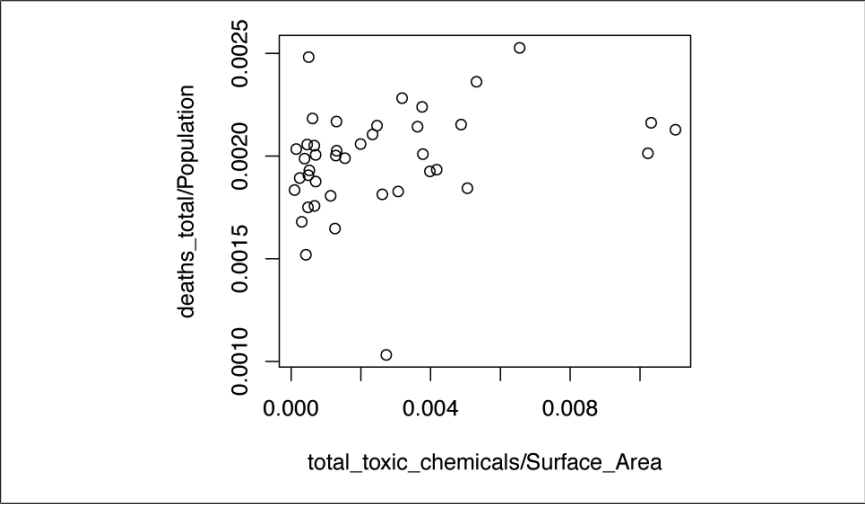
Figure 14-1. Total toxins and new cancer cases
