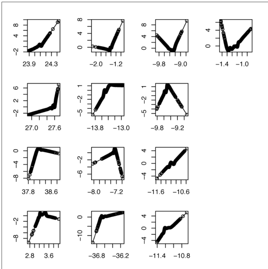
Figure 20-10. Ridge functions from projection pursuit model
