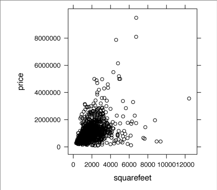
Figure 15-22. Scatter plot comparing house size and price
