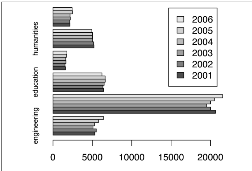
Figure 14-8. Horizontal juxtaposed bar plot example
