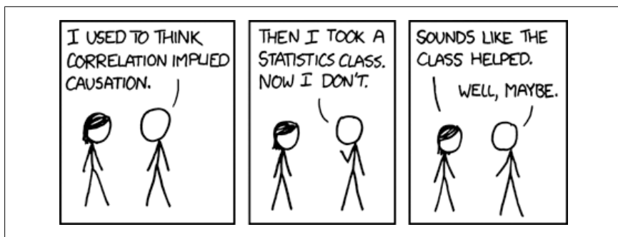
Figure 16-1. Correlation
