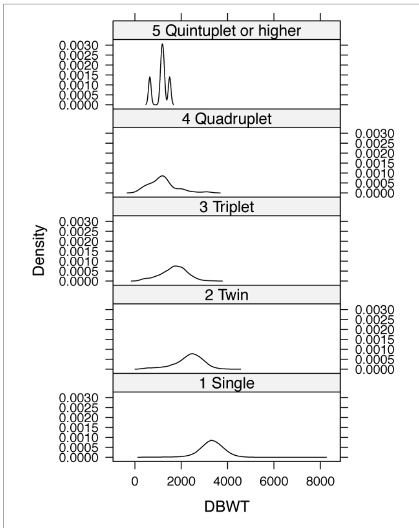
Figure 15-13. Density plots showing birth weight by number of babies
