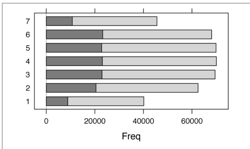
Figure 15-6. Births by day of week and method
