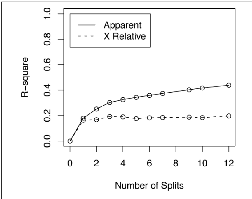
Figure 20-5. Plot from rsq.rpart(sf.price.model.rpart)
