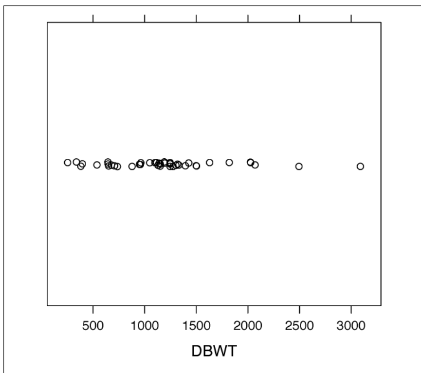
Figure 15-15. Weight of babies born in sets of four or more
