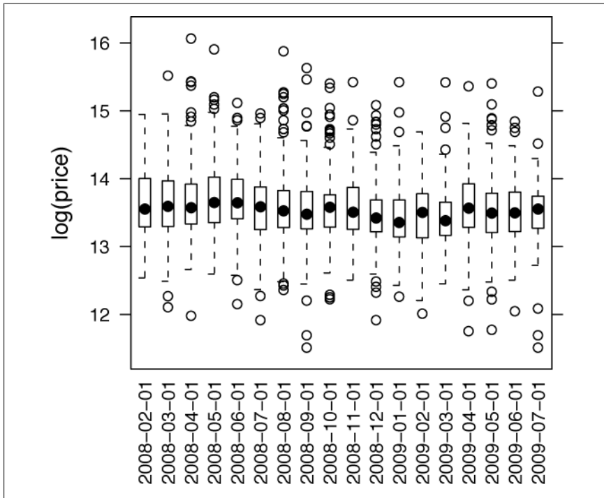
Figure 15-26. Box plot of real estate prices by month (log transformed)
