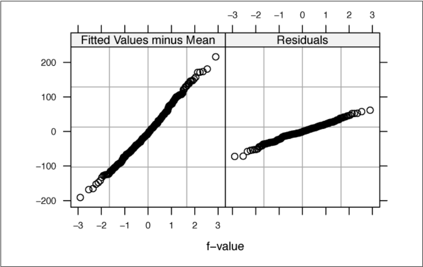
Figure 15-31. RFS plot for runs model (normally distributed residuals)
