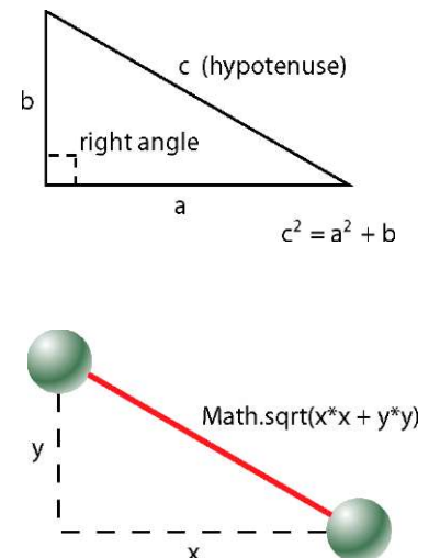
Figure 7-13. Calculating the distance between two points using geometry
