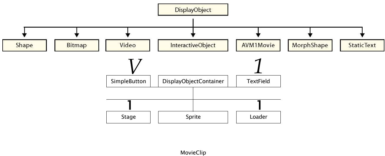
Figure 4-3. The display list classes
