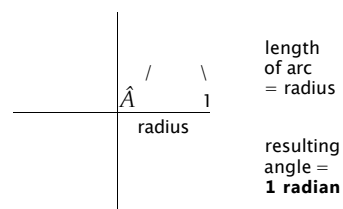
Figure 7-11. How radians are calculated
