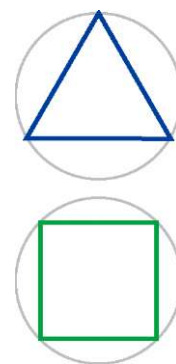
Figure 8-13. Forming polygons by dividing a circle's circumference into equal sections and then connecting the equidistant points
