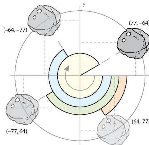
Figure 7-15. Four angles around a circle, expressed in degrees, radians, and as x and y points on a circle with a radius of 100 pixels
