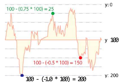
Figure 11-9. A few sample amplitude calculations, and where they appear in an example waveform
