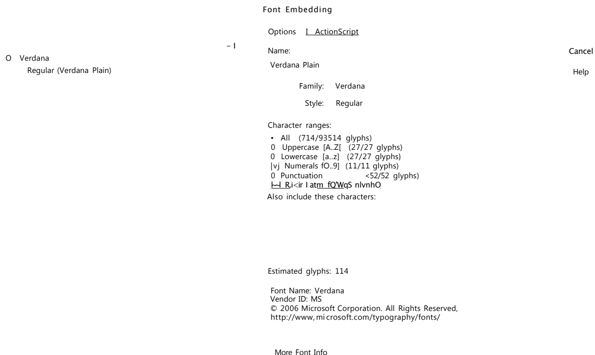
Figure 10-5. Flash Professional CS5's Font Embedding dialog, showing the Options tab
