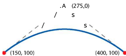
Figure 8-2. A quadratic Bézier curve with one control point for both end points of a line segment
