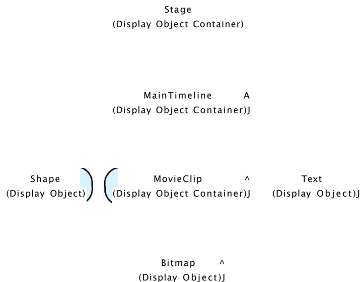
Figure 4-2. The display list of the sample file
