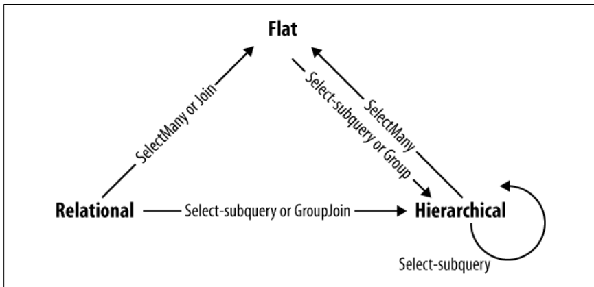
Figure 9-1. Shape-changing operators
