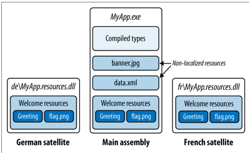
Figure 17-4. Resources
