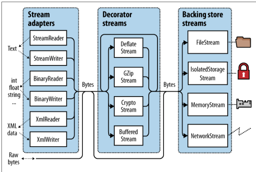
Figure 14-1. Stream architecture
