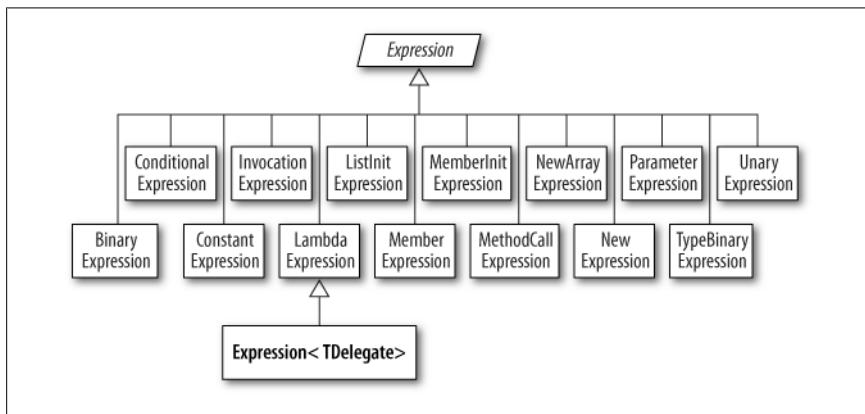
Figure 8-11. Expression types
