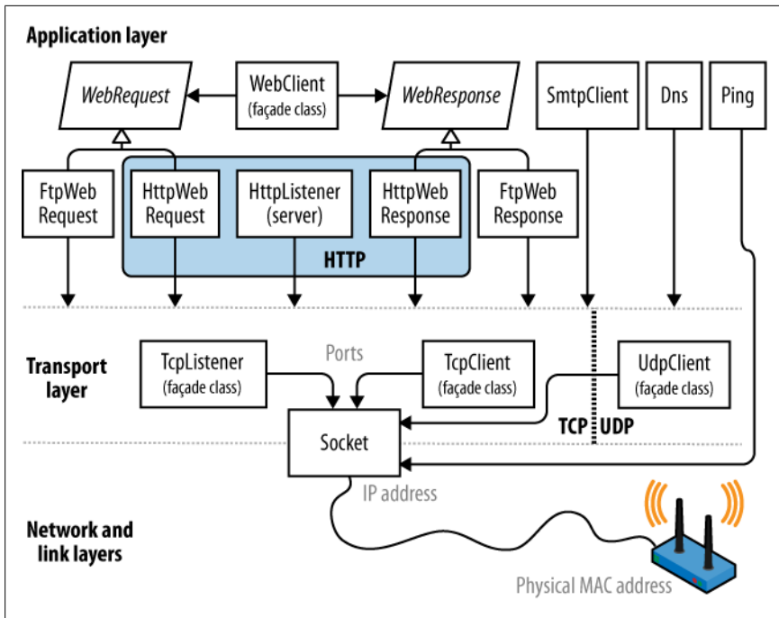
Figure 15-1. Network architecture
