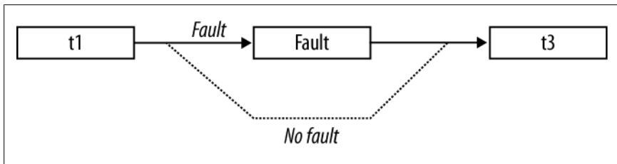
Figure 22-6. Conditional continuations
