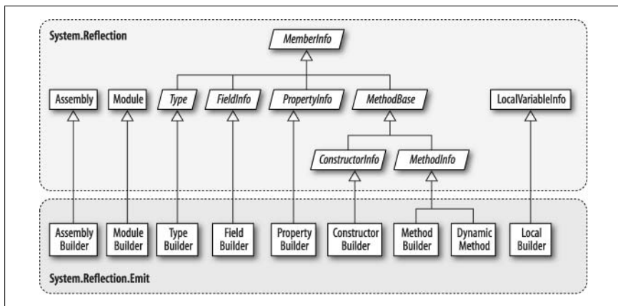
Figure 18-2. System.Reflection.Emit
