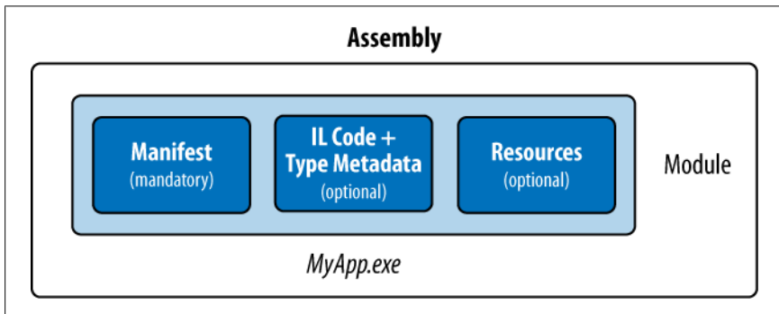
Figure 17-1. Single-file assembly
