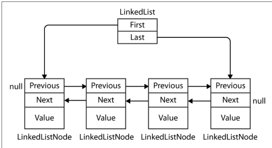
Figure 7-4. LinkedList<T>
