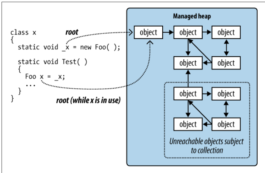
Figure 12-1. Roots
