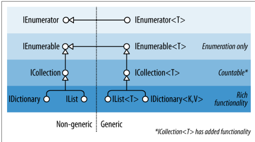
Figure 7-1. Collection interfaces
