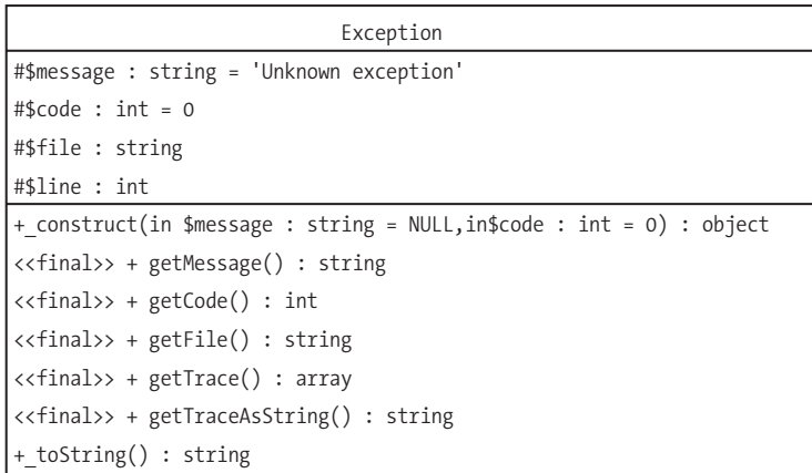
Figure 2-5. The PHP 5 Exception class (UML representation)
