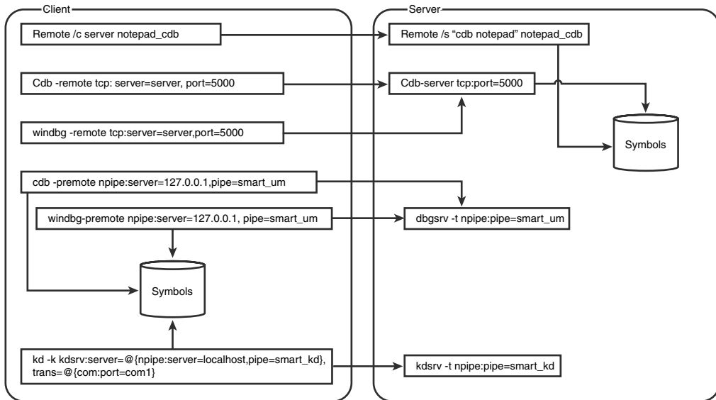
Figure 2.6 Remote debugging and symbol resolution
