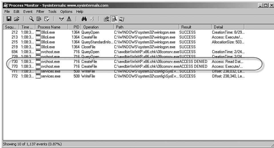
Figure 7.8 Detecting file errors using the tracing tools
