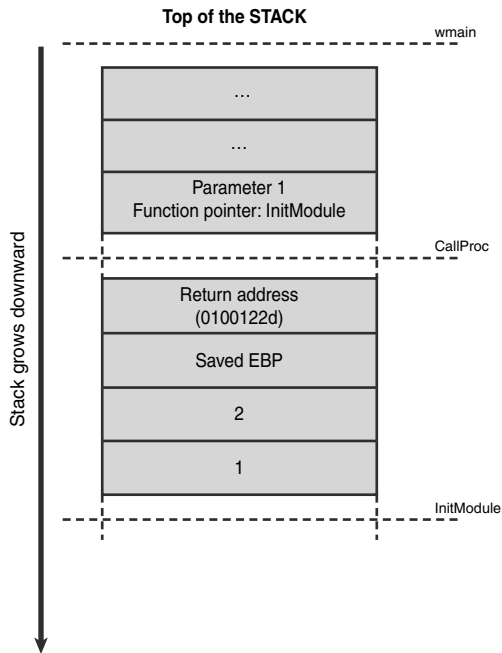
Figure 5.10 Expected stack prior to calling InitModule
