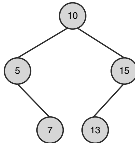
Figure 11.1 Tree representation after insertion of 10, 5, 15, 7, and 13
