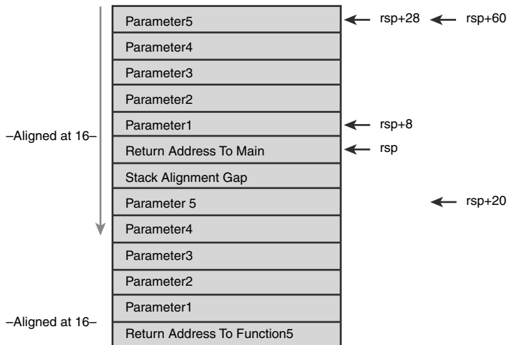
Figure 12.3 Stack usage on x86-64 calling stack
