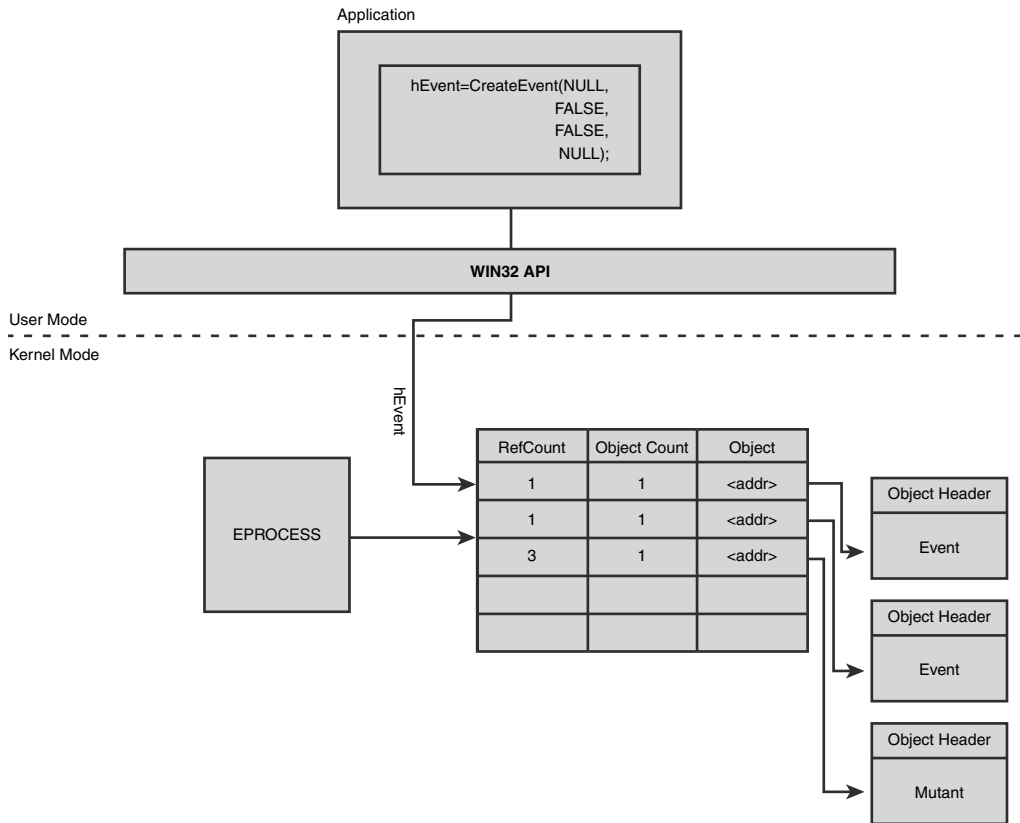
Figure 9.4 Windows handle architecture overview
