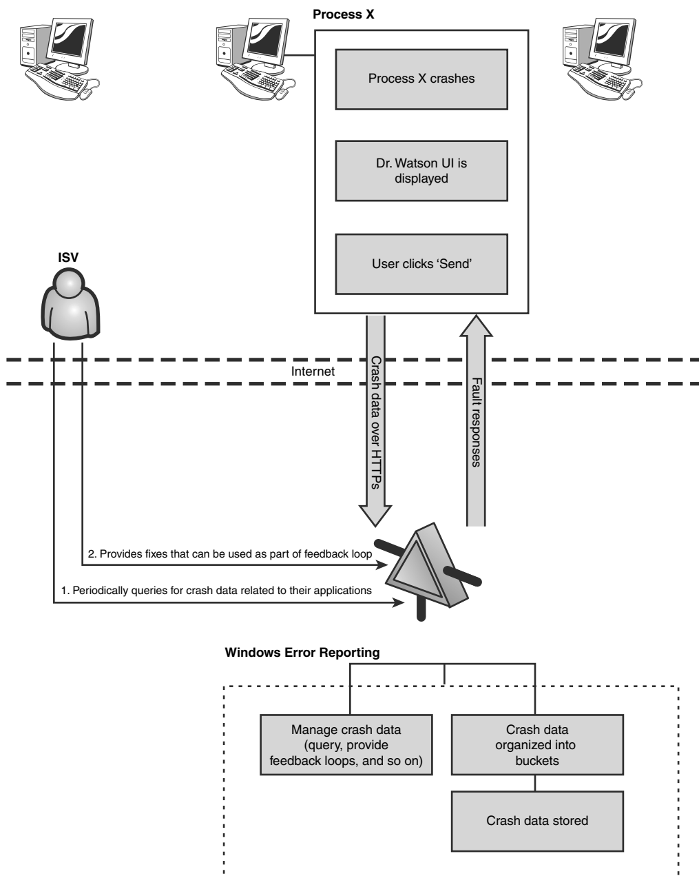
Figure 13.6 High-level overview of WER functionality
