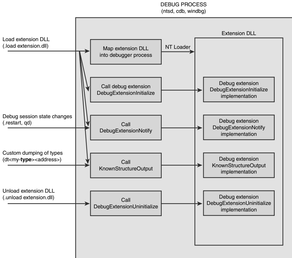
Figure 11.4 The process of loading and unloading an extension DLL
