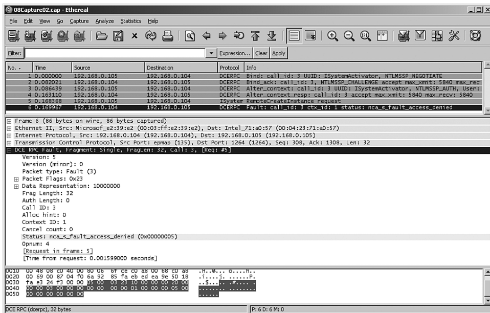
Figure 8.6 Packets captured during a failed DCOM activation
