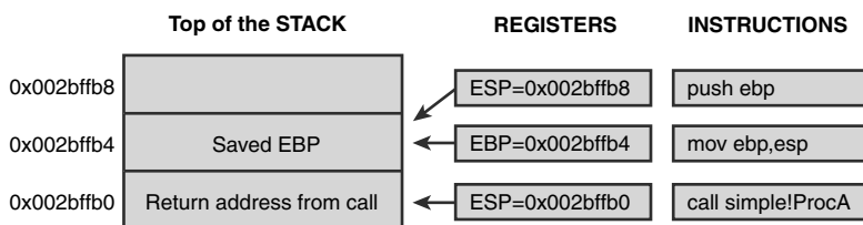
Figure 5.4 Contents of stack prior to calling ProcA
