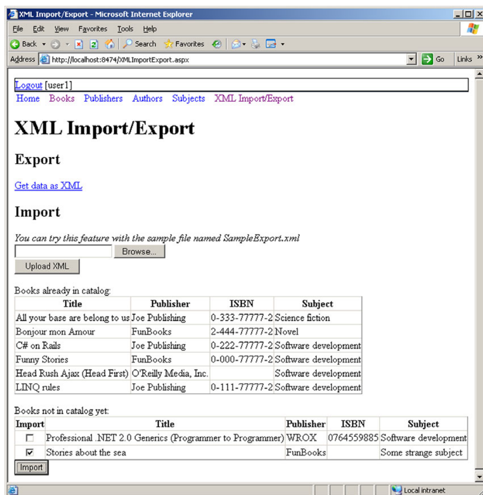
Figure 13.12 The XML import/export page displaying data from an uploaded XML document
