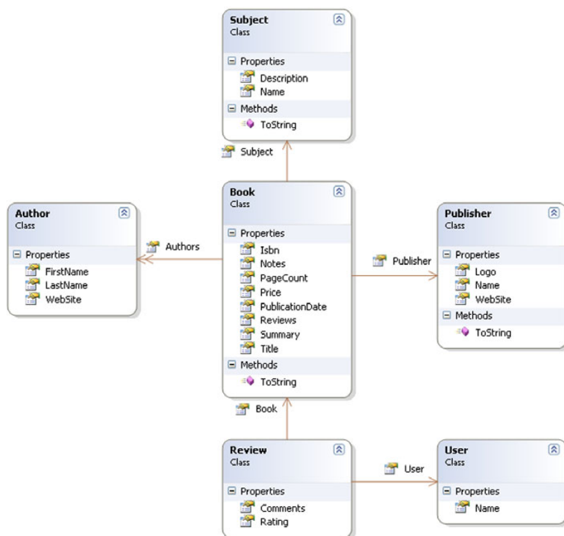
Figure 4.1 Object model for the running example
