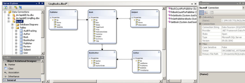
Figure 7.1 Mapping the LINQinAction database using the LINQ to SQL designer tool
