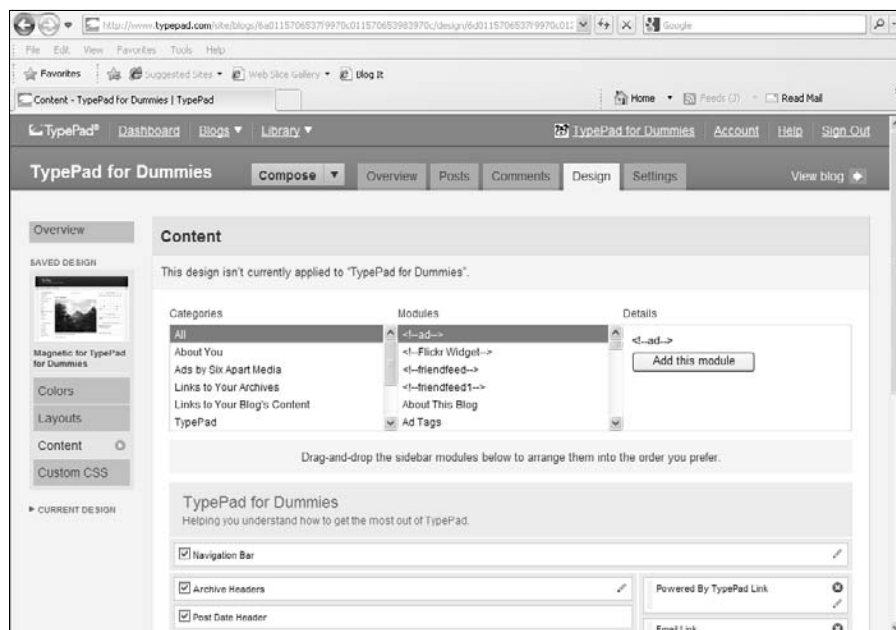
Figure 11-5: Drag-and-drop editor.
