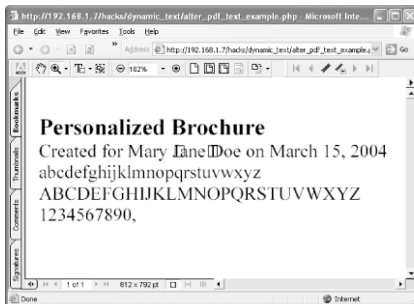
Figure 6-14. Acrobat displaying parentheses around "Jane" as empty rectangles, because we omitted them from our alphabet soup
