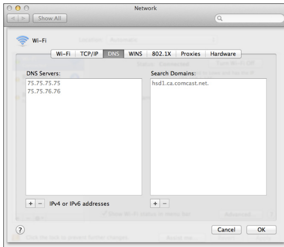
Figure 26-4: DNS settings.
