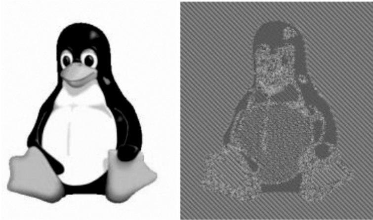
Figure 15–2. Wikipedia's illustration of the pattern flaw in ECB mode encryption. This image is licensed under the GNU Free Documentation License at http://www.gnu.org/copyleft/fdl.html . It is from the Wikipedia article “Block Cipher Modes of Operation” at http://en.wikipedia.org/wiki/Block_cipher_modes_of_operation .
