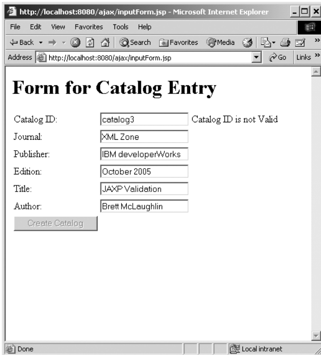
Figure 13-8. Validating a catalog entry previously defined
