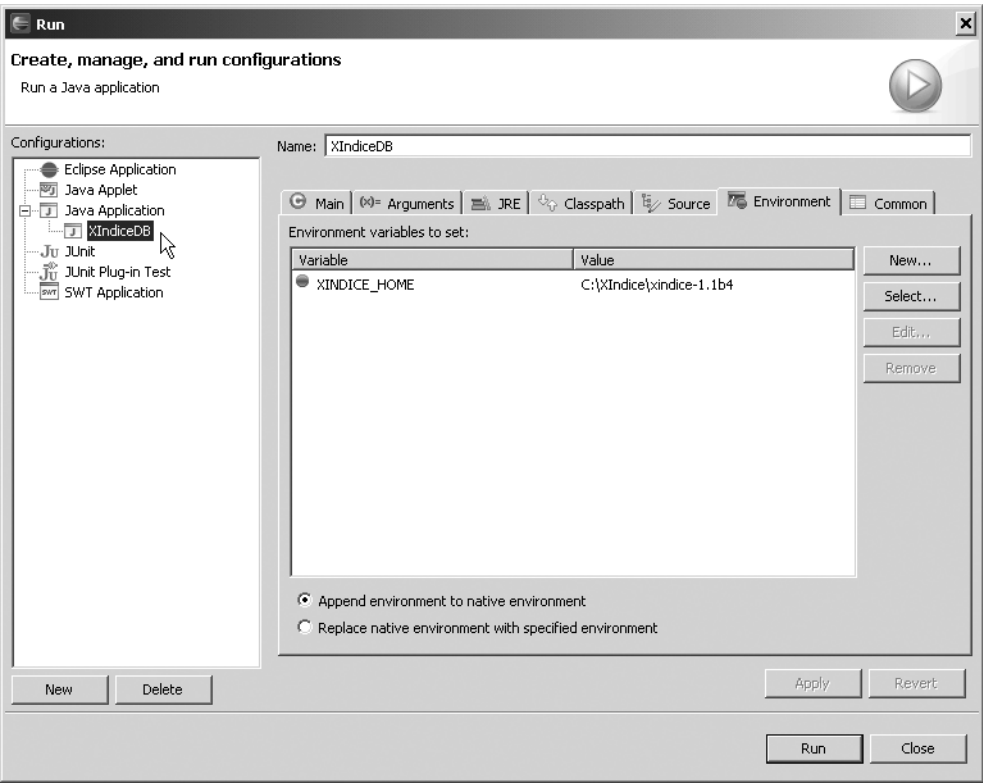
Figure 8-4. XIndexDB.java application environment variables
