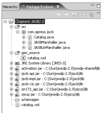
Figure 6-11. Chapter6 Eclipse project directory structure
