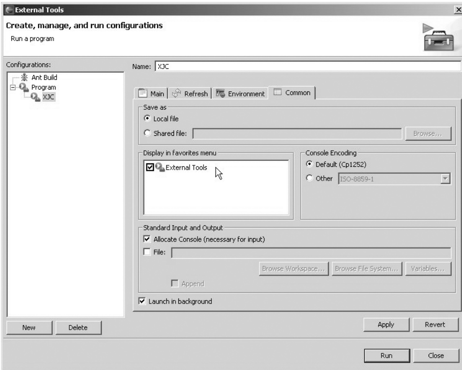
Figure 6-7. Adding the xjc configuration to the external Tools menu
