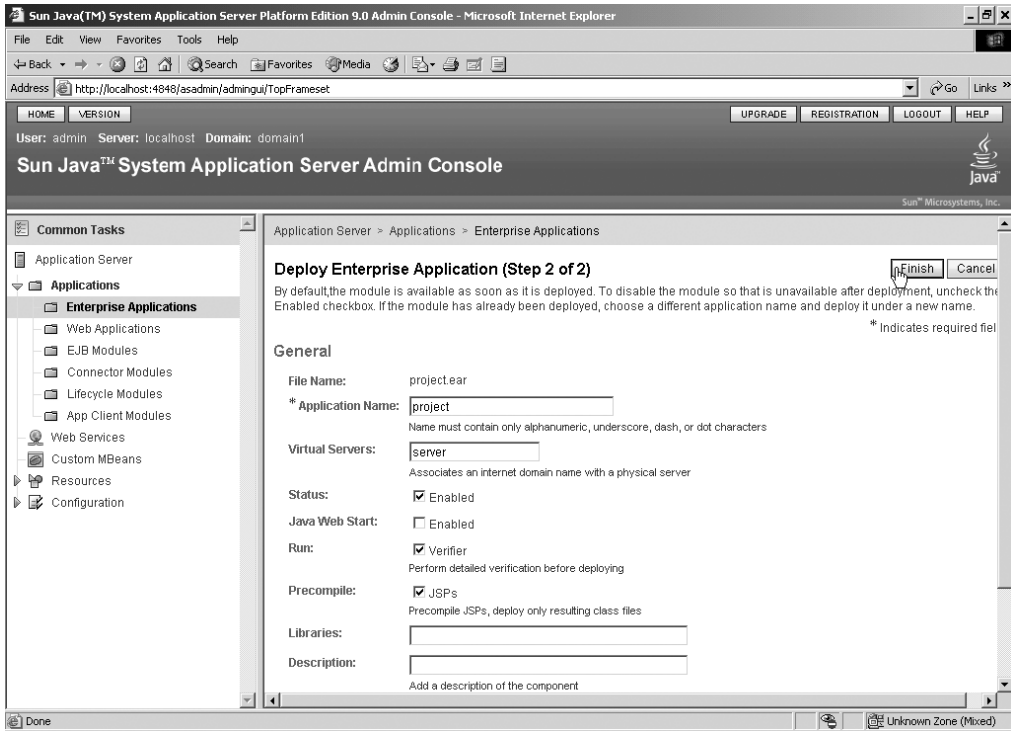
Figure 14-10. Configuring settings for and deploying the project.ear application
