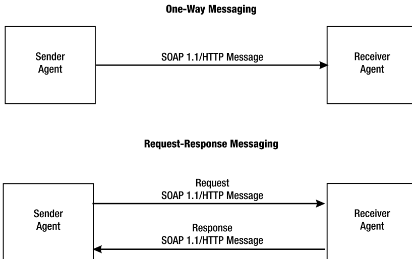
Figure 14-3. Message exchange patterns
