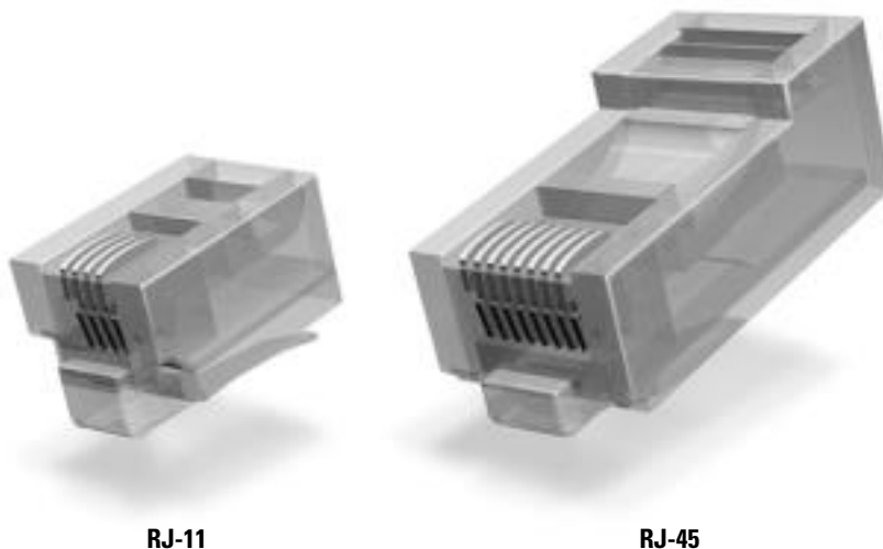
Figure 6-7: RJ-45 connectors are necessary for twisted-pair cabling; RJ-11 connectors are for phone wires.
