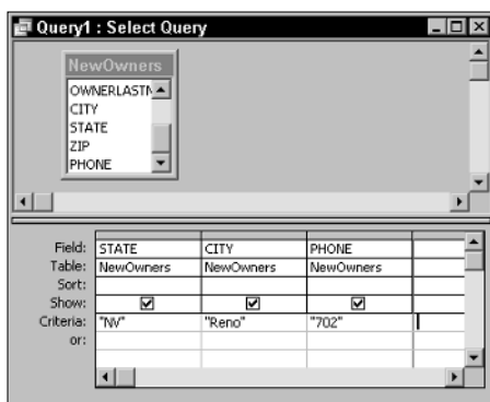
Figure 6-5: Create your select query that selects the records you want to update.
