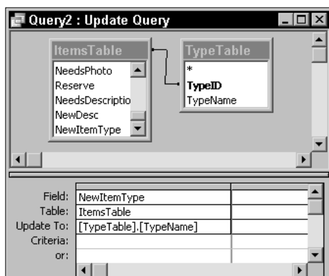
Figure 16-4: The finished query updates one table with data from another table.
