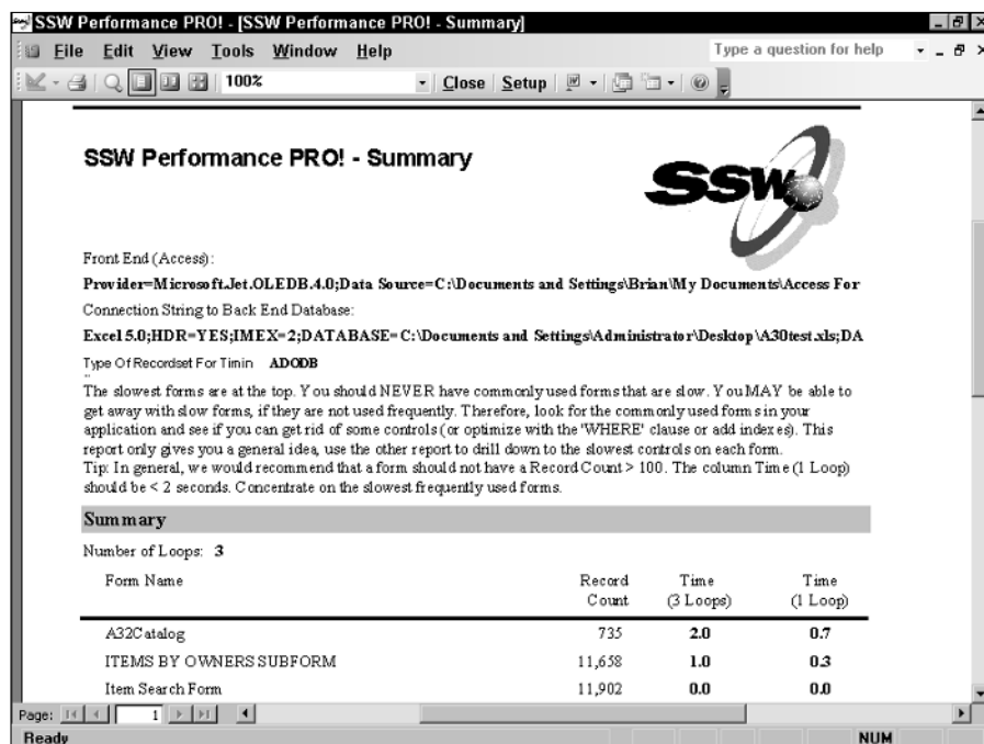
Figure 20-5: Find out what's making your forms too slow to use.
