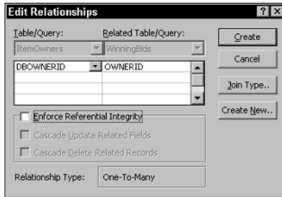
Figure 5-9: Use the Edit Relationship dialog box to specify the parameters for the relationship.
