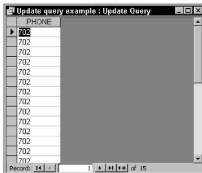
Figure 7-5: In Datasheet view you can see how records will be affected by your query.
