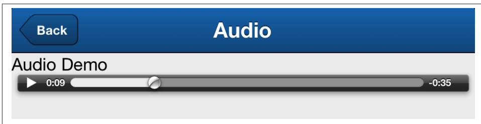
Figure 3-21. Embedded audio
