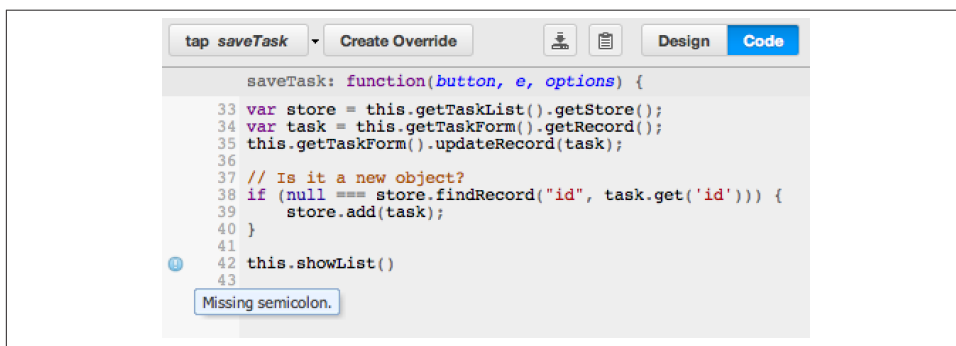
Figure 9-8. JSHint integration
