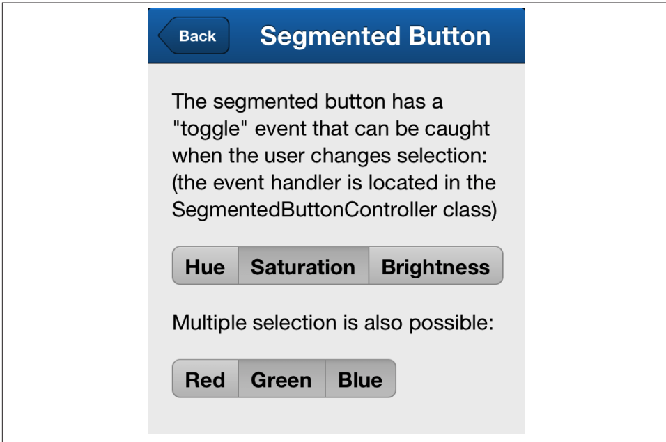
Figure 3-12. Segmented buttons
