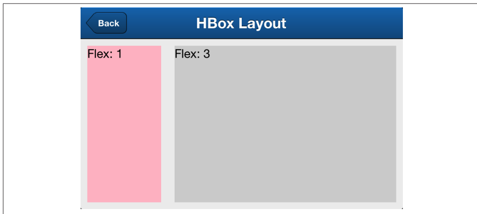
Figure 3-2. HBox layout
