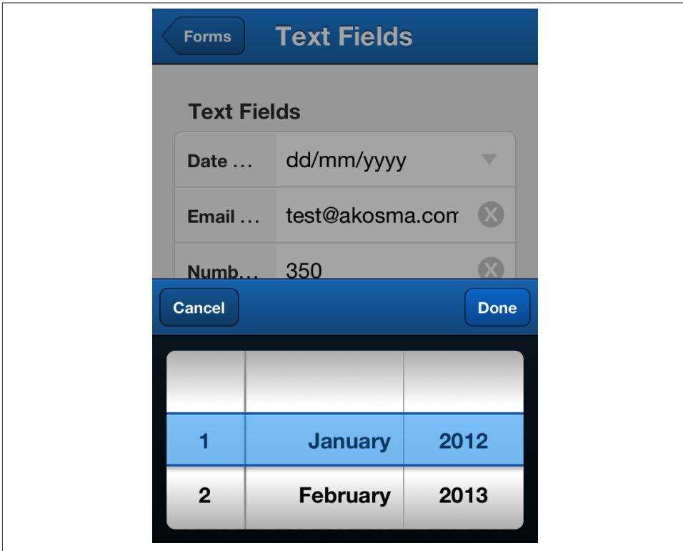
Figure 5-4. Date picker
