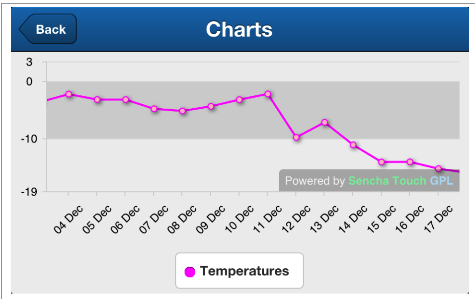
Figure 3-23. Charts
