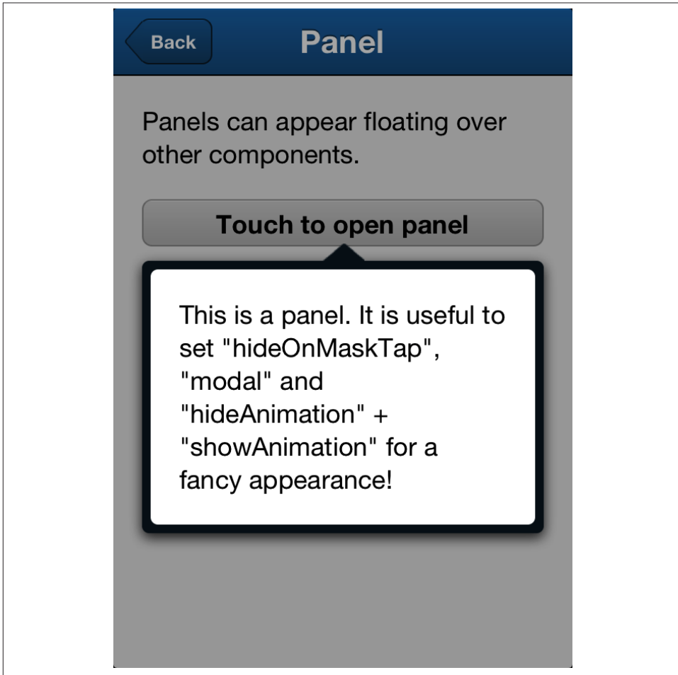
Figure 3-16. Floating panel
