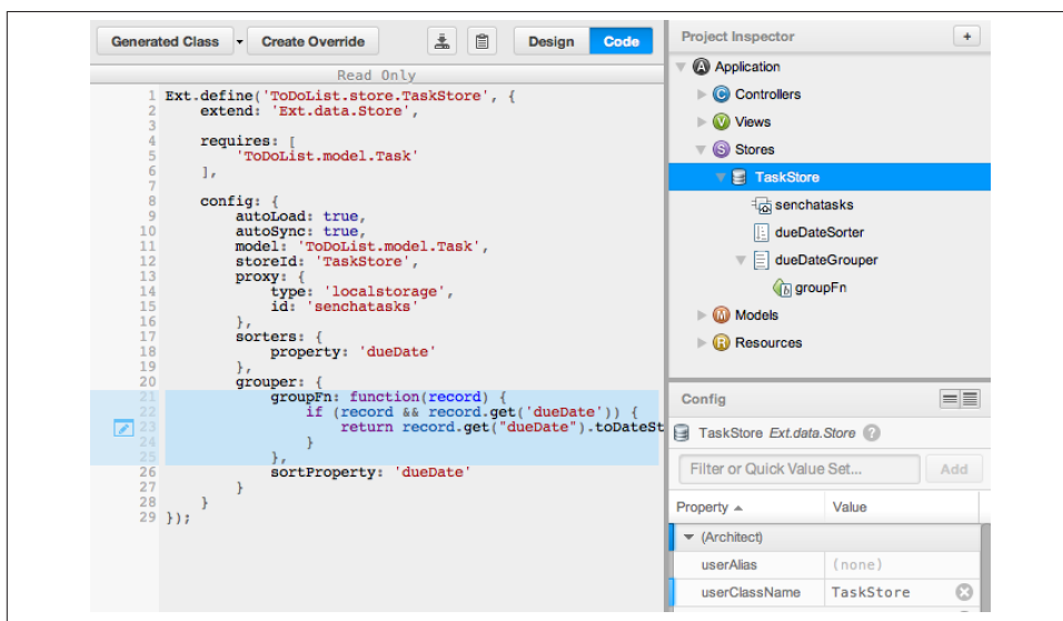
Figure 9-9. Store definition
