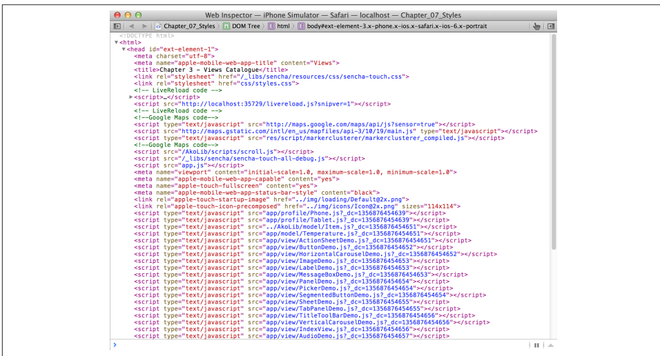
Figure 1-3. HTML5 meta tags generated by Sencha Touch 2
