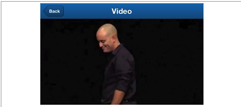
Figure 3-22. Embedded video
