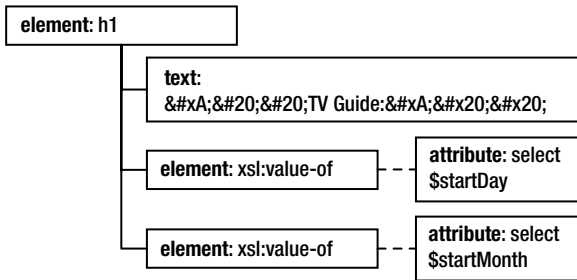
Figure 8-8. Node tree created from XSLT code after whitespace stripping
