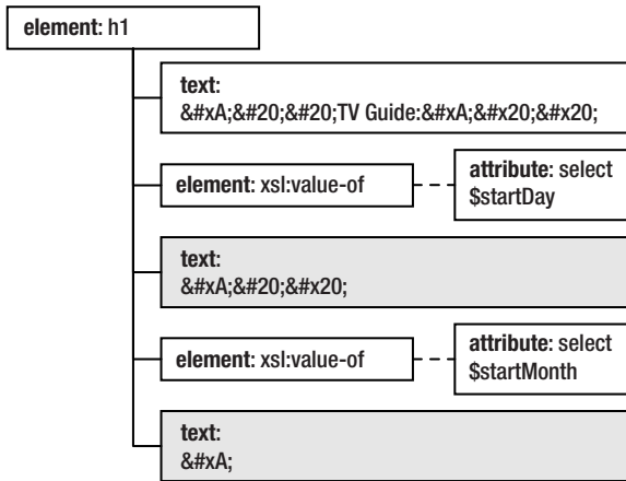
Figure 8-7. Node tree created from XSLT code
