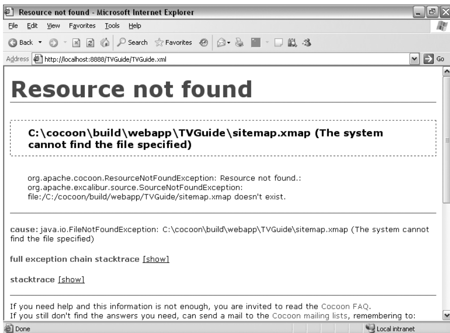
Figure 15-7. Error when trying to view TVGuide.xml without configuring Cocoon www.it-ebooks.info
