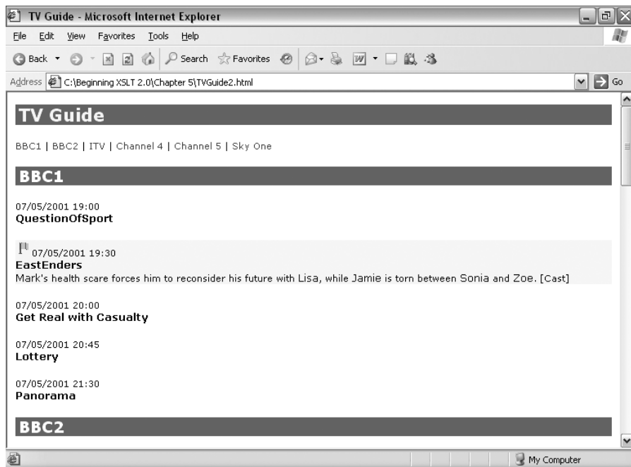
Figure 5-2. Viewing TVGuide2.html in Internet Explorer www.it-ebooks.info
