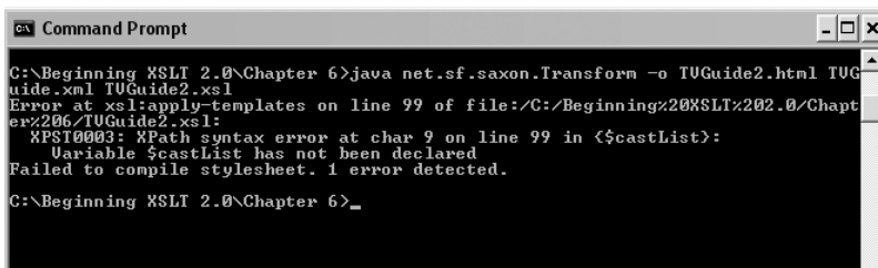
Figure 6-2. Error message when transforming TVGuide.xml with TVGuide2.xsl
