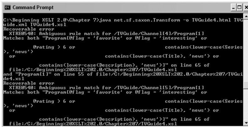
Figure 7-10. Saxon warning of ambiguous template match
