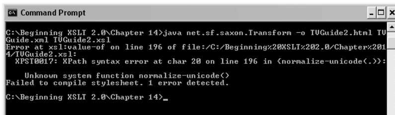
Figure 14-1. Error message due to unsupported function in Saxon 8.4
