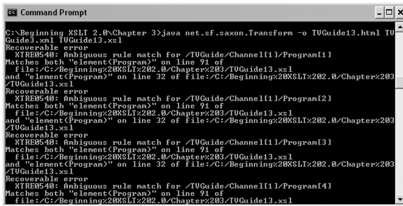
Figure 3-11. Recoverable error messages from multiple template matches in Saxon
