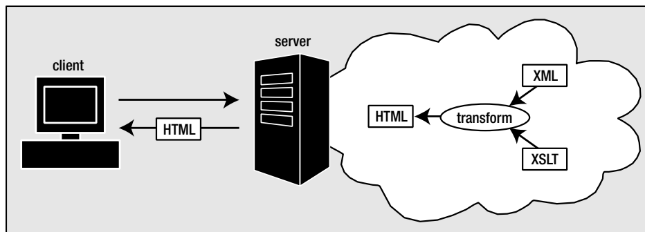
Figure 15-1. Server-side transformations
