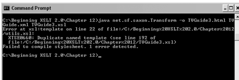
Figure 12-3. Error due to duplicate named template
