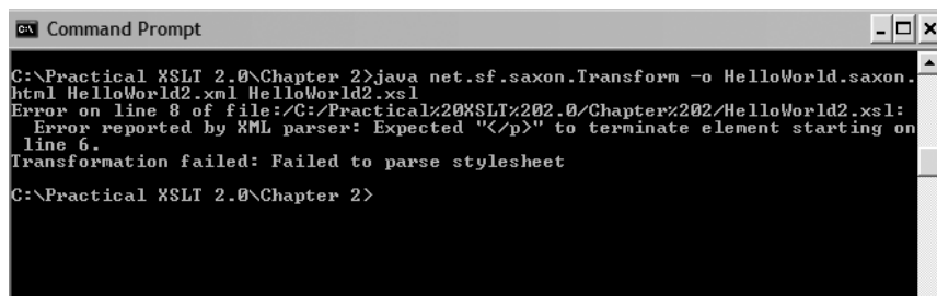
Figure 2-6. Error with Saxon from non-well-formed stylesheet
