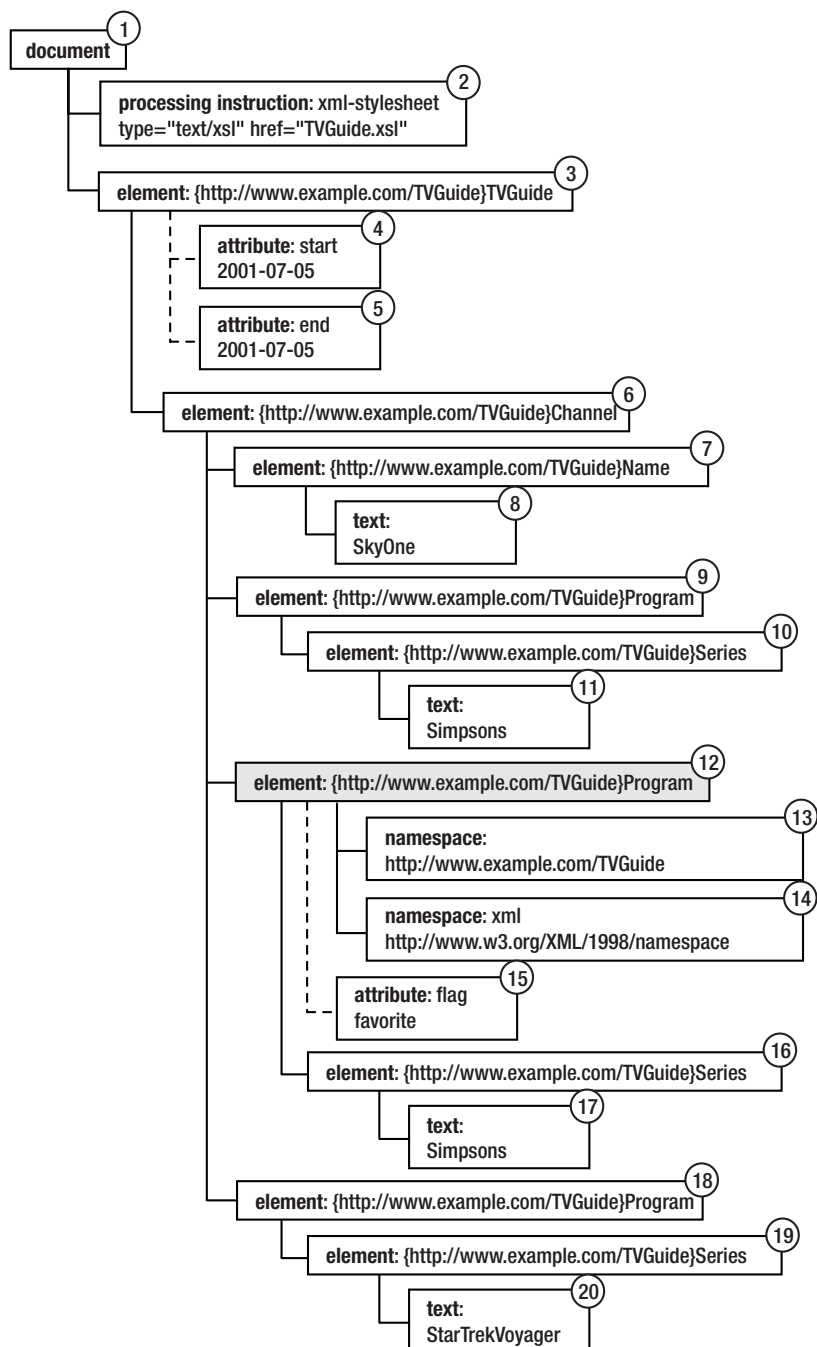
Figure 7-13. Example node tree
