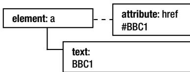
Figure 8-5. Text node generated using <xsl:value-of>
