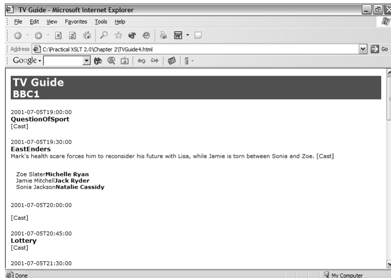
Figure 2-16. Viewing cast in TVGuide4.html in Internet Explorer
