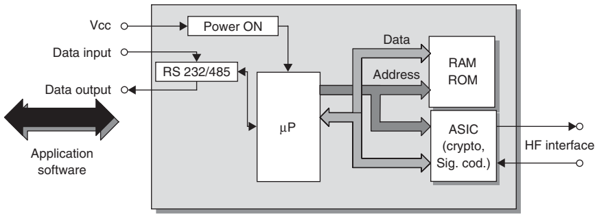
Figure 11.9 Block diagram of the control unit of a reader. There is a serial interface for communication with the higher application software
