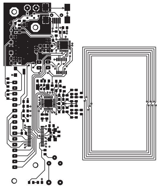
Figure 14.12 Layout of the reader board (reproduced by permission of Elektor, http://www.elektor.de )
