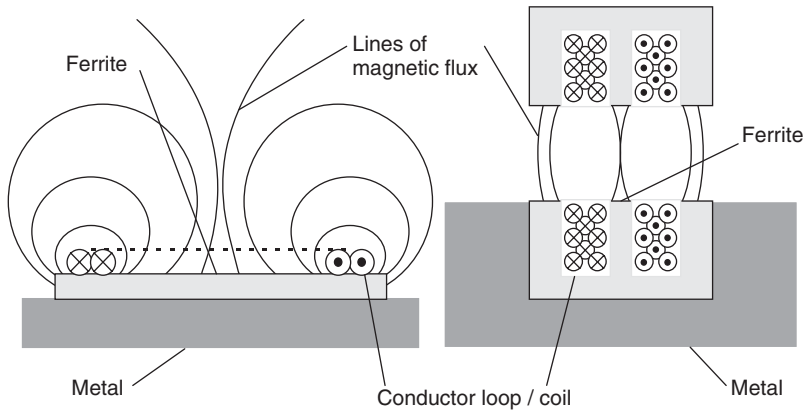
Figure 4.54 Reader antenna (left) and gas bottle transponder in a U-shaped core with read head (right) can be mounted directly upon or within metal surfaces using ferrite shielding
