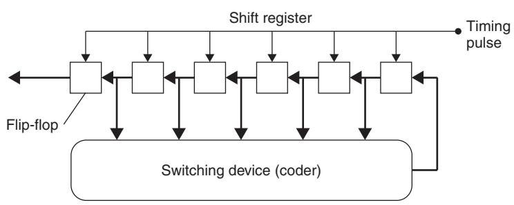
Figure 8.19 Basic circuit of a pseudorandom generator incorporating a linear feedback shift register (LFSR)
