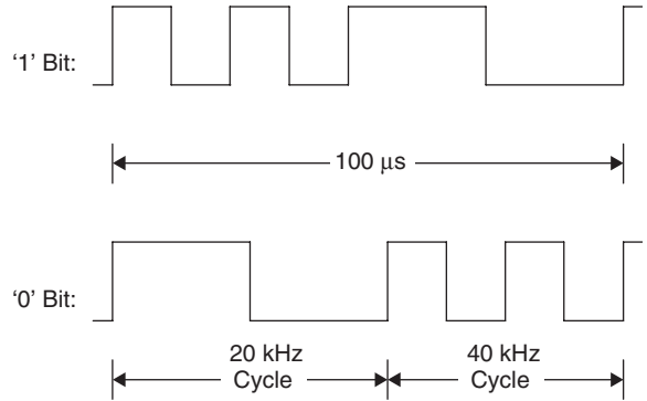
Figure 9.40 Coding of data bits using the modified FSK subcarrier procedure
