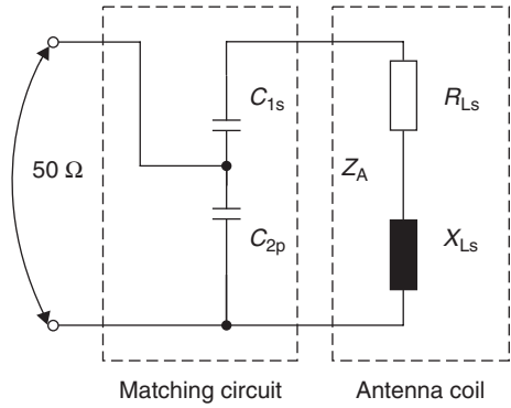
Figure 11.22 Simple matching circuit for an antenna coil
