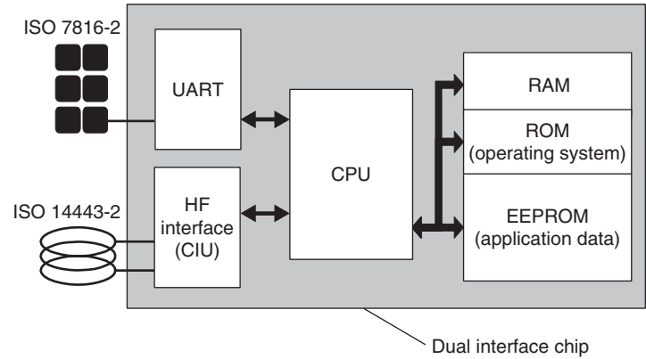
Figure 10.27 Block diagram of a dual interface card. Both smart card interfaces can be addressed independently of one another
