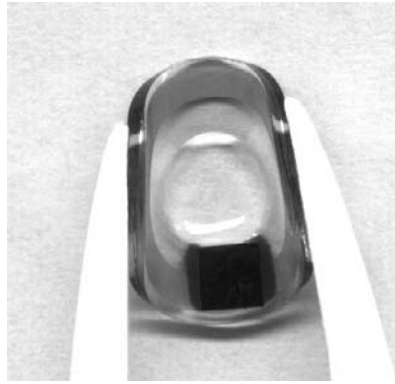
Figure 13.62 Cast transponder unit deformed by a pair of tweezers (reproduced by permission of IWE1, RWTH Aachen, D-52074 Aachen)
