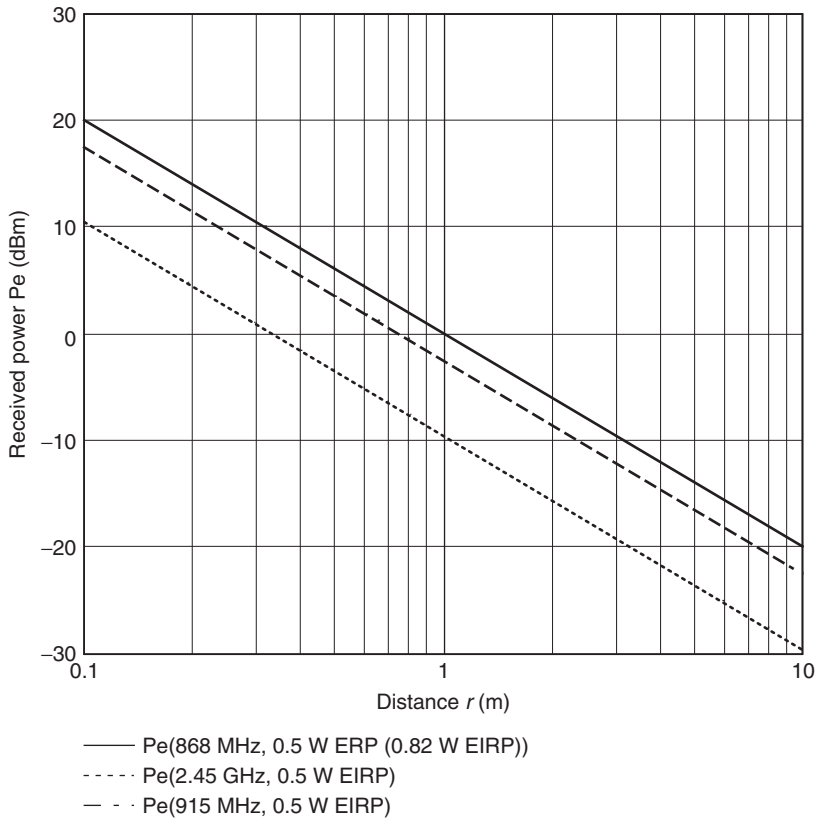
Figure 4.78 The maximum power P_e(0 \text{ dBm} = 1 \text{ mW}) available for the operation of the transponder, in the case of power matching at the distance r , using a dipole antenna at the transponder
