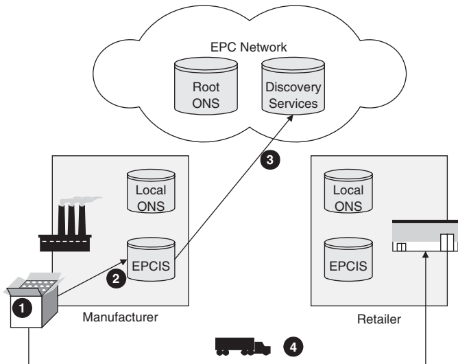
Figure 9.48 The life cycle of an EPC starts with attaching the transponder(1) to the object
