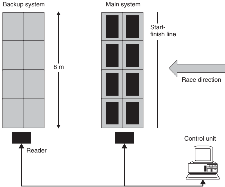
Figure 13.52 A control station consists of a main system and a reserve system. The systems are made up of arrays of antennas in mats
