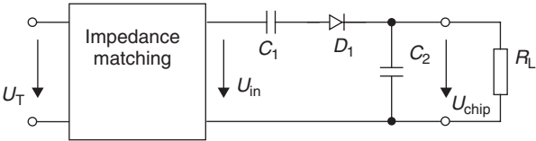
(a) Practical circuit: voltage doubler with impedance matching
