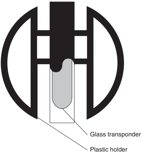
Figure 13.50 The transponder consists of a glass transponder, which is injected into a plastic housing that is shaped according to its function. The diagram shows the partially cut away plastic housing
