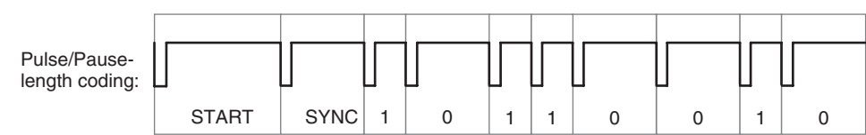
Figure 6.3 Possible signal path in pulse-pause coding
