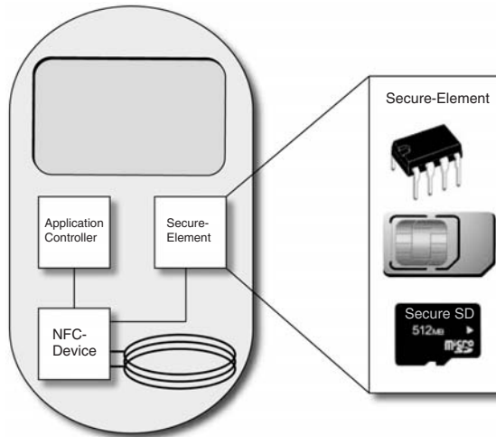
Figure 11.31 An NFC secure element can be designed as a directly soldered smart card chip, a secure memory chip or as the SIM card of a mobile phone
