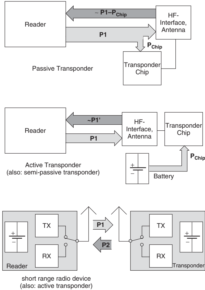
Figure 2.17 Comparison between passive and active transponders
