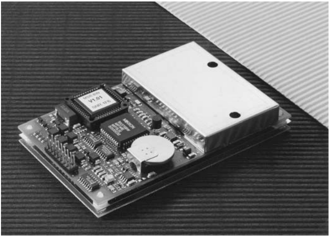
Figure 11.3 Example of a reader. The two functional blocks, RF interface and control system, can be clearly differentiated (MIFARE® reader, reproduced by permission of Philips Electronics N.V)
