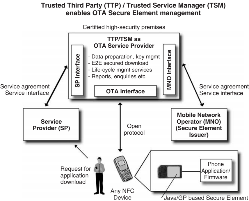
Figure 13.14 Administration of the secure element of an NFC-enabled phone via OTA service (Yliutinen, 2007; figure Venyon)
