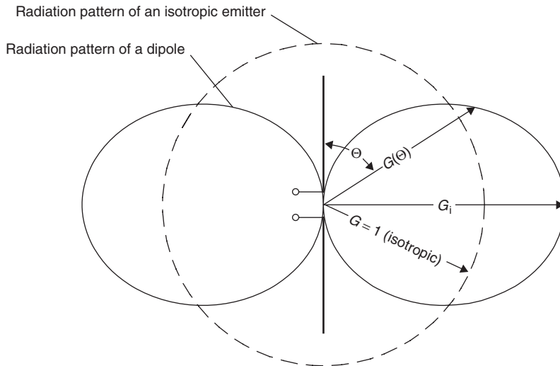
Figure 4.64 Radiation pattern of a dipole antenna in comparison to the radiation pattern of an isotropic emitter
