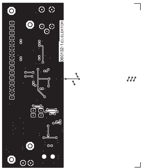
Figure 14.13 Back view of the layout of the reader board (reproduced by permission of Elektor, http://www.elektor.de )
