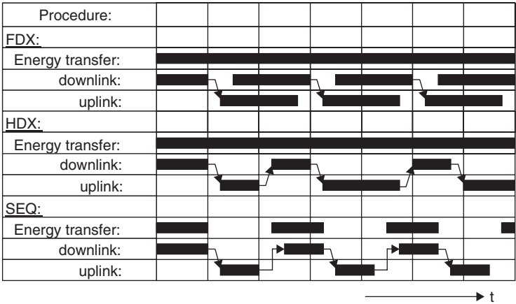
Figure 3.12 Representation of full-duplex, half-duplex and sequential systems over time. Data transfer from the reader to the transponder is termed down-link, while data transfer from the transponder to the reader is termed up-link
