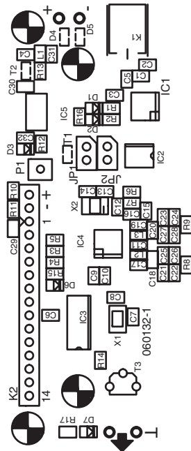
Figure 14.14 Component diagram of the reader board (reproduced by permission of Elektor, http://www.elektor.de )
