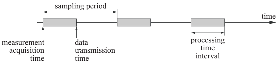
Figure 11.1. Time related quantities associated with a sensor
