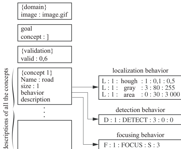
Figure 10.6. The knowledge base
