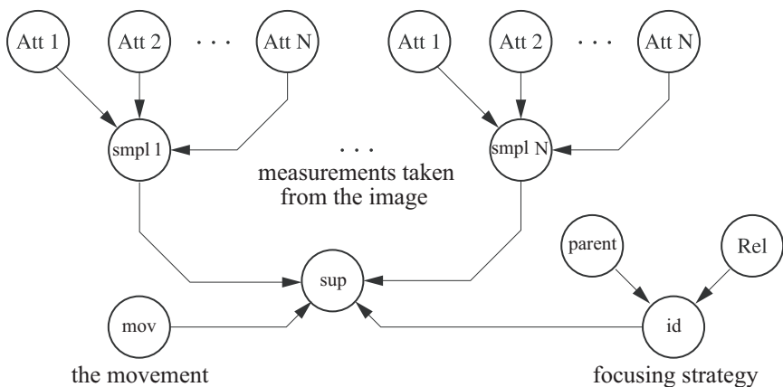
Figure 10.8. Description of the Bayesian network used for calculating the confidence of a support. This confidence depends on the confidence obtained for each sample, on focusing relations and on the movement
