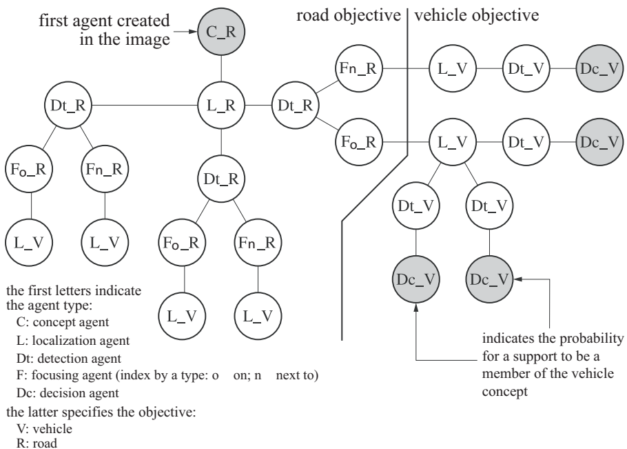
Figure 10.15. Agent graph related to vehicle detection when two focusing rules are specified. The type of the initial objective is “road”. The system searches for vehicles “on” roads or “next to” roads
