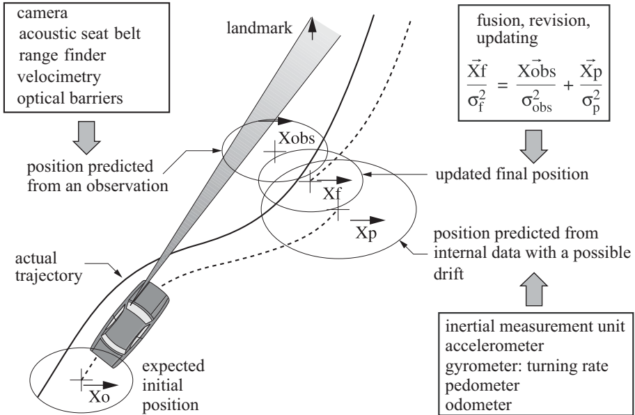
Figure 2.1. Navigation and localization
