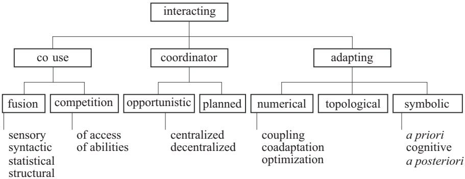
Figure 2.6. Taxonomy of the different interaction mechanisms
