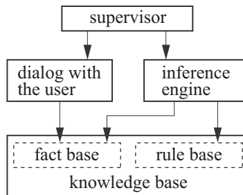
Figure 5.1. The major functions of a KBS
