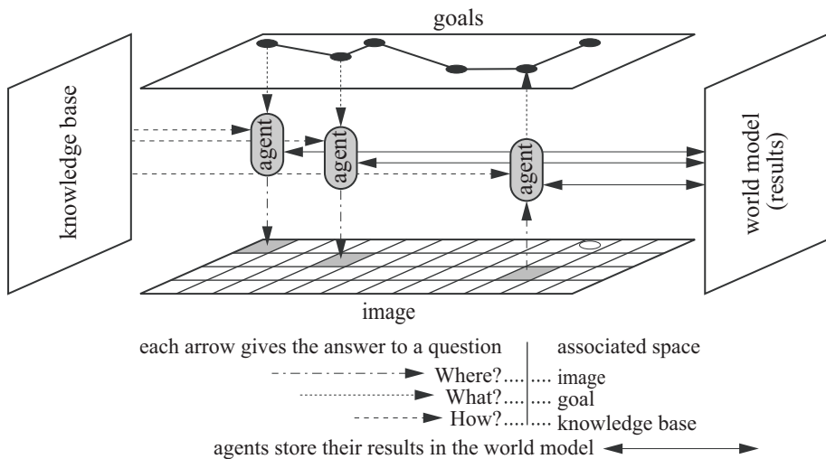
Figure 10.2. General view of the multi-agent system. Each agent is embedded in a three-dimensional space comprised of the image space, the goal space and the method space. The agents are situated in the image, with a precise goal. They work locally using the data from the knowledge base to produce partial results that will be stored in the world model. This world model is then shared among all of the agents
