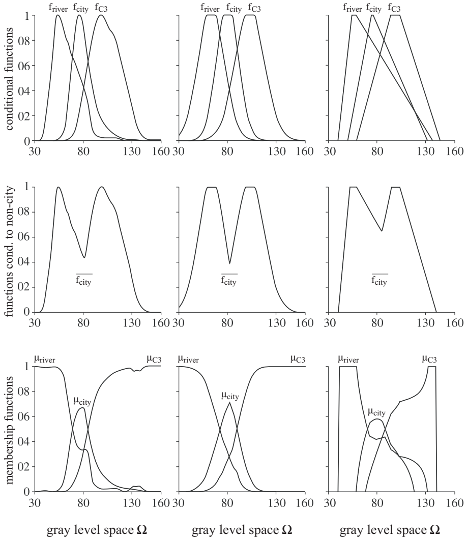
Figure 8.13. Top: the functions f_i^j conditional to the classes that were estimated under supervision on the learning areas of the images; in the center, the functions \overline{f_{city}^j} estimated from the maxima of the functions f_{river}^j and f_{C3}^j ; bottom: the membership functions \mu_i^j . Left: estimation from the normalized and smoothed histograms; center, estimation from the truncated Gaussian functions; right: estimation of the functions from the linear L-R functions
