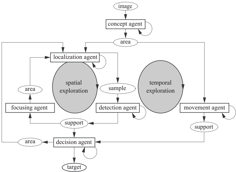
Figure 10.4. The intra-image control diagram is comprised of two analysis cycles: a spatial exploration cycle and a temporal exploration cycle in order to associate additional information in the context of information fusion
