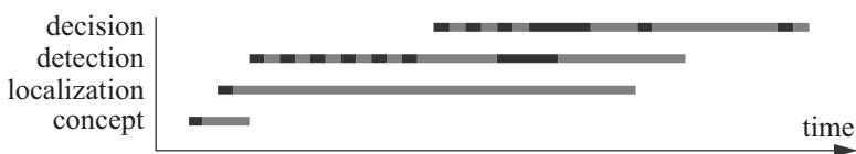
Figure 10.13. Distribution of the computation times among the different agents: black indicates the activation of an agent and gray indicates that it is running
