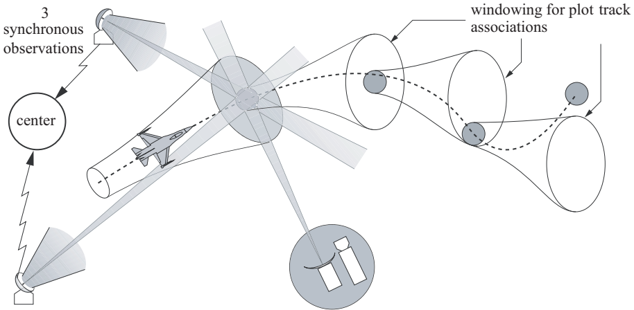
Figure 2.2. Multi-sensor tracking of a maneuvering target
