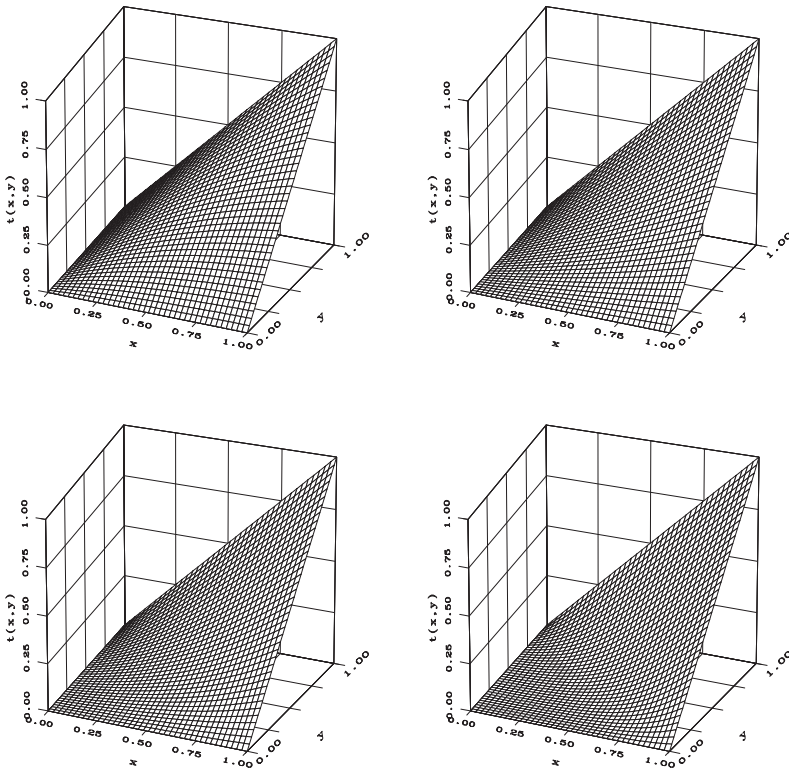
Figure 8.6. Four examples of Frank t-norms. First line: s = 0.1 and s = 2 . Second line: s = 10 and s = 1,000
