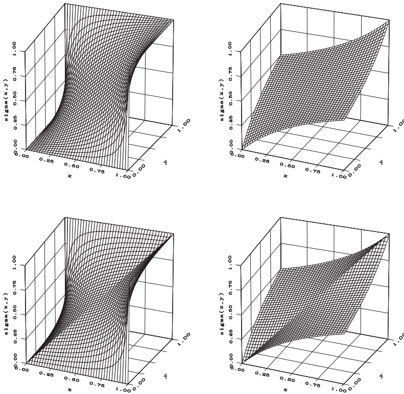
Figure 8.9. Four examples of symmetric sums. First line: \sigma_0 and \sigma_+ . Second line: \sigma_{\min} and \sigma_{\max}
