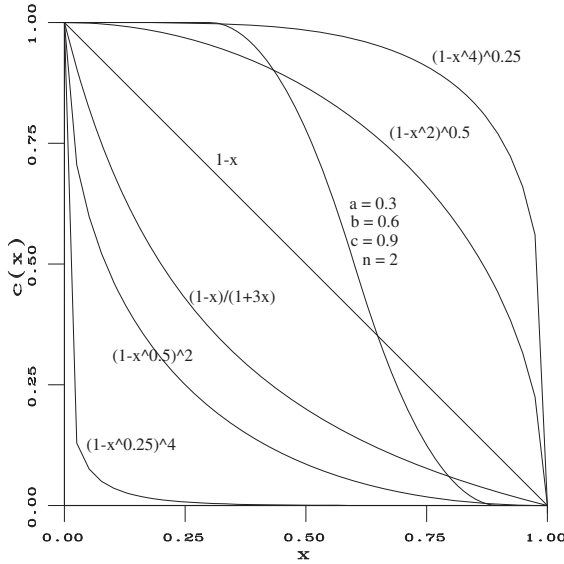
Figure 8.2. A few examples of fuzzy complementation
