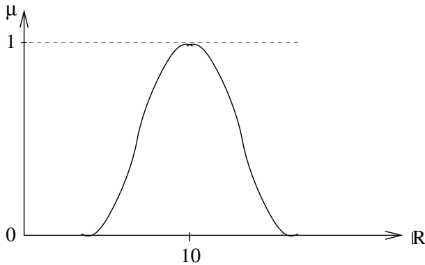
Figure 8.1. Fuzzy number representing “roughly 10”
