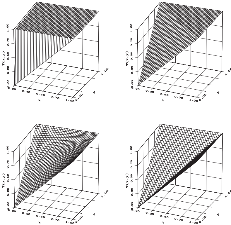
Figure 8.4. Four examples of t-conorms. First line: T_0 (highest t-conorm) and Lukasiewicz t-conorm. Second line: algebraic sum and maximum (smallest t-conorm)
