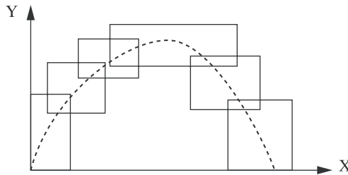
Figure 8.12. An example of a function's graph
