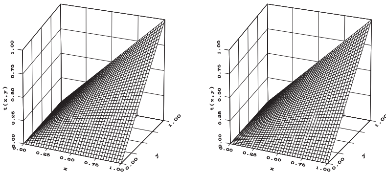
Figure 8.5. Two examples of Hamacher t-norms, for \gamma = 0 (left) and \gamma = 0.4 (right)
