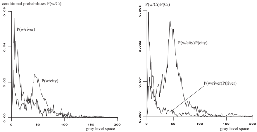
Figure 6.2. Left: conditional probabilities of the cities and rivers in the texture image on XS2. Right: probabilities conditional to the two classes multiplied by their a priori probability P(city) = 11\% and P(river) = 2\%
