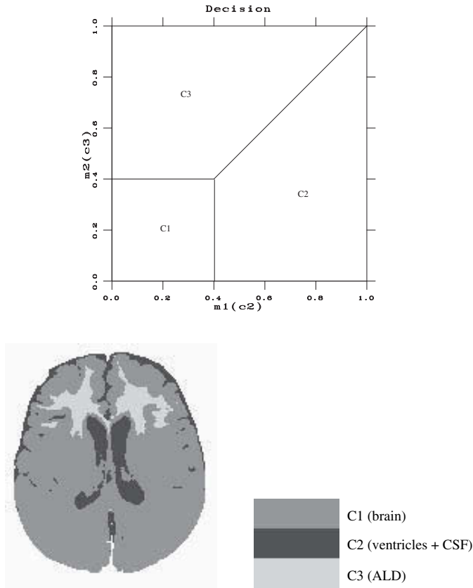
Figure 7.3. The different decision zones depending on the values of m_1(C_2) and m_2(C_3) and the decision image, by taking the maximum belief over the simple hypotheses
