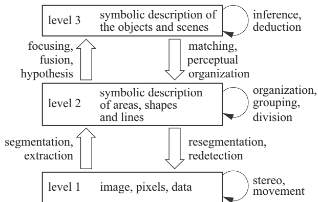
Figure 5.2. Diagram explaining how a KBS works. This representation is based on VISION [HAN 88]
