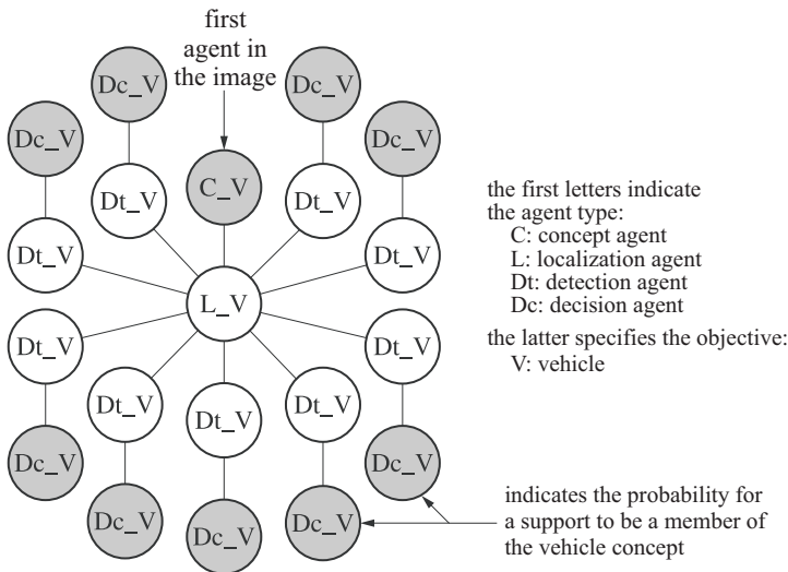
Figure 10.11. Agent graph generated for detecting vehicles using the direct strategy; four types of agents are implemented: the Concept, Localization, Detection and Decision agents. All these agents have the same objective, namely the vehicle concept. In this example, nine vehicle-type supports are detected
