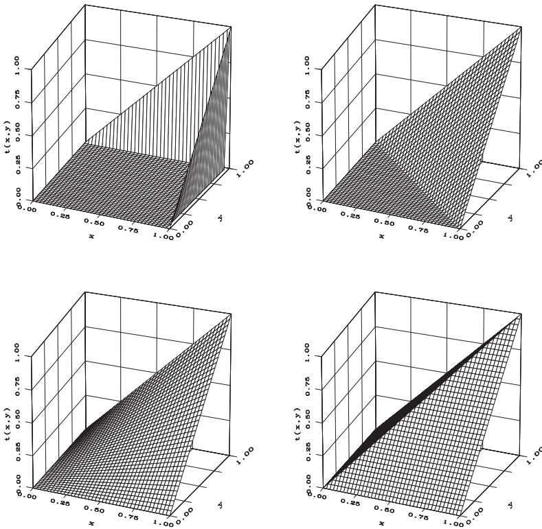
Figure 8.3. Four examples of t-norms. First line: t_0 (lowest t-norm) Lukasiewicz t-norm. Second line: product and minimum (highest t-norm)
