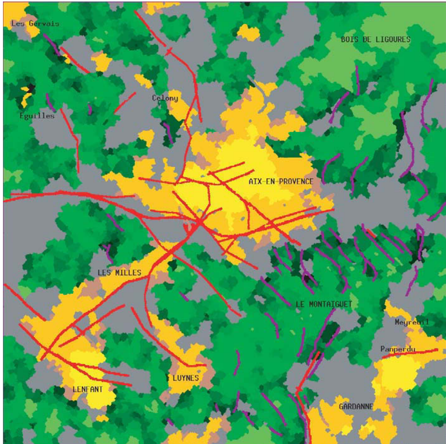
Figure 9.4. Result obtained from the image in Figure 9.2 by fusing detectors of different structures. The lighter areas represent urban areas. The dark lines correspond to roads, the lighter lines to slopes. The darkest areas (with different shades) are forest areas. Finally, the medium gray areas correspond to the empty set, i.e. unrecognized areas
