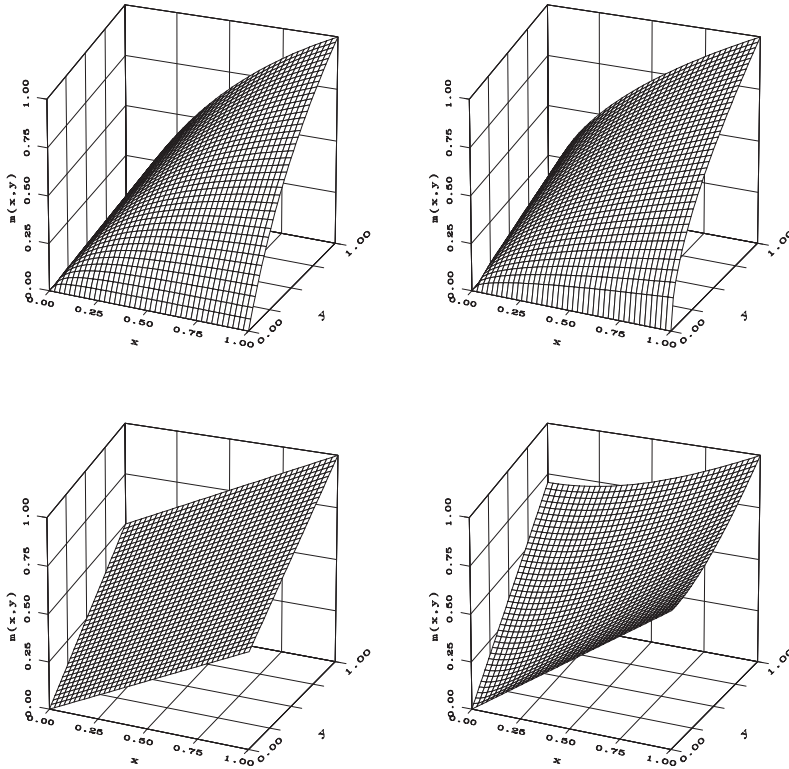
Figure 8.8. Four examples of mean operators. First line: harmonic and geometric means. Second line: arithmetic and quadratic means
