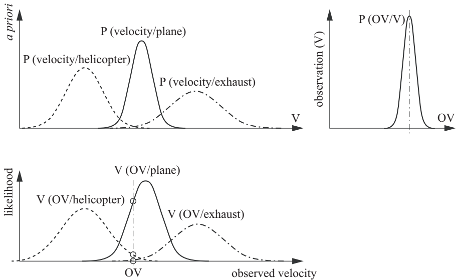
Figure 2.3. Discriminating among several hypotheses
