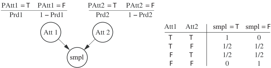
Figure 10.9. The computation of the confidence in a sample is conducted using a Bayesian network. In this example, two methods are used to characterize a sample
