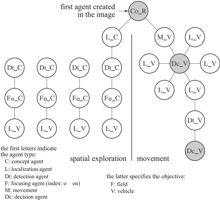
Figure 10.19. Agent graph in the presence of movement. It represents the population of agents implemented to find the vehicles, knowing that the spatial exploration is conducted along with the search for movement information
