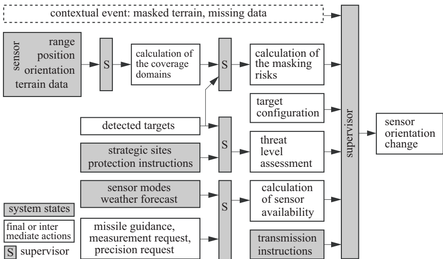
Figure 2.5. Controlling the orientation of sensors in the case of masked terrain
