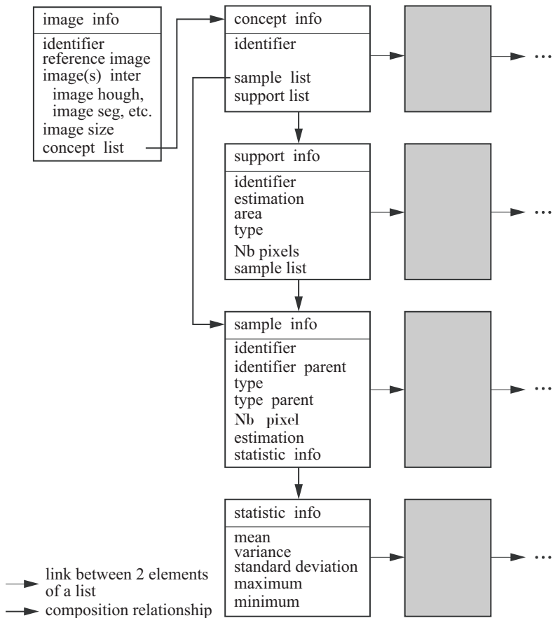
Figure 10.7. Structure of the world model: for each image, we have access to the list of concepts, of supports and of the associated statistical parameters. A concept is comprised of several supports, which are themselves comprised of samples characterized by a list of statistical information
