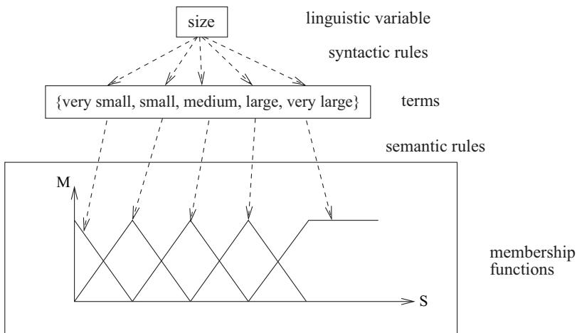
Figure 8.11. Illustration of the linguistic variable "size", its terms and the associated fuzzy sets. The arrows drawn from the linguistic variable to the term set represent syntactic rules. The second set of arrows represents the semantic rules and translates the terms into membership functions
