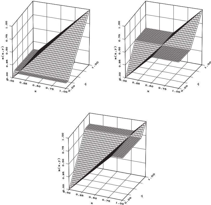
Figure 8.7. Three examples of medians, for \alpha equal to 0.1, 0.5 and 0.8, respectively
