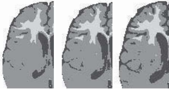
Figure 7.4. Decision by maximum belief based on simple hypotheses, for an increasing weight on m_2(C_3) and m_1(C_2)
