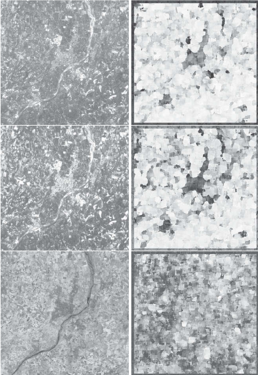
Figure 6.1. SPOT satellite images in XS multi-band spectral mode with a size of 512 \times 512 pixels and a 1-B level of pre-processing in vertical viewing (the area of Vignola, near Modena, in Italy) © Spot Image. From top to bottom, the green (XS1), red (XS2) and near infrared (XS3) channels. Left: original SPOT images. Right: images of temperature parameters of a Gaussian Markovian field on the three SPOT channels (texture images)
