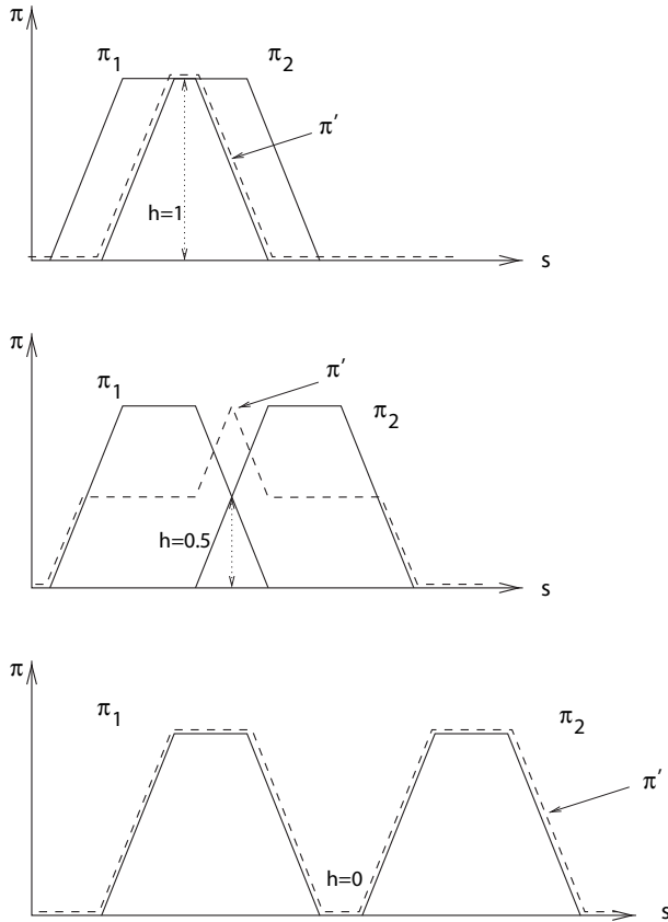
Figure 8.10. Example of adaptive operators varying from the min to the max when the conflict between two distributions increases
