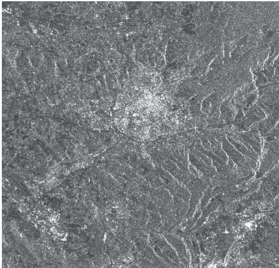
Figure 9.2. ERS-1 radar image of Aix-en-Provence region
