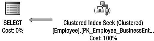
Figure 8-4. Every set of arguments passed to the stored procedure results in the same execution plan.
