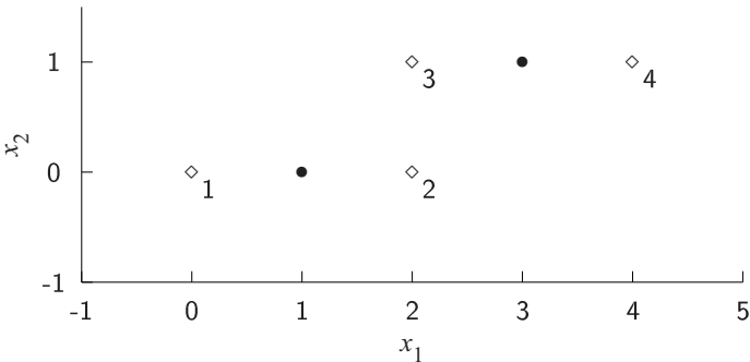
Figure 11.9 Data to illustrate the k -means local optimum.
