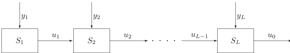
Figure 8.7 Sensors arranged in a serial configuration.
