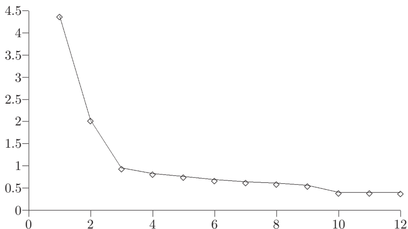
Figure 10.9 Eigenvalue spectrum: a plot of the ordered eigenvalues against eigenvalue number, with an ‘elbow’ at the third eigenvalue.
