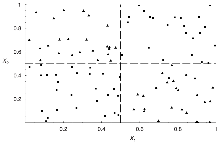
Figure 10.4 Relevance in context. The distribution of X_1 and X_2 are independent of the class variable ( X_1 \perp Y , X_2 \perp Y ), but jointly, the distribution depends on class ( \{X_1, X_2\} \perp / Y ).
