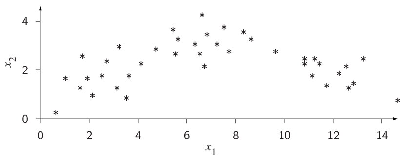
Figure 11.3 Illustration of chaining with the single-link method.
