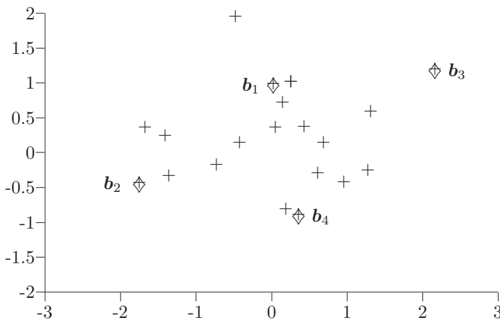
Figure 4.4 Selection of base prototypes (◊) from the dataset (+).
