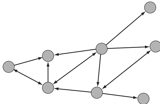
Figure 12.2 A directed graph in which some of the edges are unidirectional and some bidirectional.
