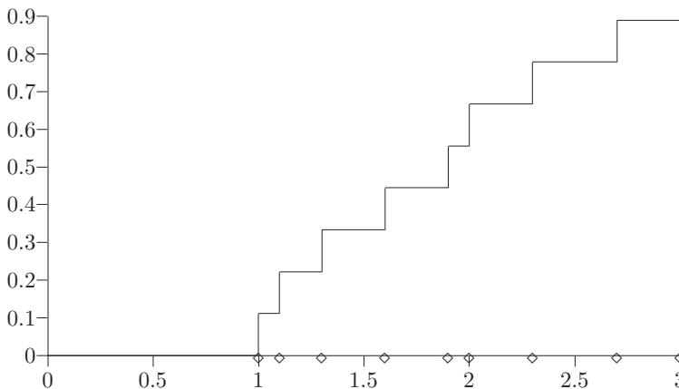
Figure 4.25 Cumulative distribution.
