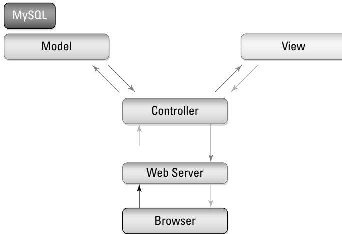
Figure 10-1: MVC pattern workflow.
