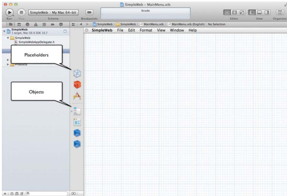
Figure 33-6. Your first look at MainMenu.xib in Xcode
