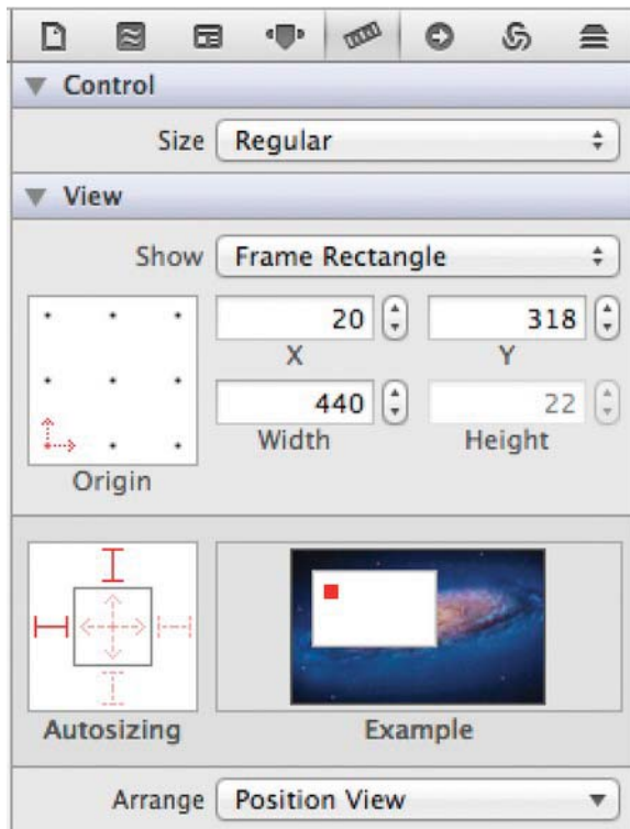
Figure 33-12. You can adjust the sizing properties of your object using the Size inspector.
