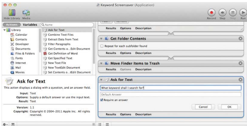
Figure 31–11. The Ask for Text action in your workflow
