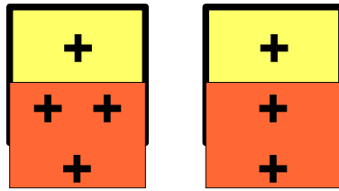
Figure C.6 UNION ALL versus UNION. The thick box is M and the thinner box is N. The first UNION ALL shared regions are duplicated; in UNION only one of the shared regions is kept, resulting in a distinct set.
