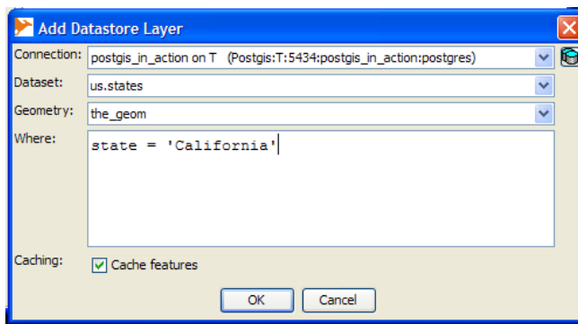
Figure 12.5 Datastore Layer setup in OpenJUMP
