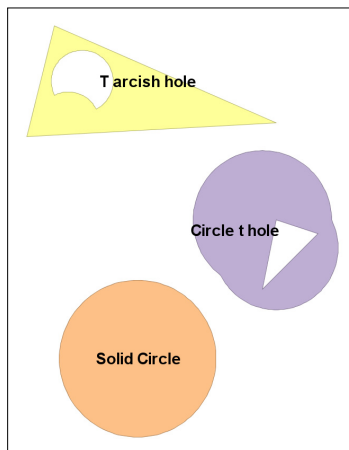
Figure 2.15 Curvepolygons generated from the code in listing 2.5
