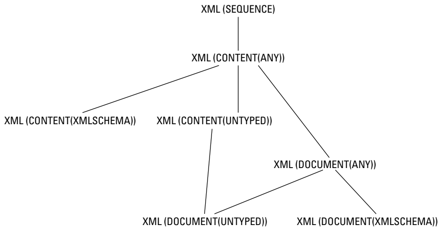
Figure 2-1: Relationships of the XML subtypes.
