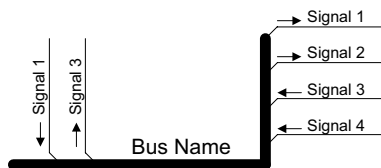
Figure 7-38. A bus with vertical and horizontal segments
