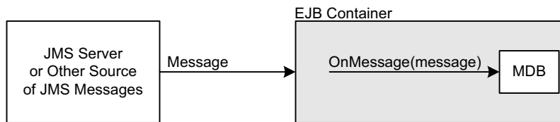
Figure 5-10. How messages are delivered to a Java message-driven bean
