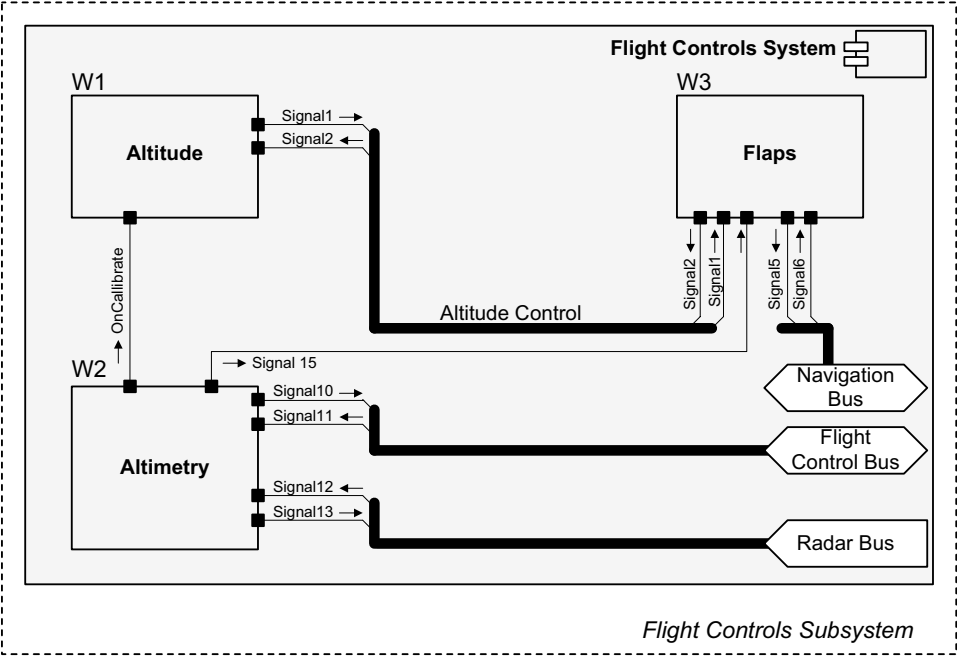
Figure 7-68. A more detailed view of a single subsystem
