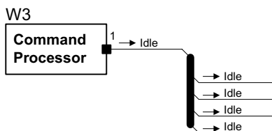
Figure 7-42. Using a bus to group outgoing signals from the same pin
