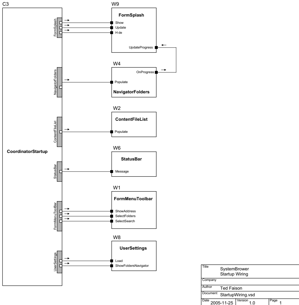
Figure 11-12. The wiring diagram of the startup system
