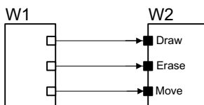
Figure 7-31. Omitting signal names on short wires
