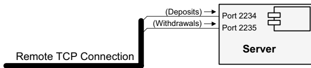
Figure 7-49. Input pins labeled to indicate their TCP socket port
