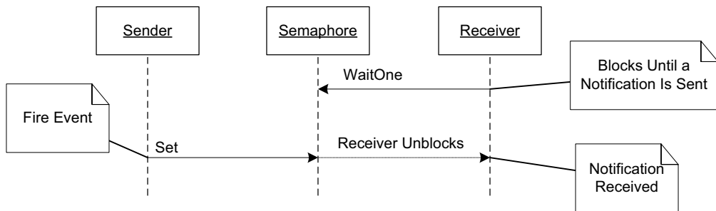
Figure 8-18. Using a binary semaphore to deliver notifications
