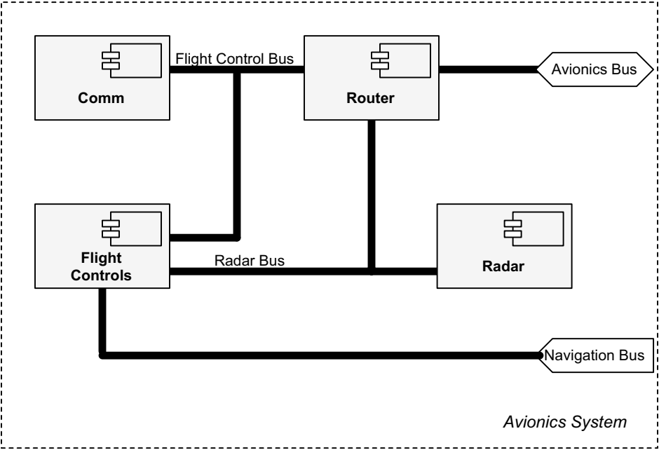
Figure 7-67. The top-level view of a single system
