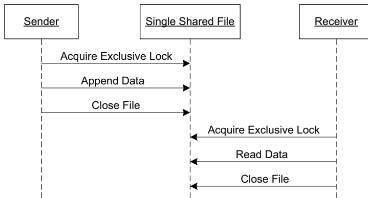
Figure 3-5. Using a single file to send notifications
