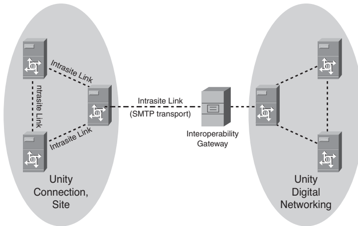
Figure 10-7 Unity to Unity Connection Networking
