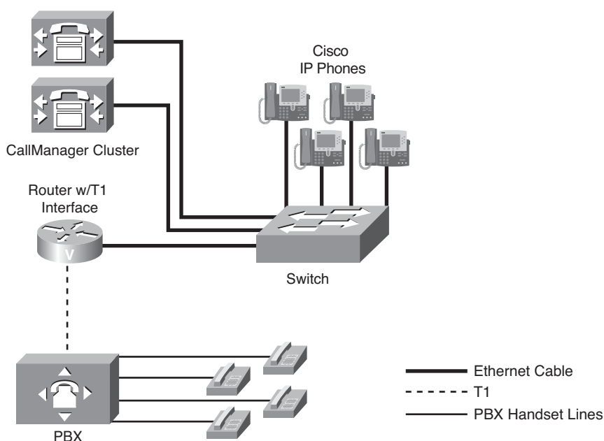
Figure 1-2 Communications Manager-to-PBX Integration
