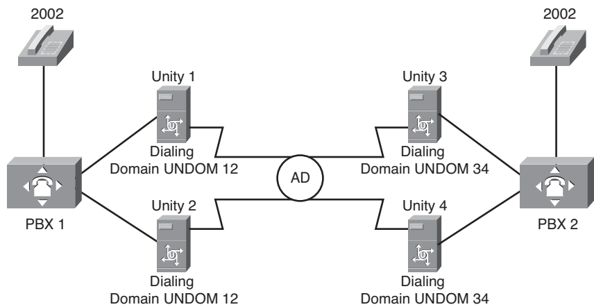
Figure 10-5 Digital Networking Overview
