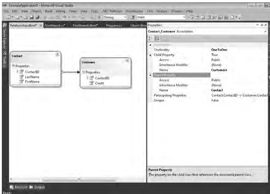
FIGURE 7-13 Association properties of a one-to-one relationship.
