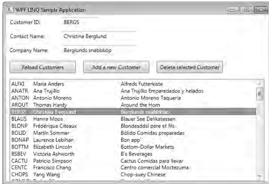
FIGURE 19-11 A XAML window with complex (list and detail) data binding.
