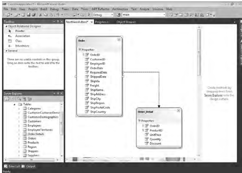
FIGURE 7-4 Two entities created from a server connection.
