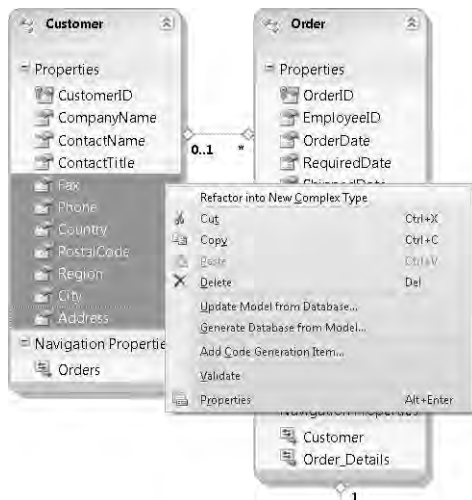
FIGURE 8-8 Part of the Entity Data Model Designer interface, used to refactor a set of properties into a complex type.
