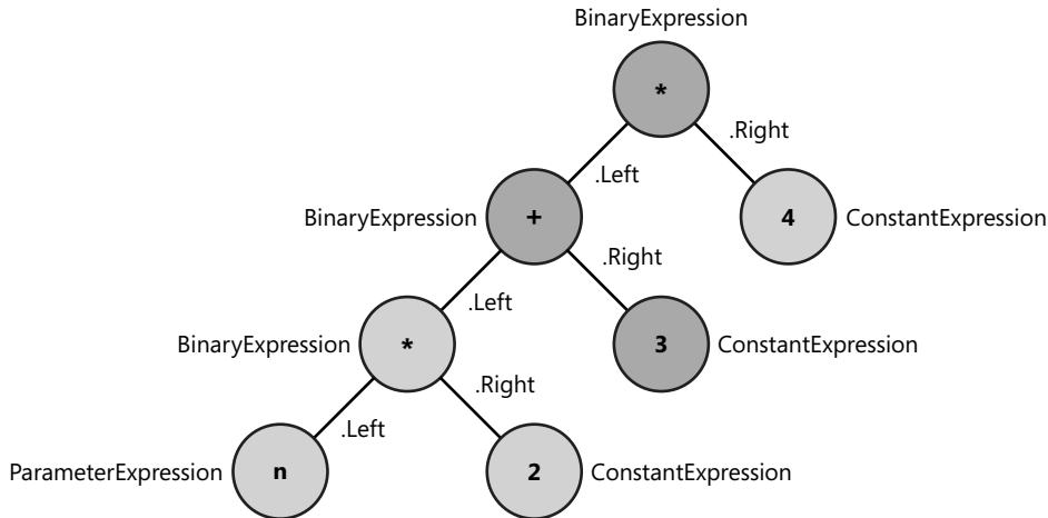
FIGURE 14-7 Dark gray nodes are new; light gray nodes are the same as in the older tree.
