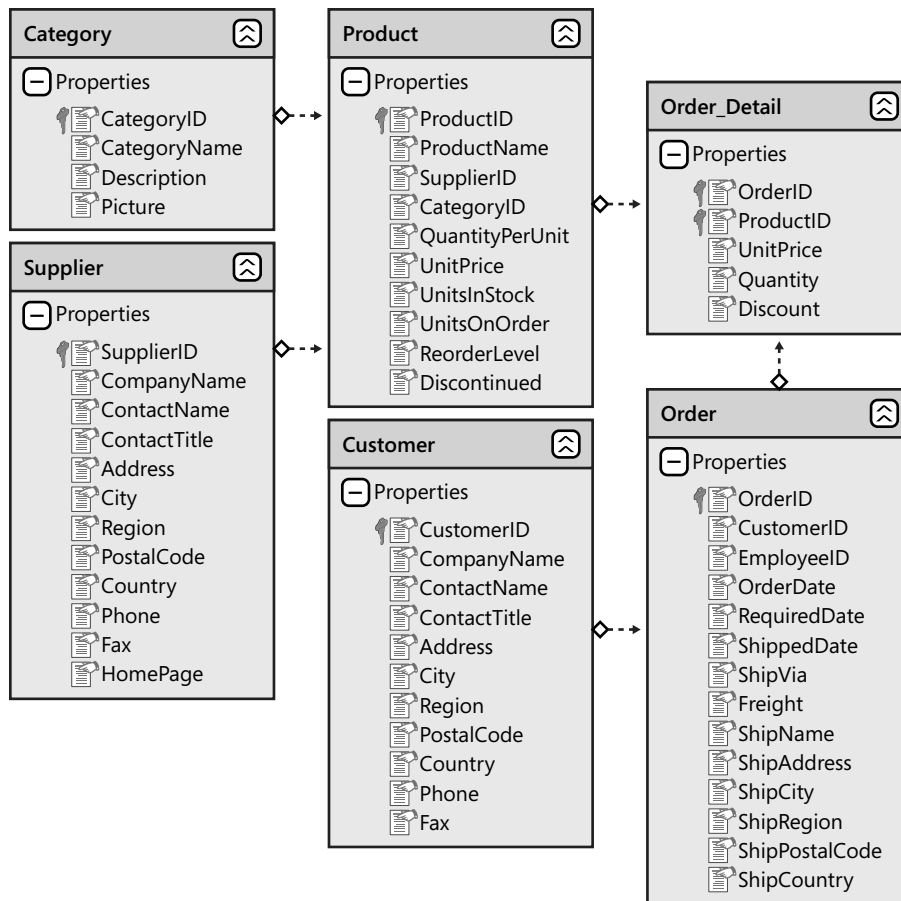
FIGURE 19-1 The LINQ to SQL Database Model schema used in the samples of this chapter.
