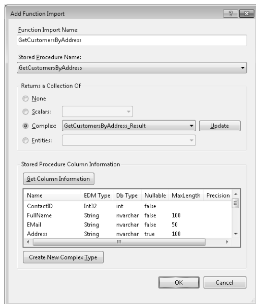
FIGURE 8-12 The dialog box used to import a stored procedure as a function into the conceptual model.
