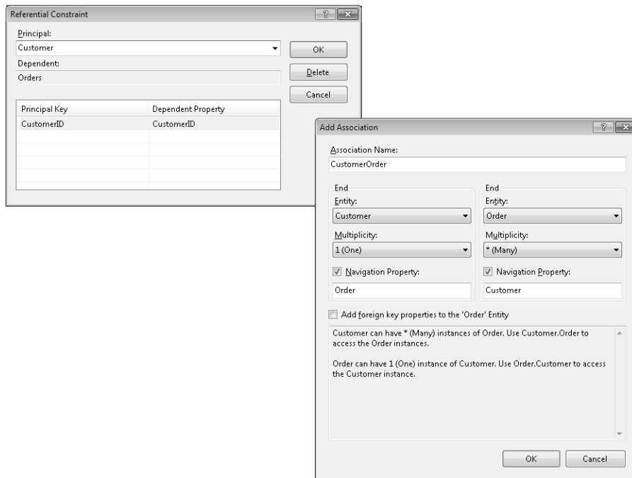
FIGURE 8-7 The Entity Data Model Designer dialog boxes for adding or managing the referential constraint of a Foreign Key Association (on the left) or an Independent Association (on the right).
