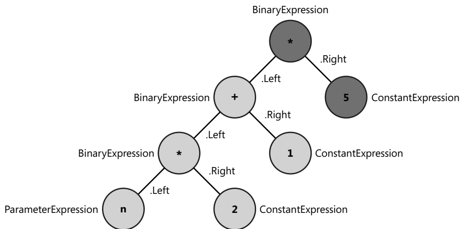
FIGURE 14-6 Dark gray nodes are new; light gray nodes are the same as in the older tree.
