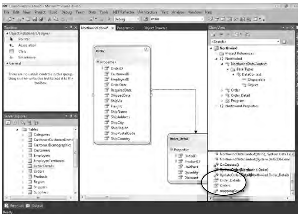
FIGURE 7-5 FPlural names for Table<T> properties in a DataContext -derived class.
