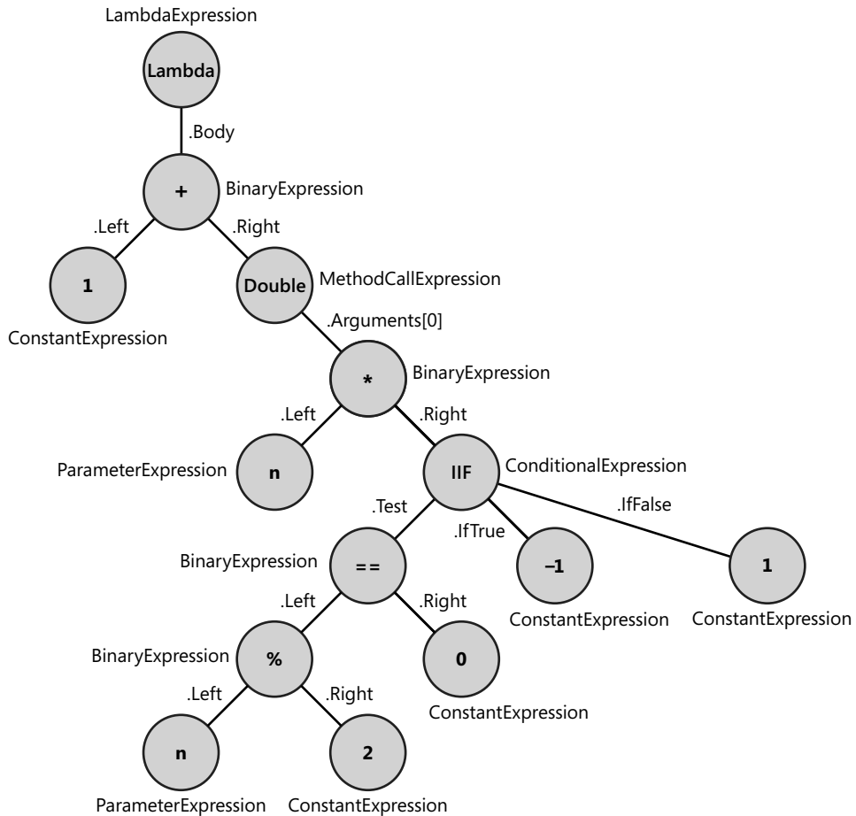
FIGURE 14-9 Complex expression tree.
