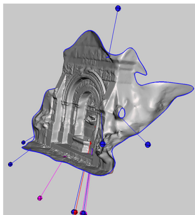
Figure 9-28. Model shown with spheres indicating mesh problems
