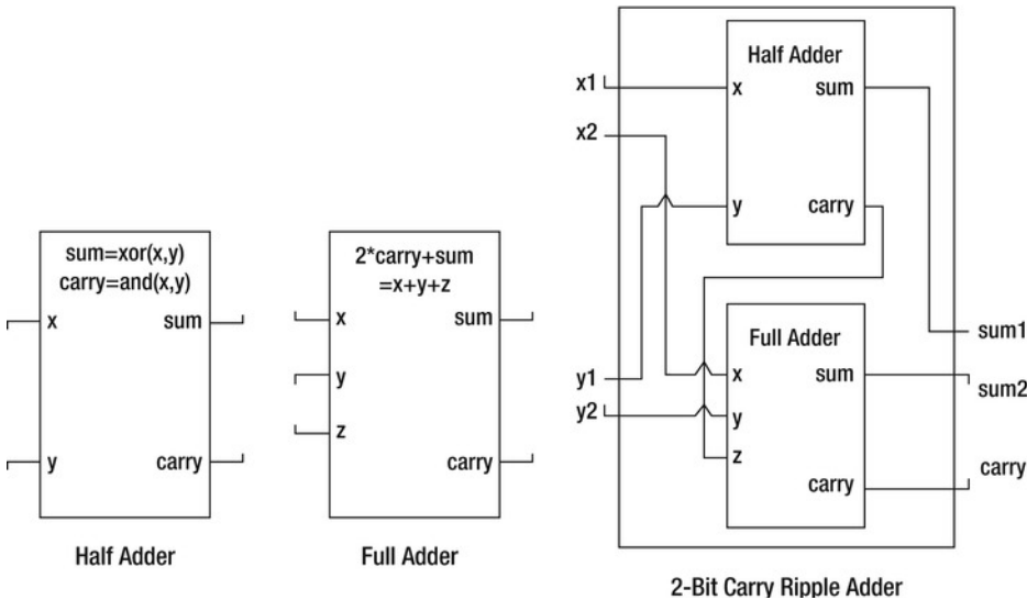
Figure 12-1. Three simple hardware circuits
