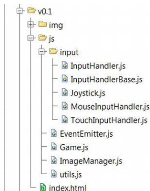
Figure 7-3. Initial structure of the project
