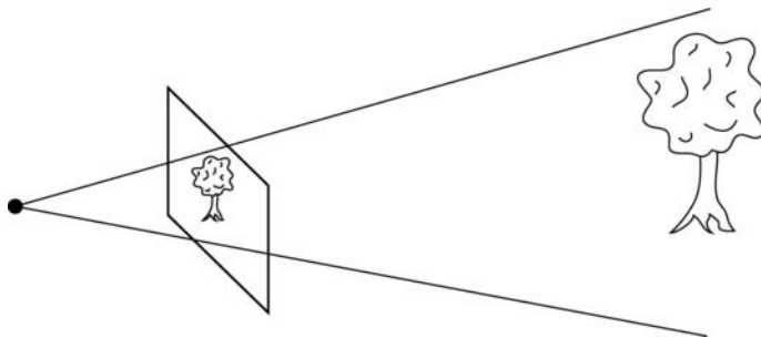
Figure 8-3. In computer graphics, there are no lenses. That's why the plain that “captures” the scene projection is placed in front of the focal point. Still the rules for the field of view remain the same: the more you see, the smaller individual objects become.
