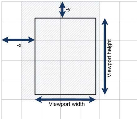
Figure 6-7. Draw only the tiles that are currently visible in the viewport. Stroked out tiles are the ones that we will draw.
