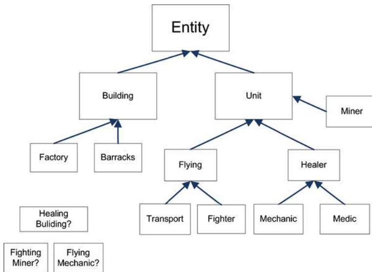
Figure 14-4. A typical problem with inheritance of game entities
