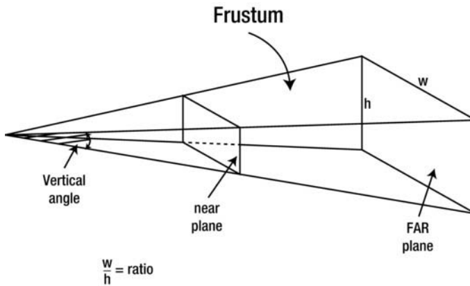
Figure 8-18. Defining scene bounds with perspective
