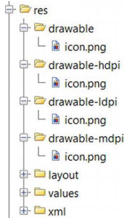
Figure 15-6. Icons of different sizes are placed into the appropriate folders
