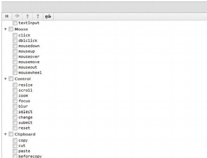
Figure 5-1. A fragment of the long list of browser events
