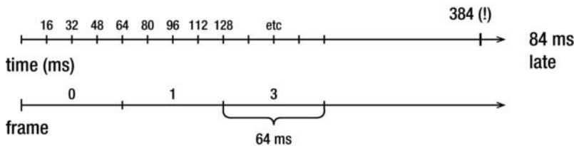
Figure 4-11. In the real world, timers are inaccurate and animations are running late.
