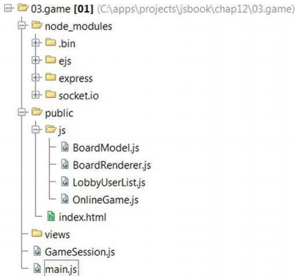
Figure 12-3. The structure of the project
