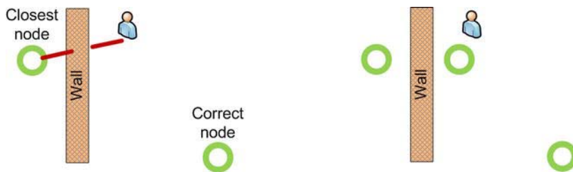
Figure 13-13. On the left, the problem with a naïve pathfinding graph: due to the mistake of the level designer, the character attempts to move through the wall to reach the node. The corrected version is on the right.
