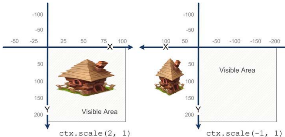
Figure 2-29. Scaling. The left image is scaled on the x axis; the image on the right shows a flipped scene.
