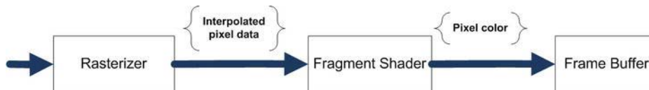
Figure 9-3. In the second part of rendering process, data received from the vertex shader is interpolated and passed to the fragment shader. The fragment shader outputs the pixel color.
