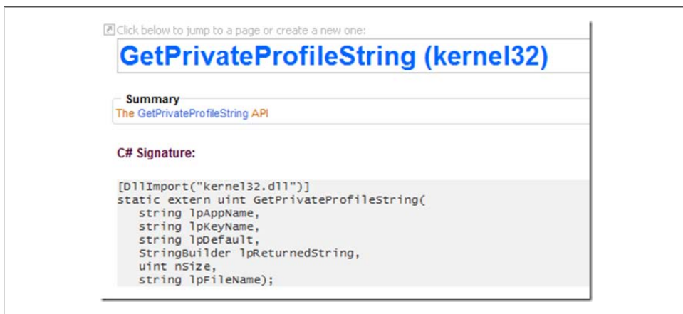
Figure 17-2. The Windows API signature for GetPrivateProfileString
