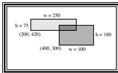
Figure 8.10 Intersecting rectangles
