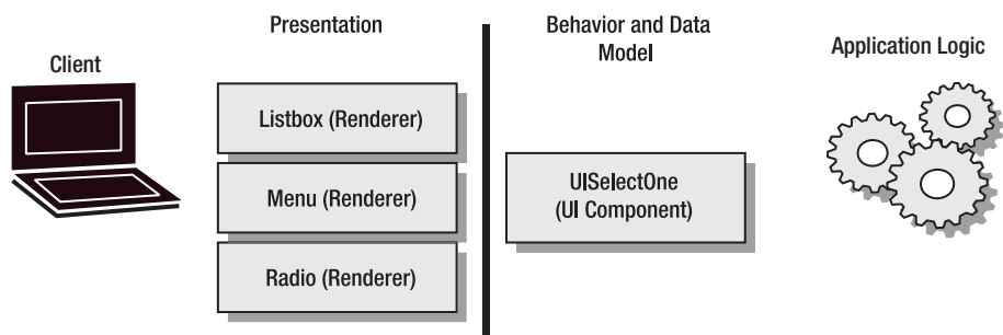
Figure 1-6. UISelectOne and its renderers
