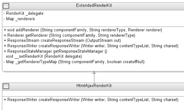
Figure 6-8. Class diagram of the HtmlAjaxRenderKit
