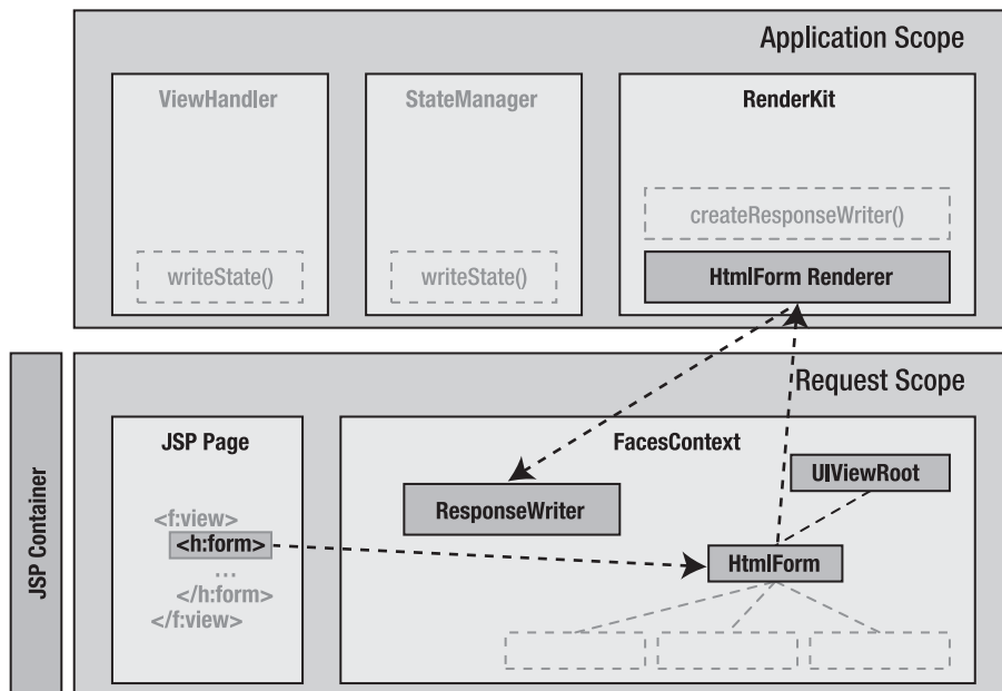
Figure 1-14. Writing <h:form> start element to the <f:view> body content buffer
