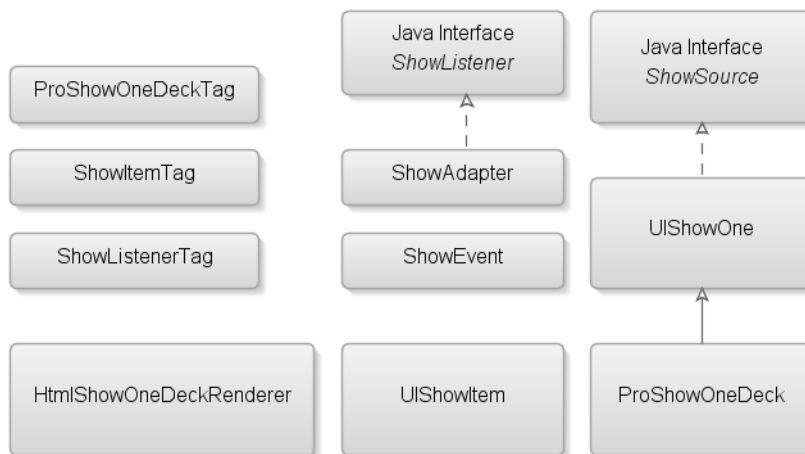
Figure 3-2. Class diagram showing classes created in this chapter
