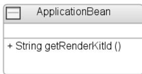
Figure 10-2. Class diagram showing the ApplicationBean class
