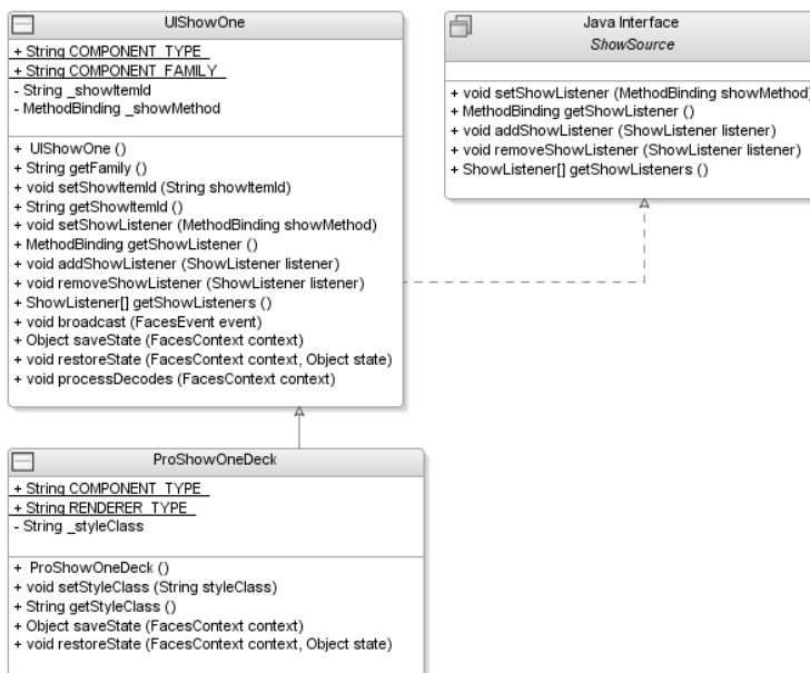
Figure 3-8. Class diagram showing the UIMShowOne implementation
