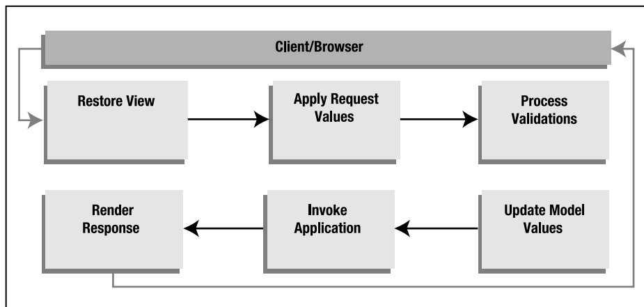
Figure 1-8. Formal lifecycle of JSF
