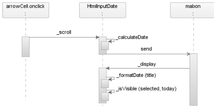
Figure 7-12. HtmlInputDate.prototype._scroll method
