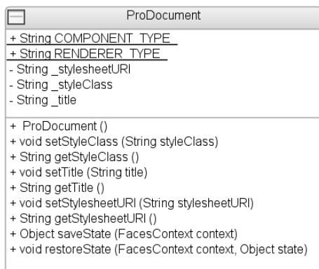
Figure 8-11. Class diagram showing the ProDocument class
