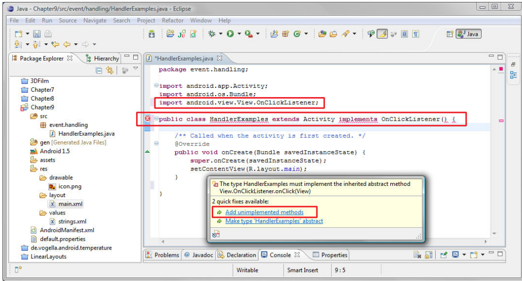
Figure 9–2. Editing HandlerExamples.java
