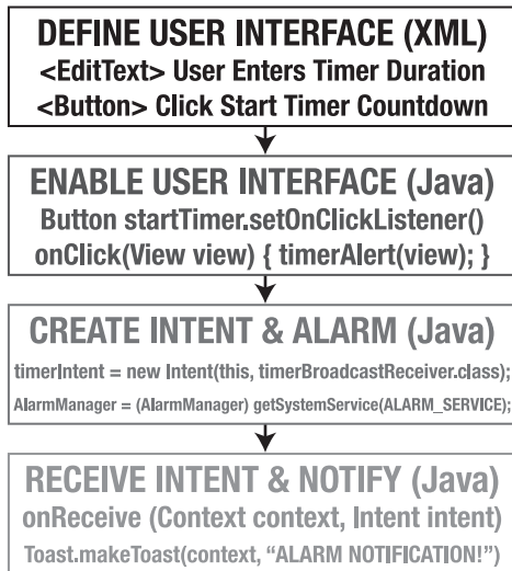
Figure 11–19. What we have to do in XML and Java to create the intent and alarm
