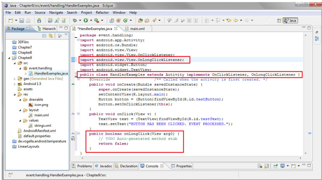
Figure 9–10. Implementing an OnLongClick listener in HandlerExamples.java
