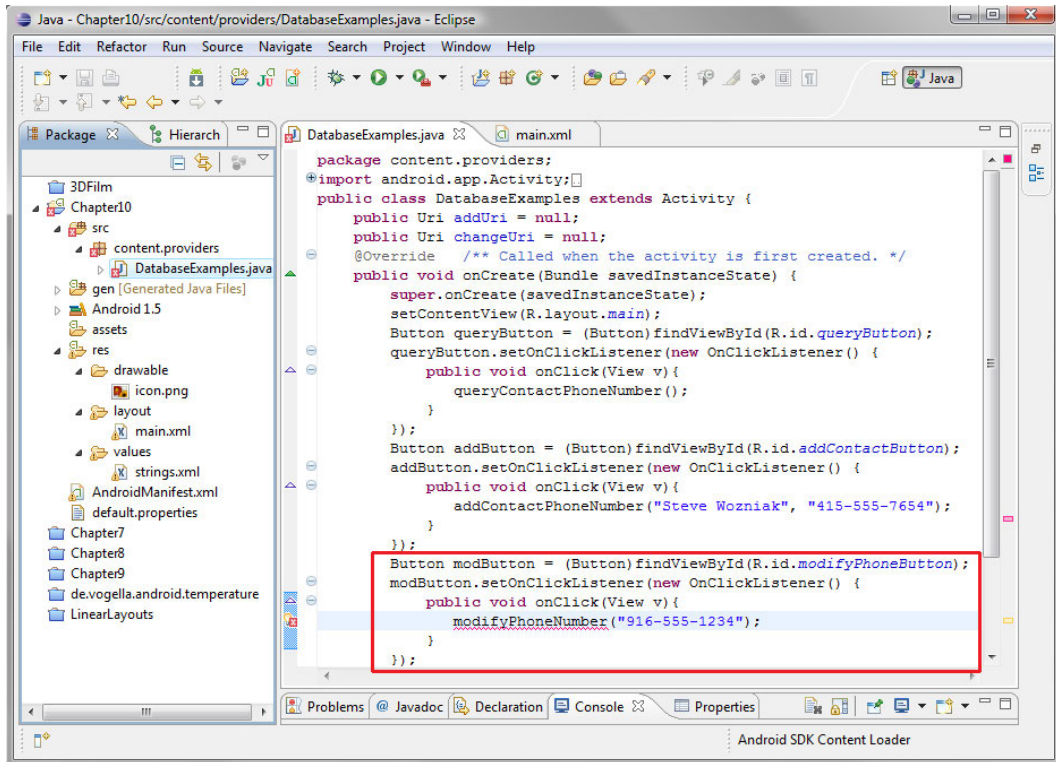
Figure 10-24. Adding the our Java code to implement the delete button
