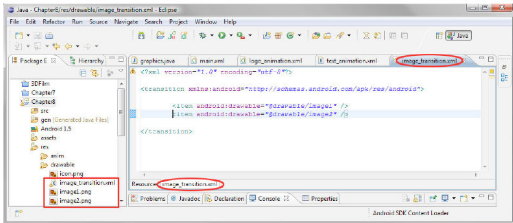
Figure 8–12. Writing our XML mark-up to transition between two images in our image_transition.xml file
