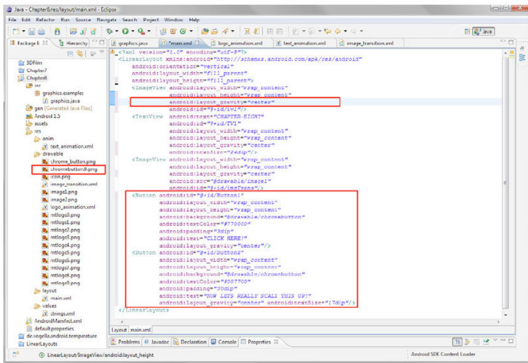
Figure 8-21. Adding our 9-patch PNG in our main.xml UI layout and setting layout_gravity to center buttons
