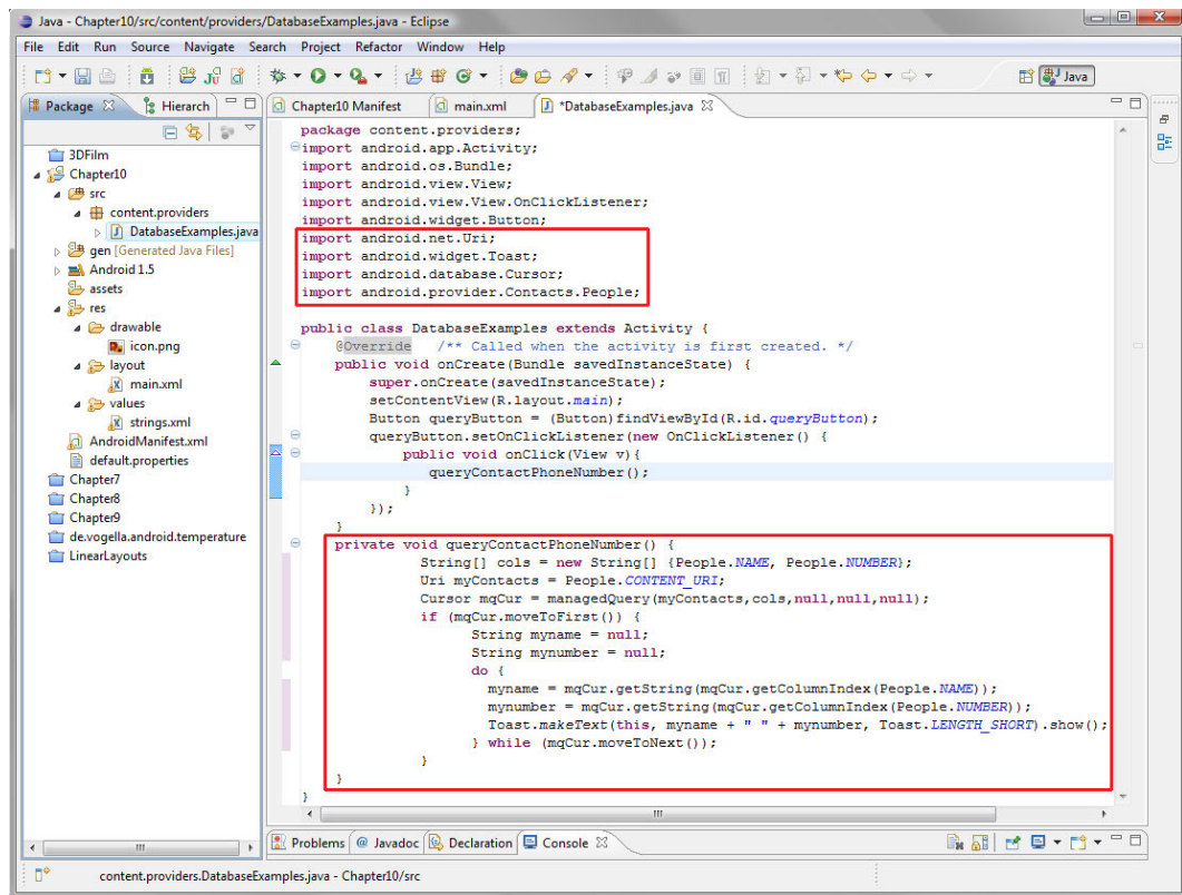
Figure 10–12. Java for our queryContactPhoneNumber() and import statements
