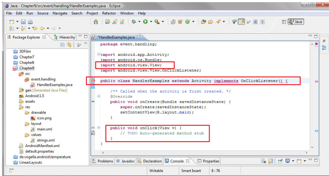
Figure 9–3. Implementing a listener in our class definition via the implements keyword
