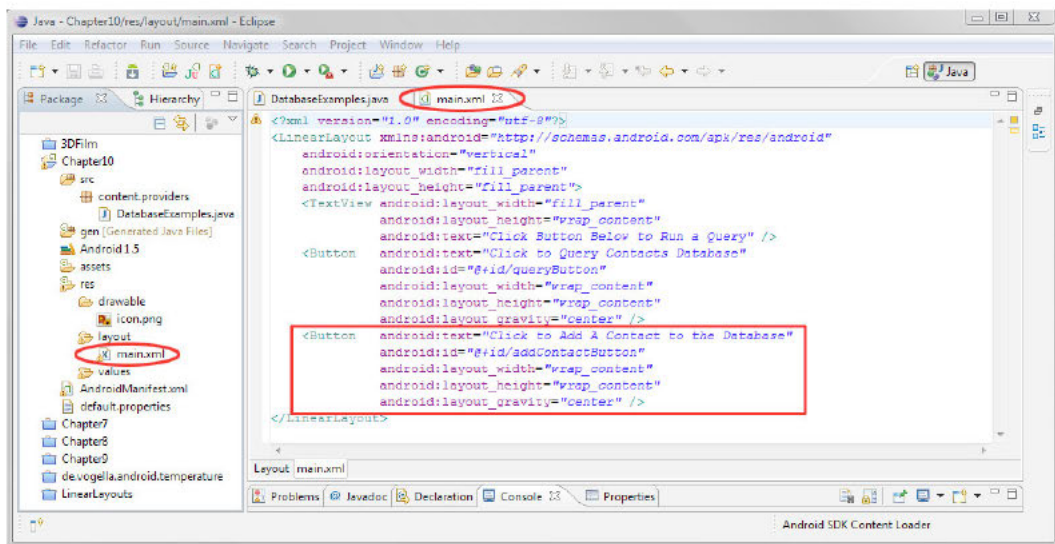
Figure 10-14. Adding our second button in main.xml
