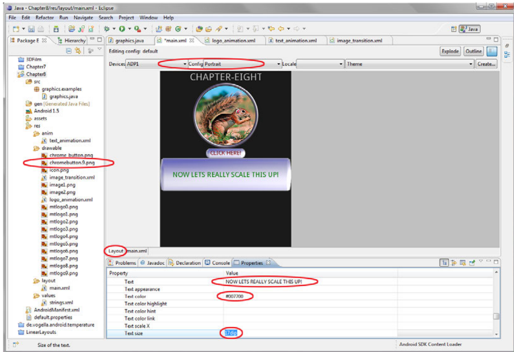
Figure 8–20. Setting UI parameters and portrait mode in the Eclipse layout editor
