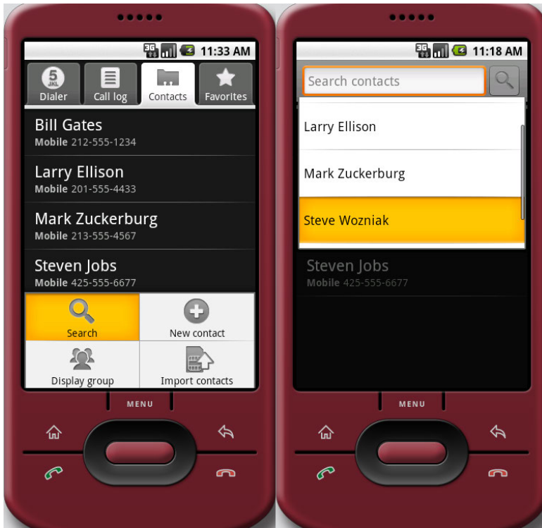
Figure 10-18. Using the Contacts editor utility in the Android 1.5 emulator
