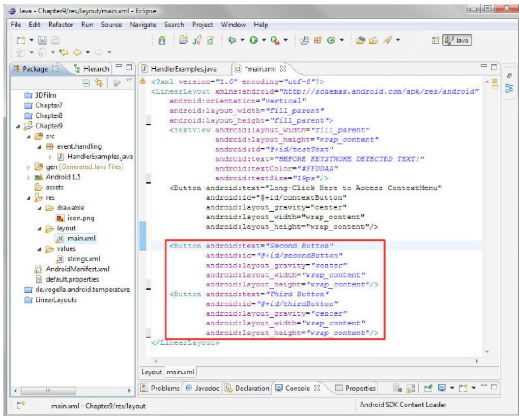
Figure 9–18. Adding UI buttons to the main.xml file
